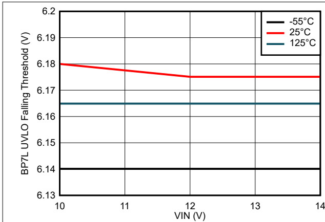
7-25. BP7L UVLO Falling Threshold vs VIN Voltage
