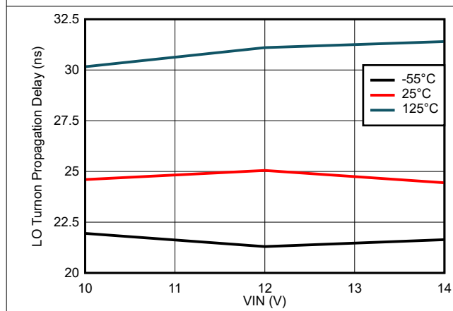
7-5. LO Turnon Propagation Delay vs VIN Voltage (IIM)
