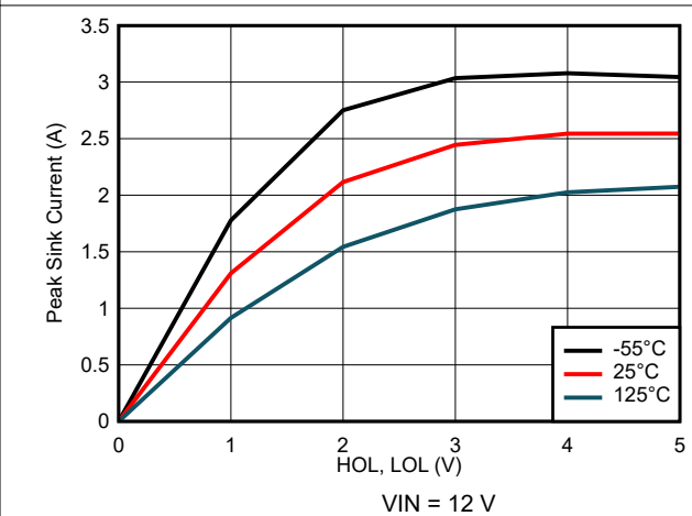
7-12. Peak Sink Current vs Output Voltage
