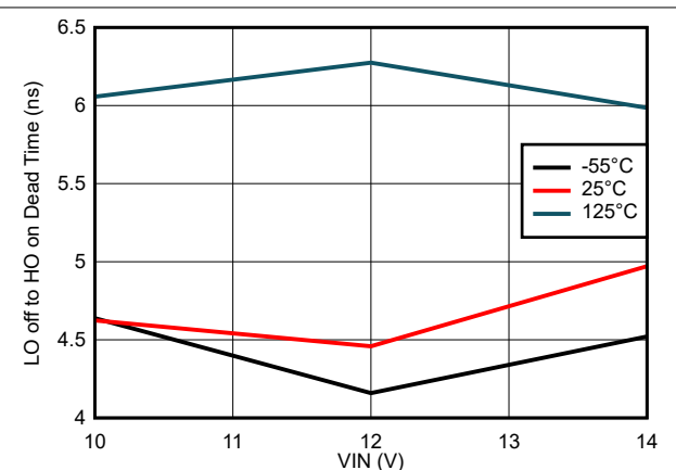
7-30. LO off to HO on Dead Time vs VIN Voltage RLH = 3.32 kΩ
