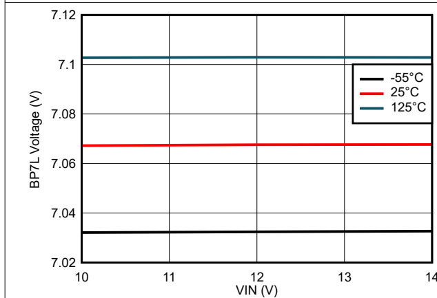
Figure 7-15. BP7L Output Voltage vs VIN Voltage
