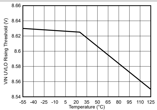
7-26. VIN UVLO Rising Threshold vs Temperature
