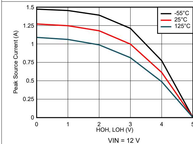
7-11. Peak Source Current vs Output Voltage
