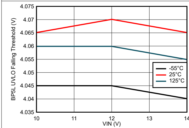
7-21. BP5L UVLO Falling Threshold vs VIN Voltage
