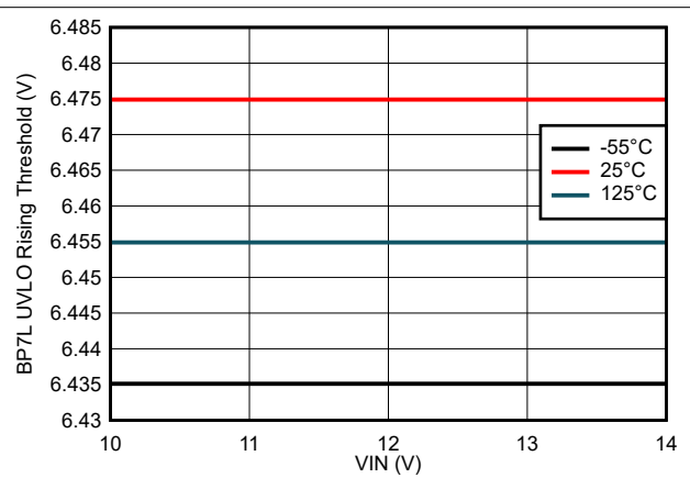
7-24. BP7L UVLO Rising Threshold vs VIN Voltage
