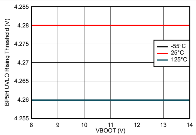
7-22. BP5H UVLO Rising Threshold vs BOOT Voltage
