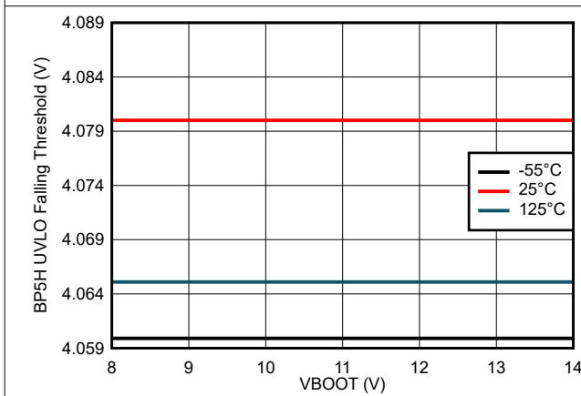
7-23. BP5H UVLO Falling Threshold vs BOOT Voltage
