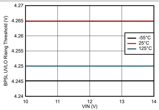
7-20. BP5L UVLO Rising Threshold vs VIN Voltage
