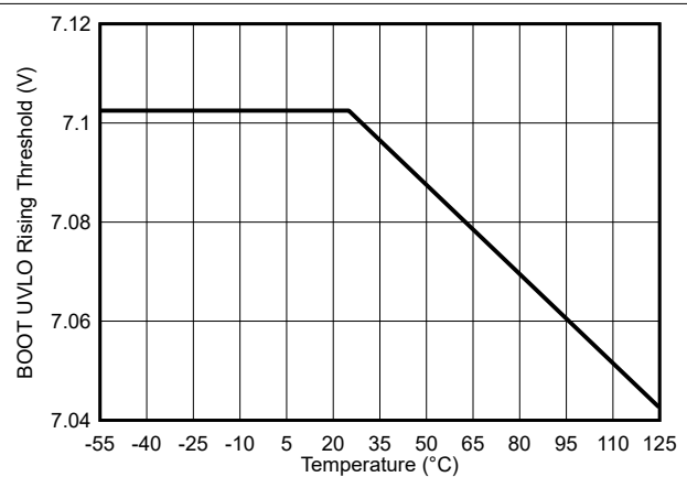
7-28. BOOT UVLO Rising Threshold vs Temperature
