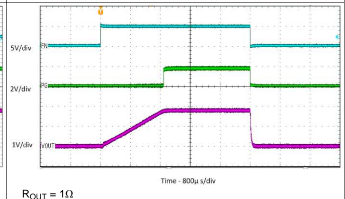
图 29. Startup / Shutdown with Resistance Load
