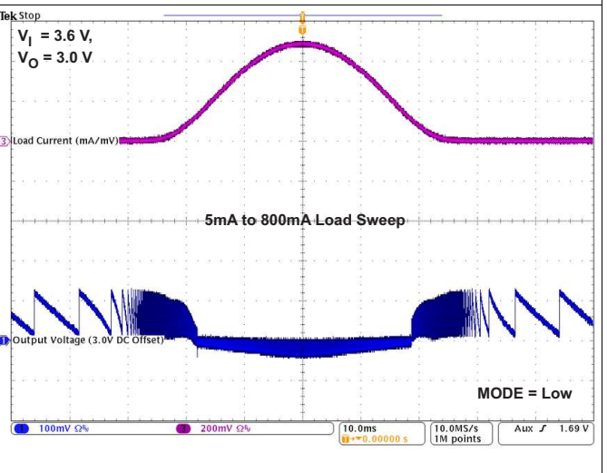
Figure 41. TPS82698 AC Load Transient Response
