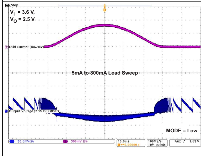
Figure 40. TPS826951 AC Load Transient Response
