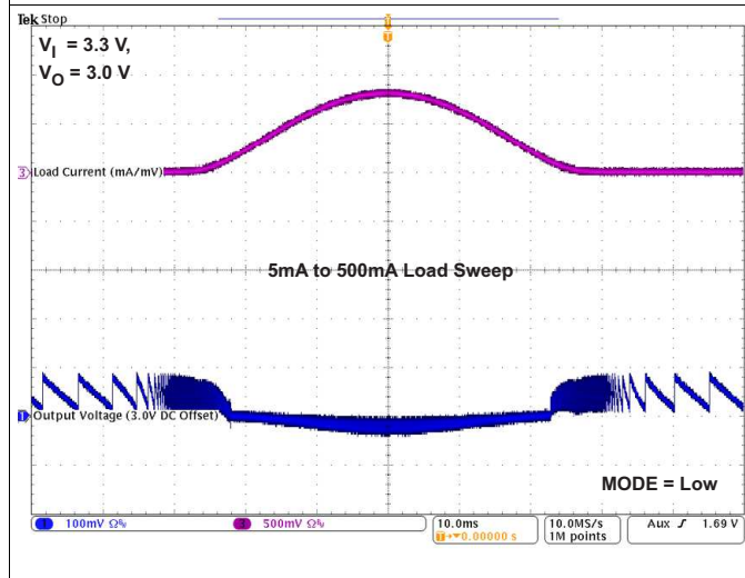
Figure 42. TPS82698 AC Load Transient Response
