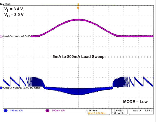
Figure 43. TPS82698 AC Load Transient Response
