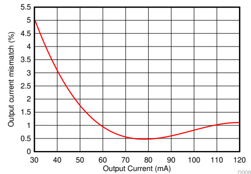
7-4. LED Current Sink Matching
