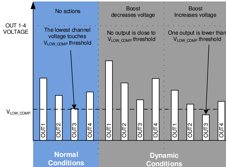
8-2. Adaptive Boost Voltage Control Loop Function
