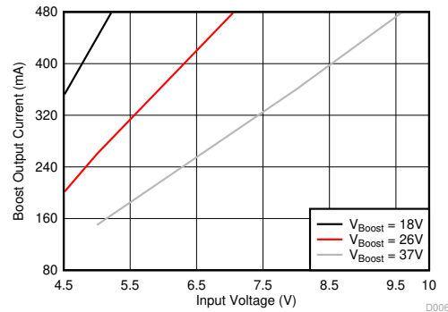
7-2. Maximum Boost Current
