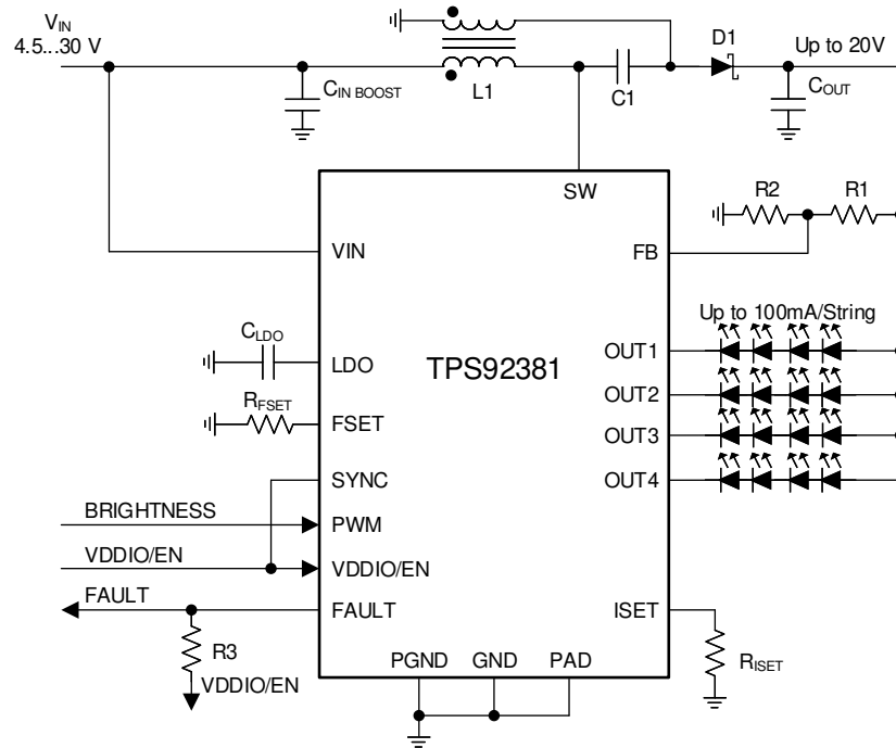
9-4. SEPIC Mode, 4 Strings 100 mA per String Configuration
