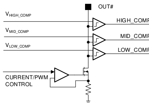
8-6. Comparators for LED Fault Detection
