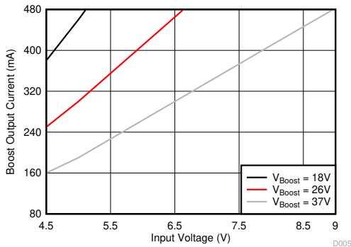
7-1. Maximum Boost Current
