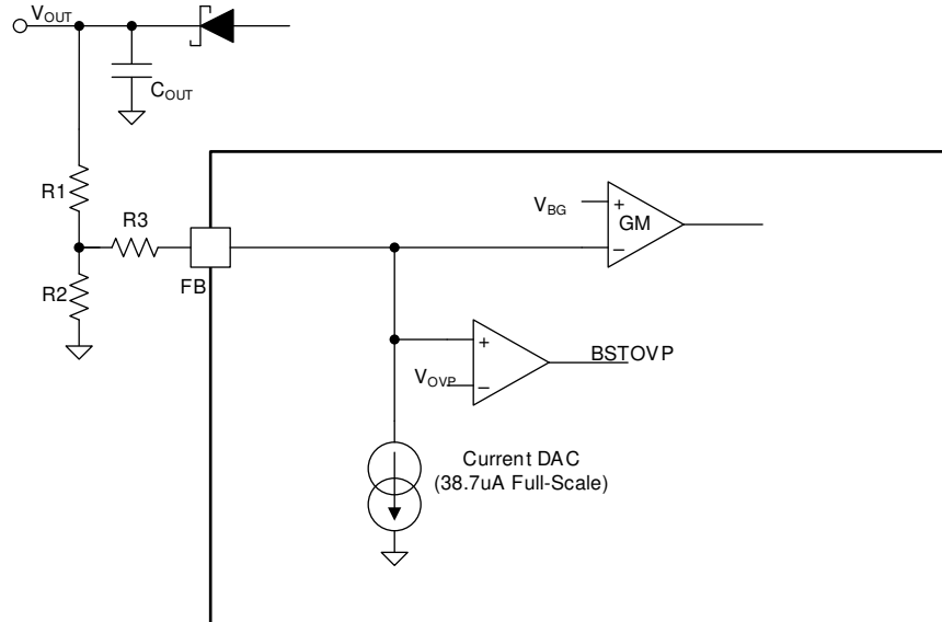
8-4. FB External T-divider Resistors
