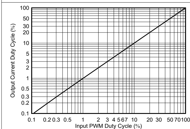
Figure 6-5. PWM Output Duty Cycle vs PWM Input Duty Cycle
