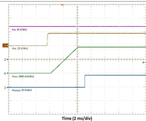
8-3. Start-Up Waveforms
