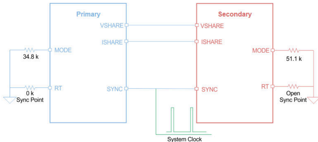
7-5. 2-Phase Stackable, 180° Phase Shift: Primary and Secondary Sync to External System Clock
