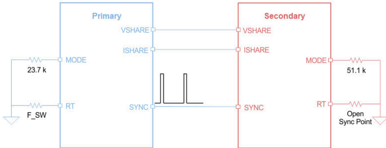
7-4. 2-Phase Stackable, 180° Phase Shift: Primary Sync-Out Clock to Secondary
