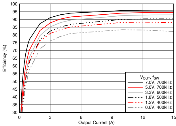
6-1. Efficiency vs Output Current
