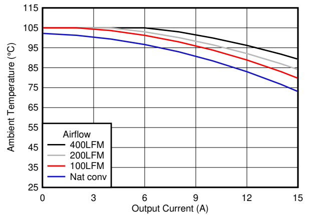
6-4. Safe Operating Area
