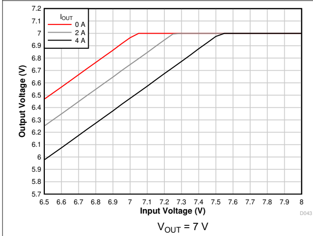
7-11. Voltage Dropout
