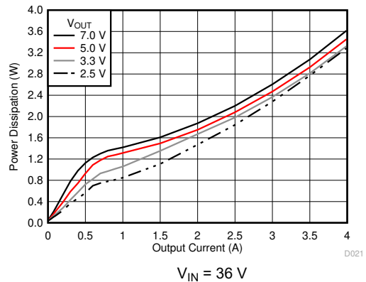
6-21. Power Dissipation versus Output Current
