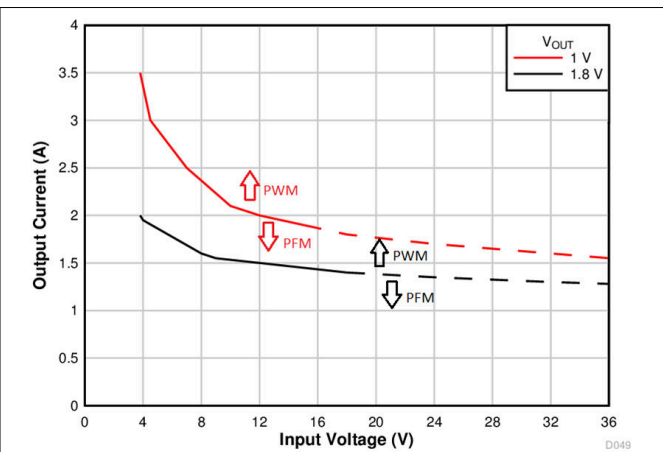
Figure 7-15. PFM/PWM Thresholds (1 V and 1.8 V)
