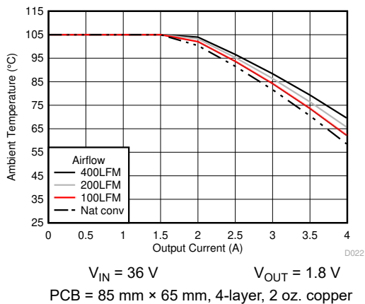
6-23. Safe Operating Area
