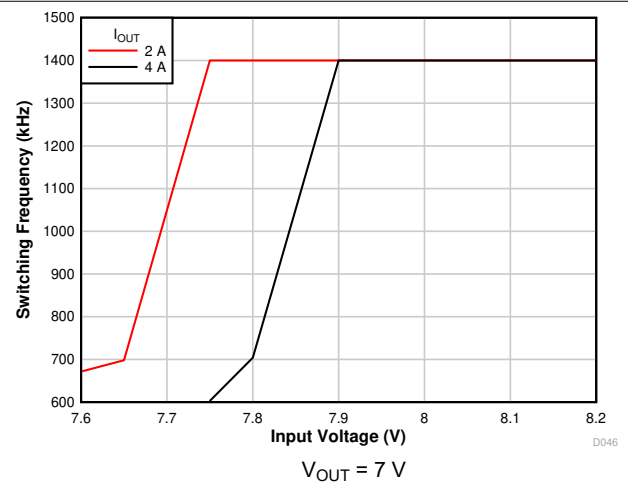
7-12. Frequency Foldback
