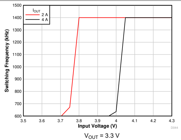
7-8. Frequency Foldback
