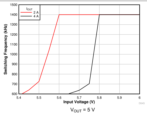
7-10. Frequency Foldback
