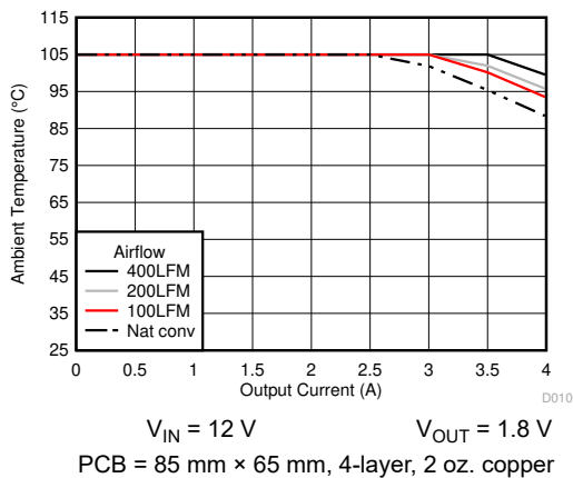
6-11. Safe Operating Area
