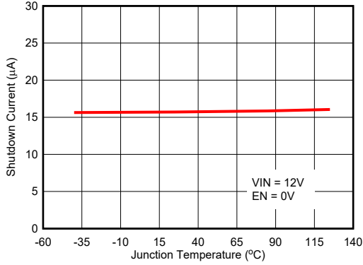
☒ 5-13. Shutdown Current
