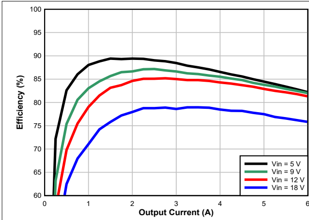
7-4. Efficiency
