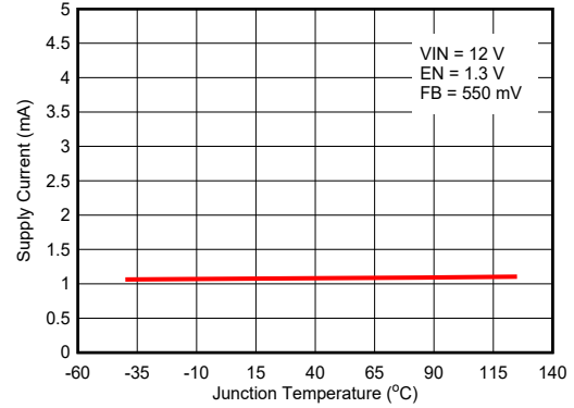
☒ 5-14. Non-Switching Supply Current
