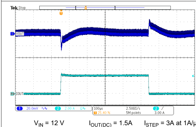
7-8. Load Transient
