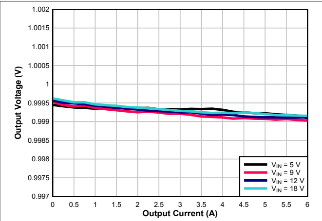
7-5. Load Regulation
