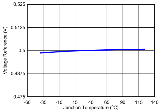
5-7. Voltage Reference
