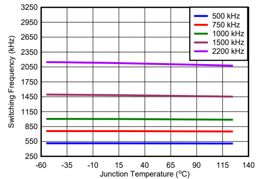
5-12. Switching Frequency
