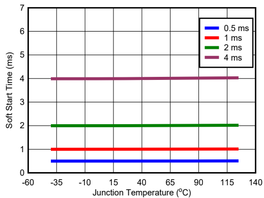
5-11. Soft Start
