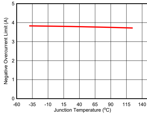
図 5-15. Negative Overcurrent
