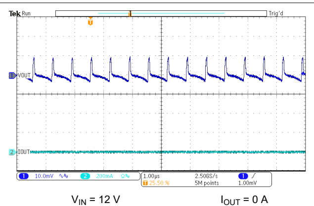
7-15. Output Ripple – No Load
