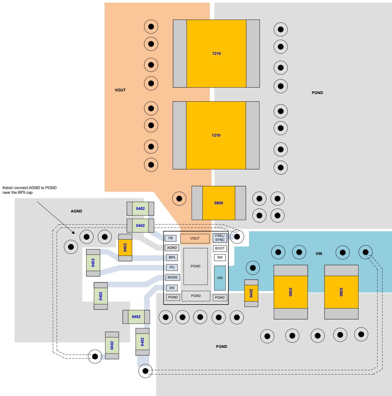
7-19. Example PCB Layout
