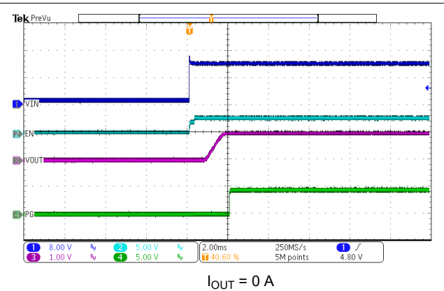
7-13. VIN Start-Up
