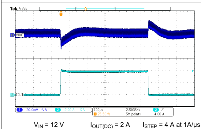
7-8. Load Transient
