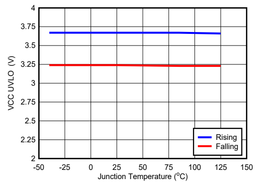
Figure 6-8. VCC UVLO
