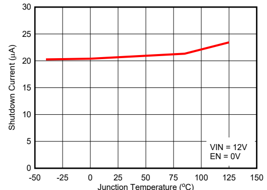
Figure 6-14. Shutdown Supply Current
