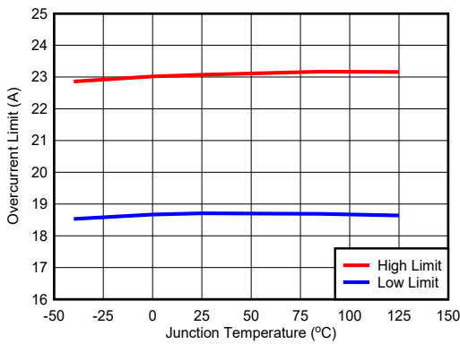
6-3. Overcurrent Limit
