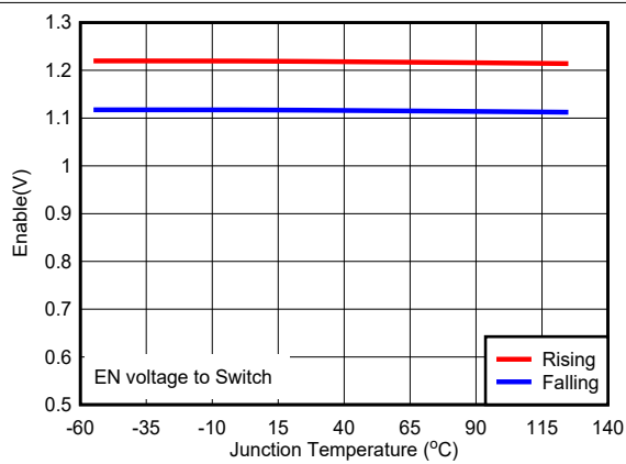
Figure 6-5. Enable Voltage
