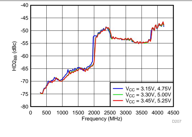
Figure 63. BB-HD2 vs Supply, Typical Operating Mode
