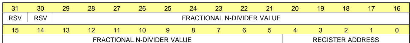
Figure 70. PLL 4WI Register 3
