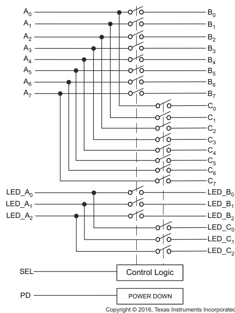
8-1. Logic Diagram (Positive Logic)
