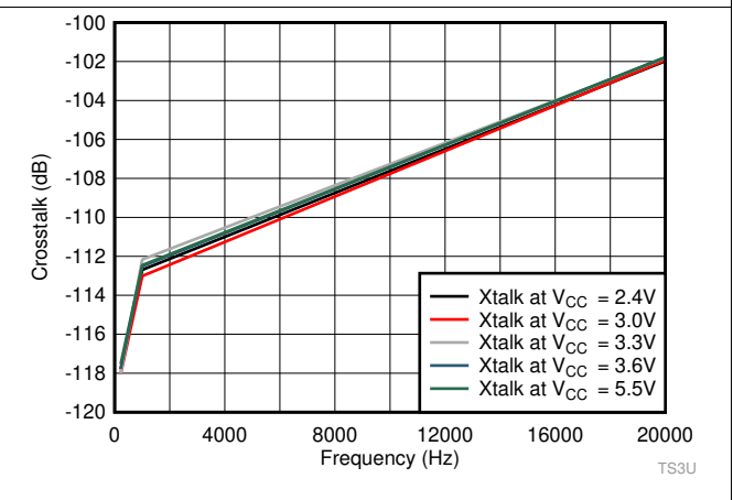
Figure 6. Crosstalk
