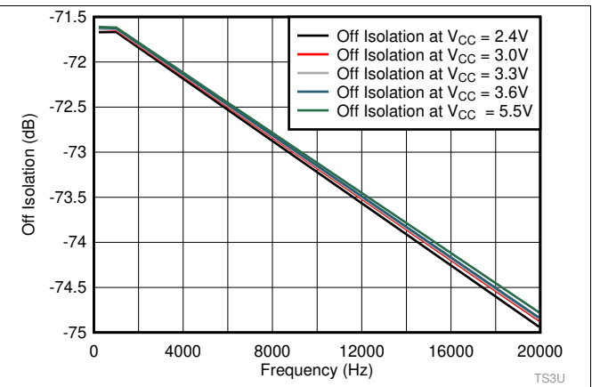
Figure 4. Off Isolation
