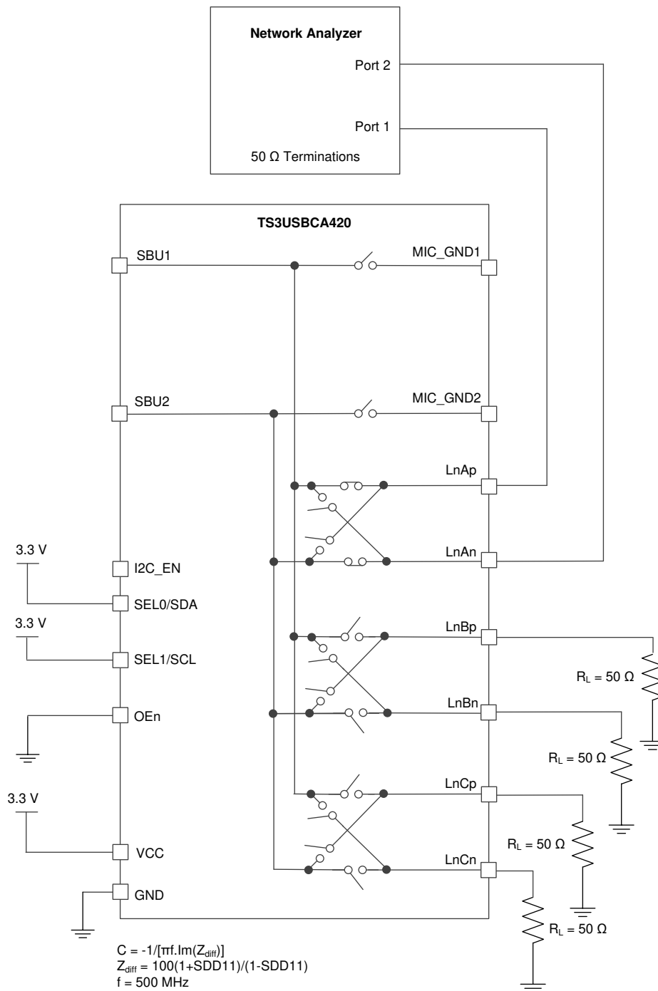
图 9. ON-State and OFF-State Output Capacitance for High-Speed Data Paths ( C_{\text{ON\_HS}} , C_{\text{OFF\_HS}} )
