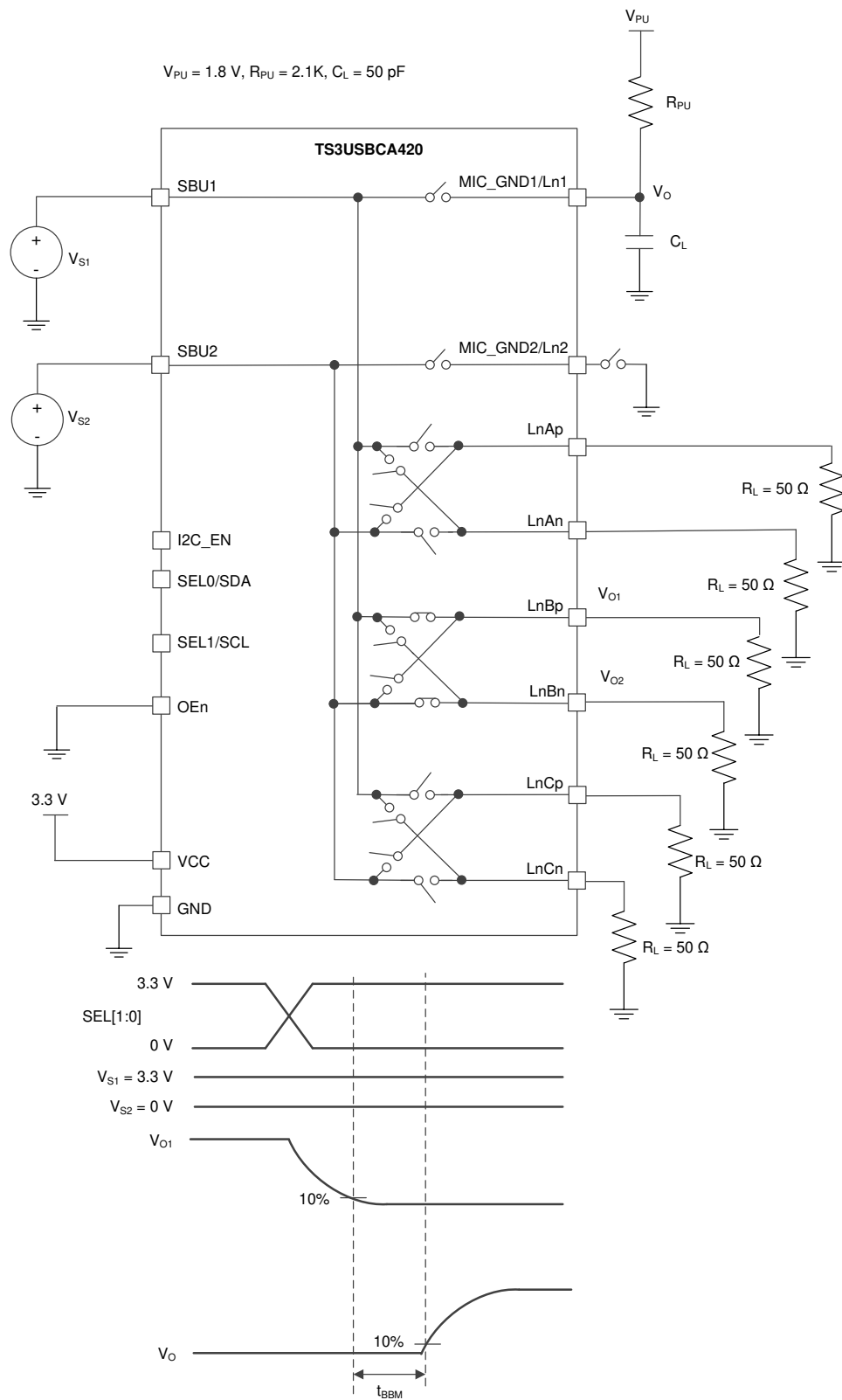
16. Break-Before-Make Time (t BBM )
