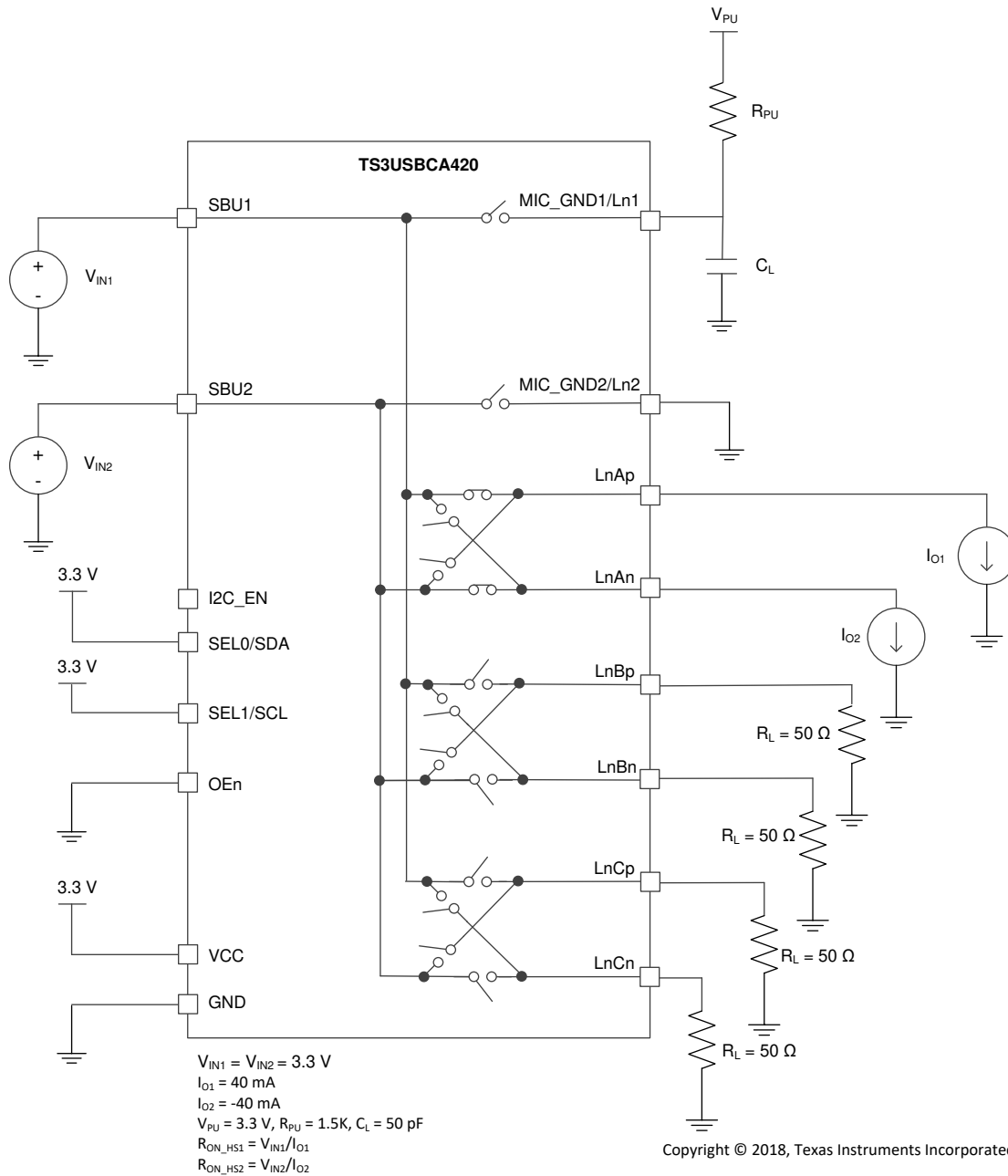
8. ON-State Resistance for High-Speed Data Paths ( R_{ON\_HS} )
