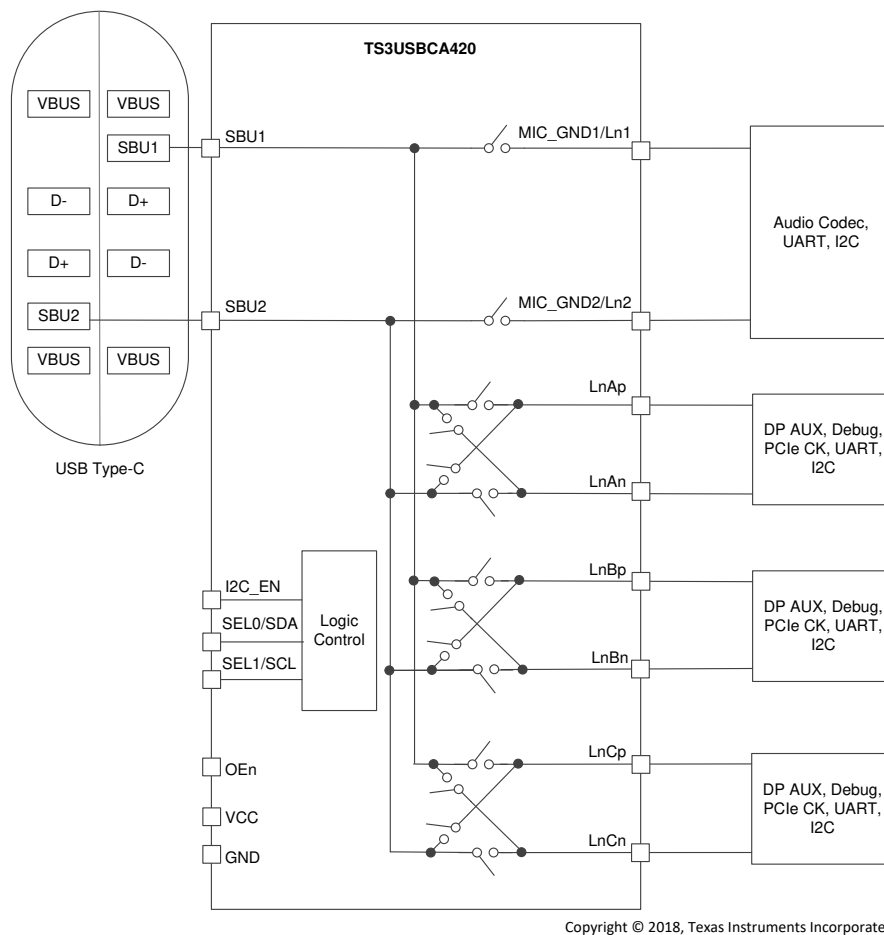
✎ 17. Functional Block Diagram
