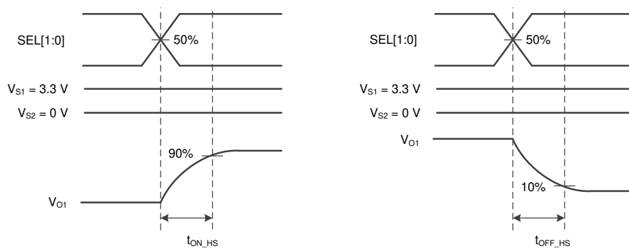
15. Turn-ON time ( t_{ON} ) and Turn-OFF time ( t_{OFF} ) for High-Speed Data Paths
