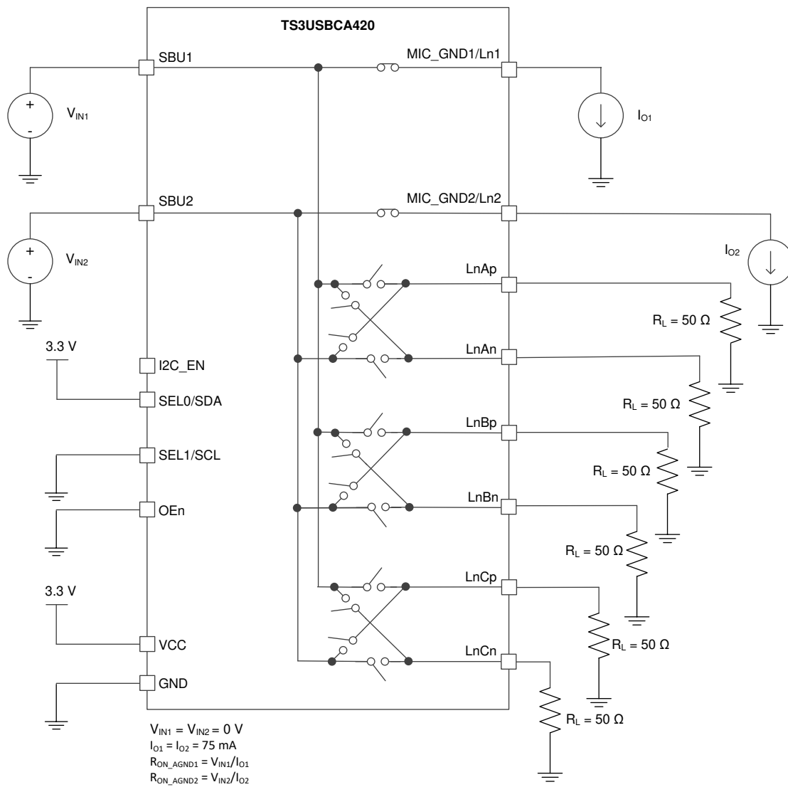
7. ON-State Resistance for the Analog Audio GND ( R_{ON\_AGND} )
