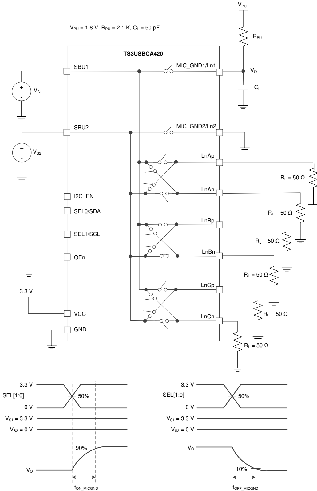
14. Turn-ON time ( t_{ON} ) and Turn-OFF time ( t_{OFF} ) for MIC and AGND
