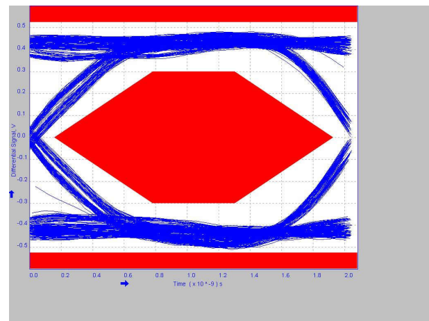
9-4. 2 Meter Pre-Channel With TUSB217A BOOST=1 RX_SEN=MED
