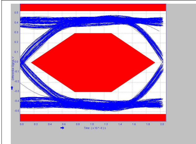
9-5. 2 Meter Pre-Channel With TUSB217A BOOST=0 RX_SEN=HIGH
