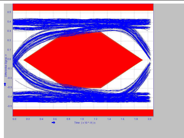
9-6. 3 Meter Pre-Channel Without TUSB217A
