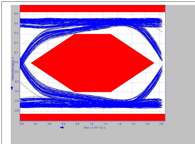
9-3. 2 Meter Pre-Channel Without TUSB217A
