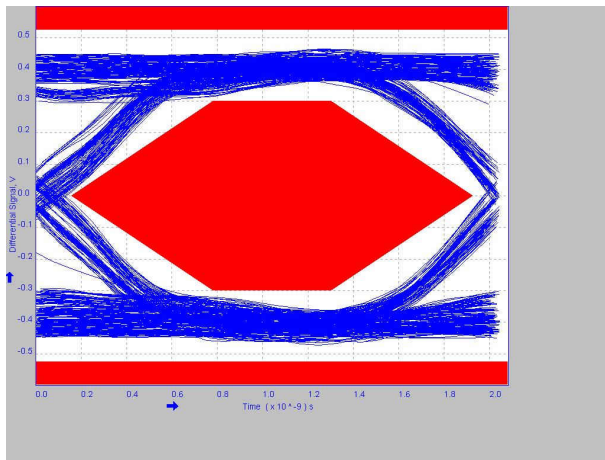
9-9. 5 Meter Pre-Channel With TUSB217A BOOST=1 RX_SEN=MED
