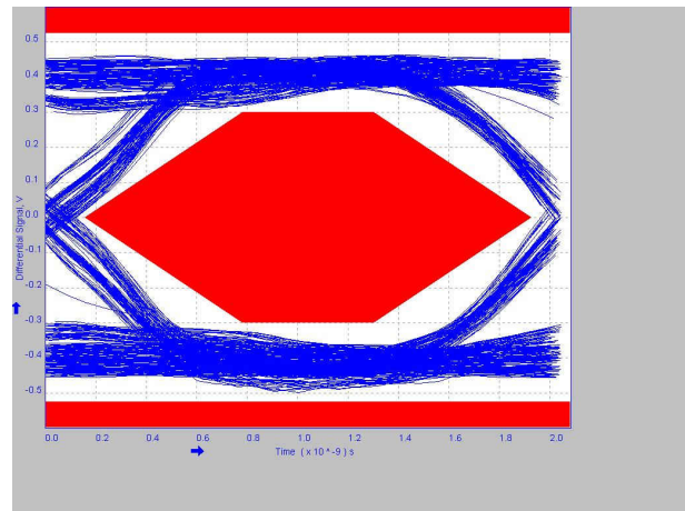
9-10. 5 Meter Pre-Channel With TUSB217A BOOST=2 RX_SEN=MED
