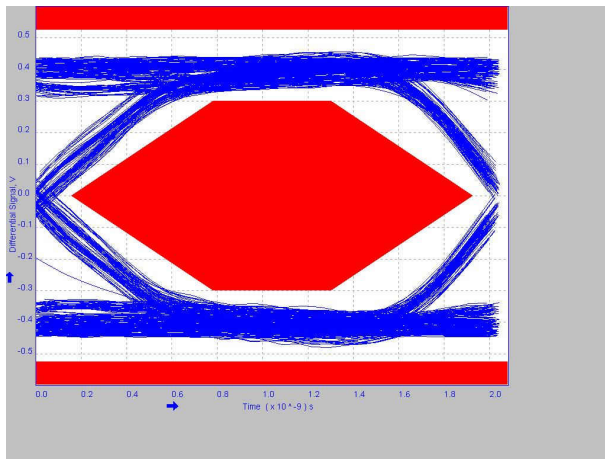
9-7. 3 Meter Pre-Channel With TUSB217A BOOST=0 RX_SEN=HIGH
