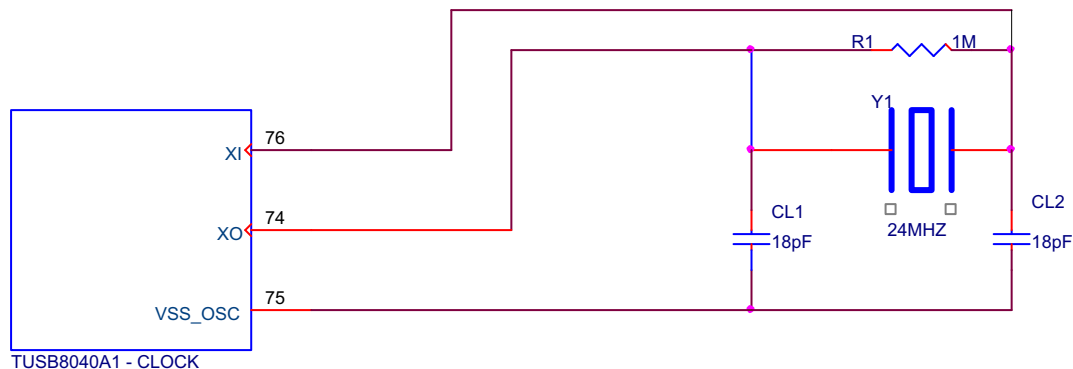
FIG 6-1. TUSB8040A1 Clock
