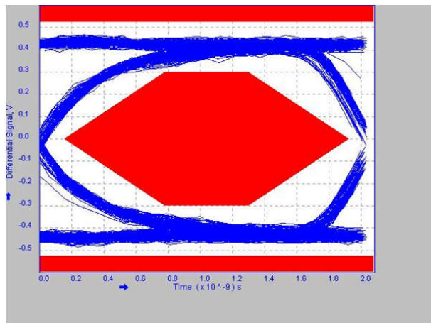
8-15. High-Speed Upstream Port
