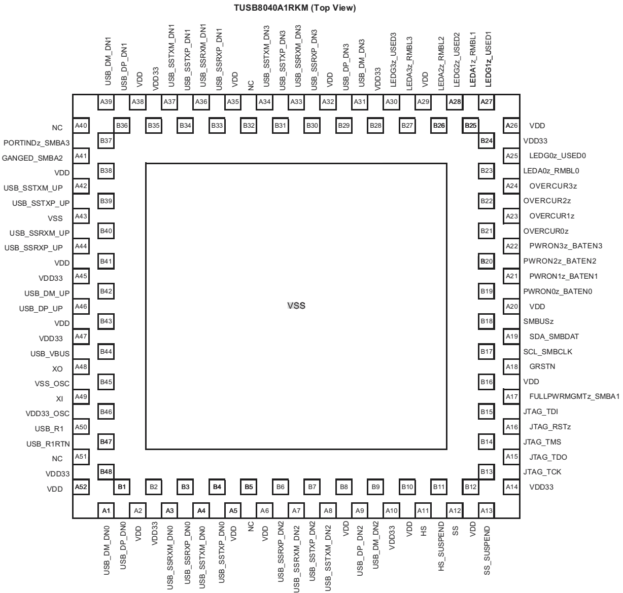
5-1. 100-Pin TUSB8040A1 RKM Package, 100-Pin WQFN (Top View)
