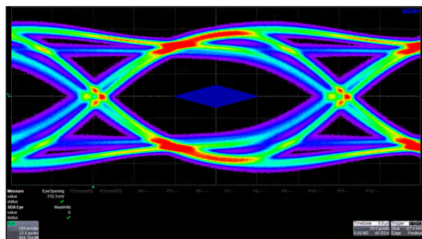
8-13. Downstream Port 3
