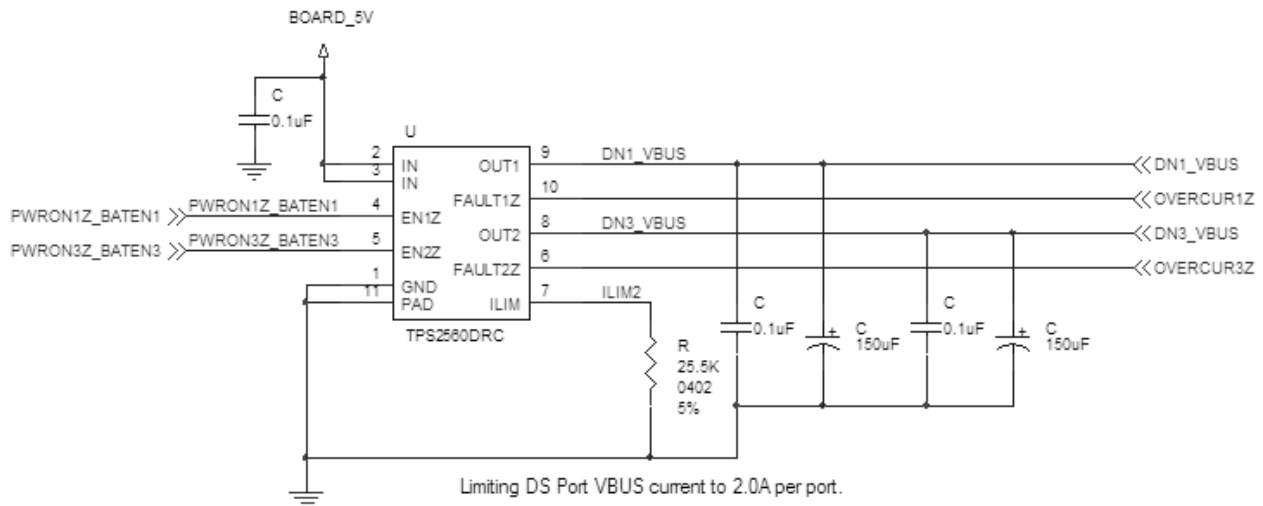
8-7. VBUS Power Switch Implementation
