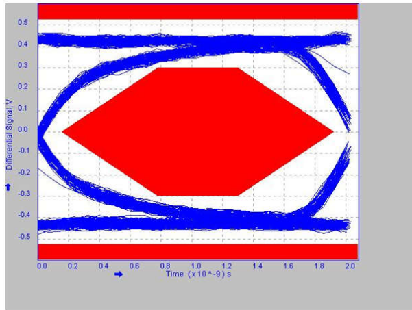
8-16. High-Speed Downstream Port 1
