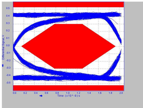
8-18. High-Speed Downstream Port 3
