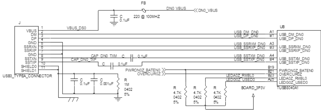
8-3. Downstream Port 1 Implementation
