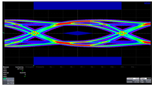
8-11. Downstream Port 1
