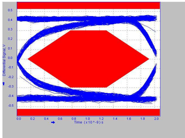
8-19. High-Speed Downstream Port 4
