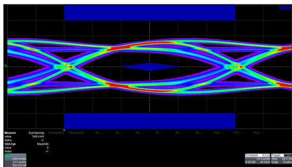
8-14. Downstream Port 4
