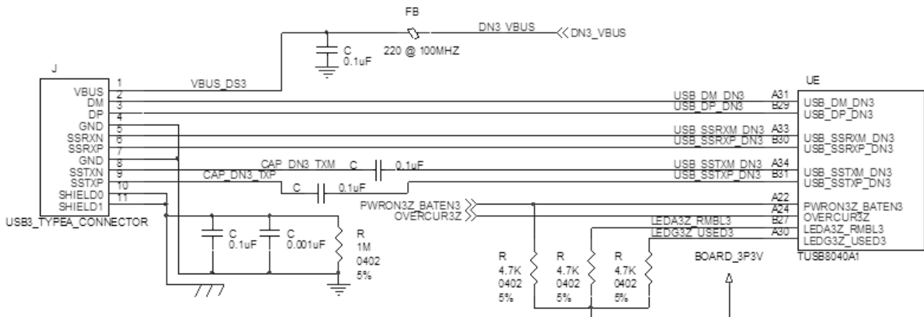
FIG 8-6. Downstream Port 4 Implementation
