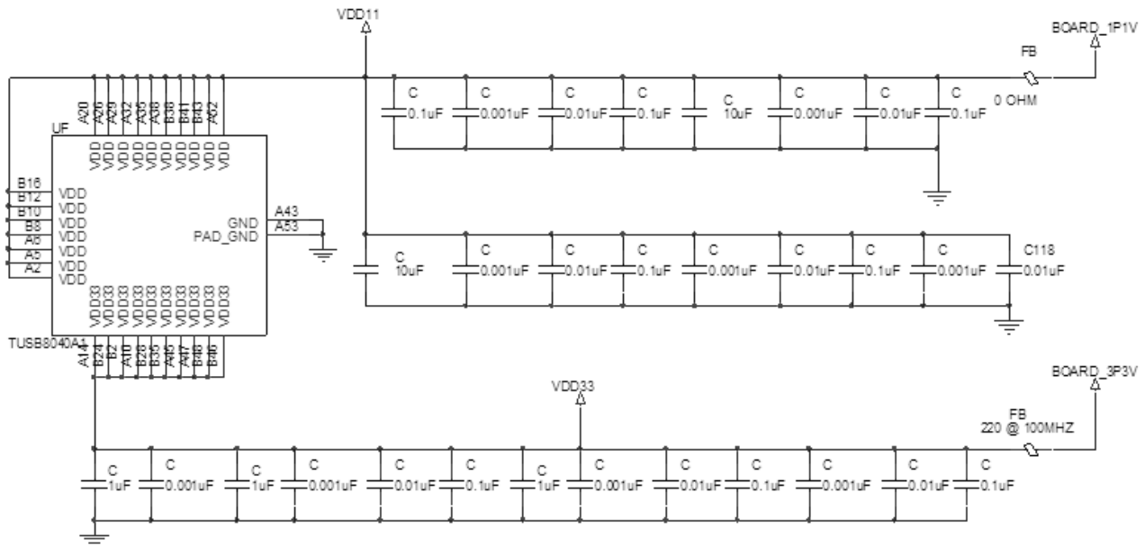
FIG 8-9. Power Implementation
