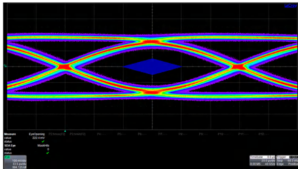
8-10. Upstream Port
