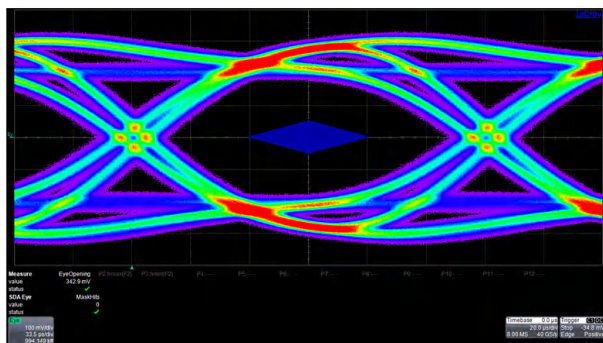
8-12. Downstream Port 2
