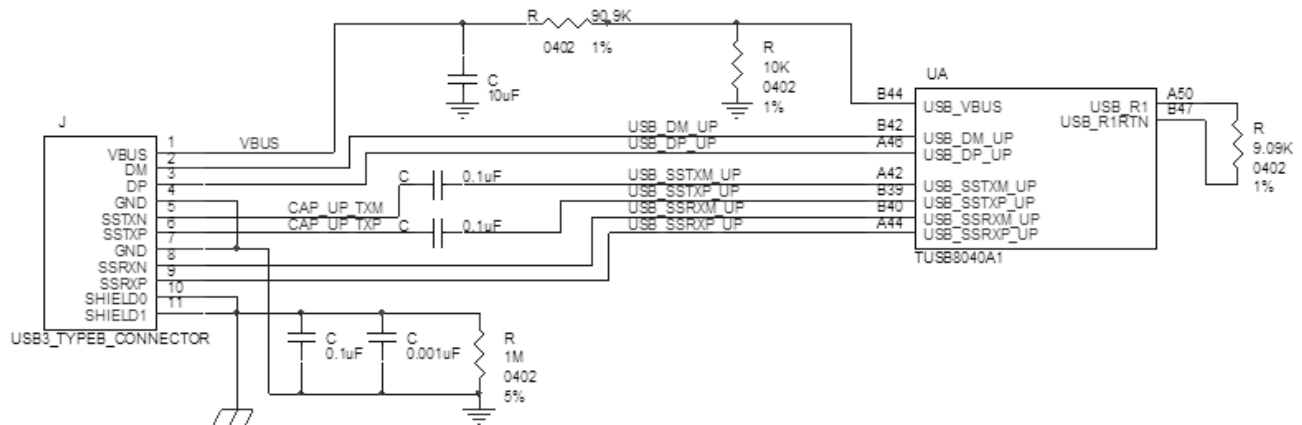
図 8-2. Upstream Port Implementation
