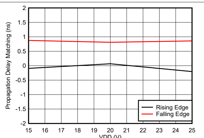
图 5-15. Propagation Delay Matching (t DM ) vs VDD
