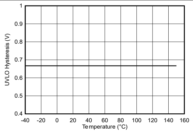
5-19. VDD 8-V UVLO Hysteresis vs Temperature
