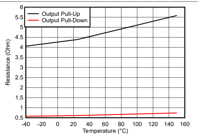
图 5-11. Output Resistance vs Temperature
