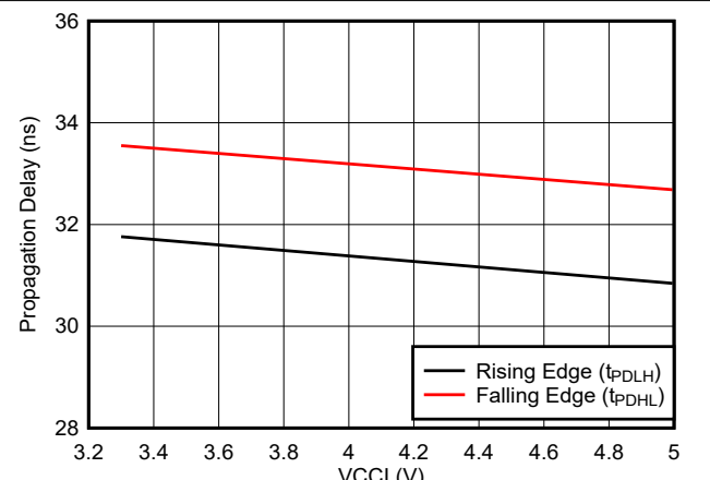
图 5-13. Propagation Delay vs VCCI
