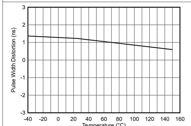
图 5-14. Pulse Width Distortion vs Temperature
