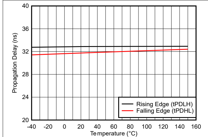
图 5-12. Propagation Delay vs Temperature
