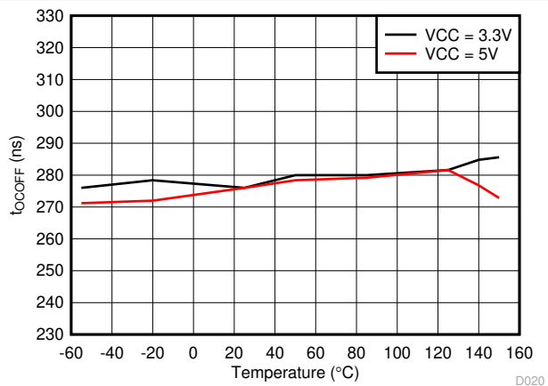
图 5-24. t_{COFF} OC Propagation Delay vs. Temperature
