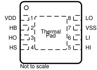
5-2. DRM Package 8-Pin SON Top View
