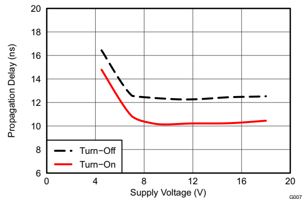
図 5-16. Propagation Delays vs Supply Voltage
