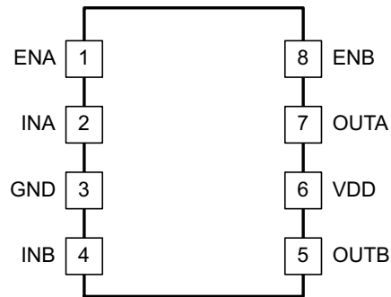
図 5-1. D and DGN Packages 8-Pin SOIC and HVSSOP Top View
