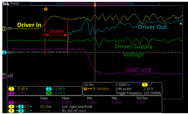
図 8-4. Turn-On Propagation Delay Waveform
