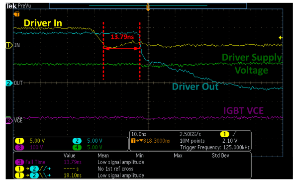
8-5. Turn-Off Propagation Delay Waveform
