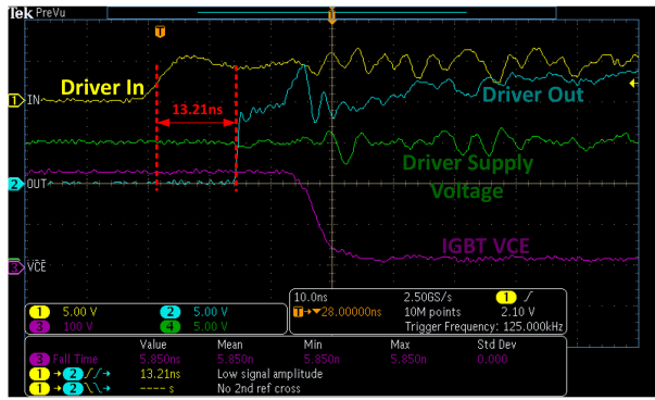
8-4. Turn-On Propagation Delay Waveform
