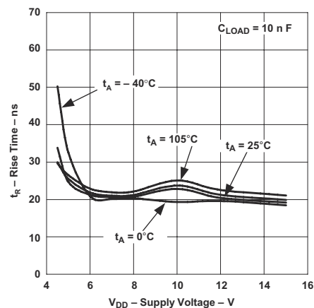
7-7. Rise Time vs Supply Voltage
