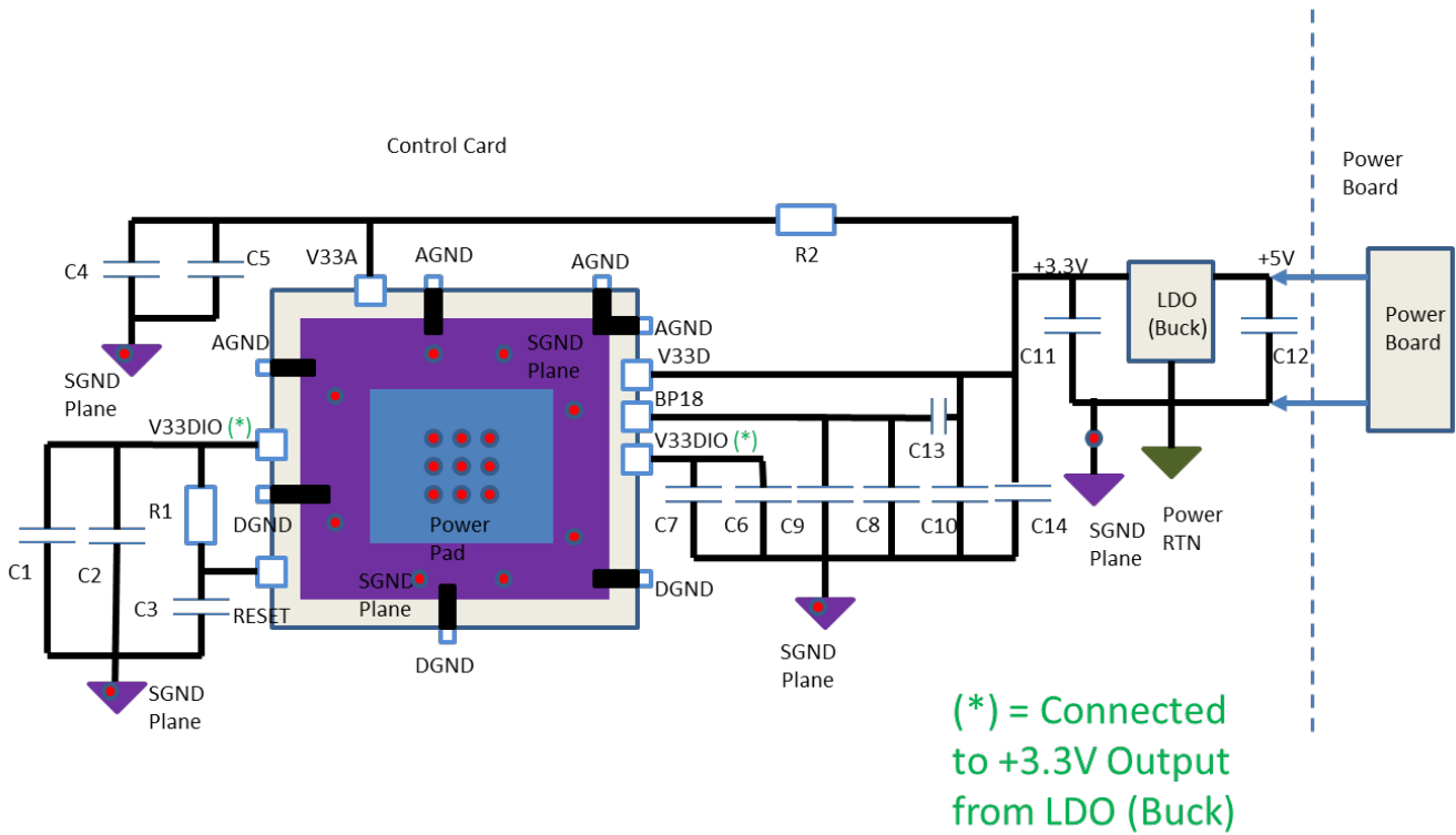
☒ 12-13. Power and Ground Schematic for UCD3138 and UCD3138064 64 Pin
