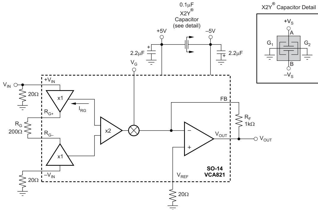
Figure 79. DC-Coupled, A_{V_{MAX}} = 20\text{ dB} , Bipolar Supply Specification and Test Circuit
