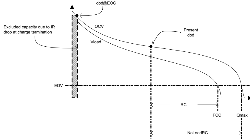
Figure 16-1. No Load
