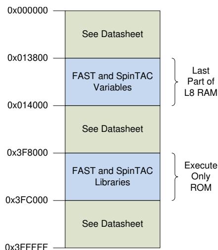
Figure 6-2. F2806xF and F2806xM Allocated Memory for InstaSPIN-FOC and SpinTAC Library
