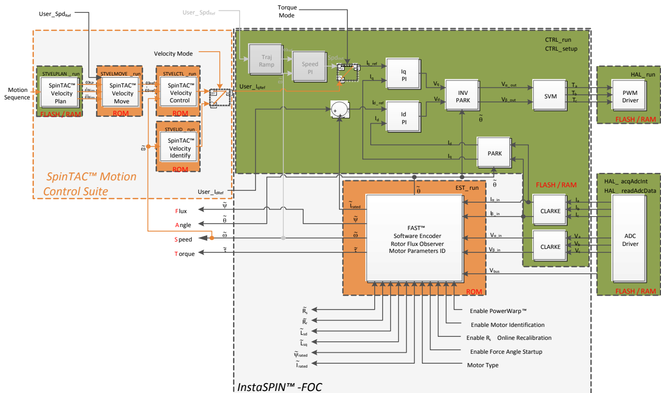
Figure 1-1. InstaSPIN-MOTION = C2000 F2806xM MCU + FAST Software Sensor (optional) + Auto-Tuned Inner-Torque Controller + SpinTAC Motion Control Suite
