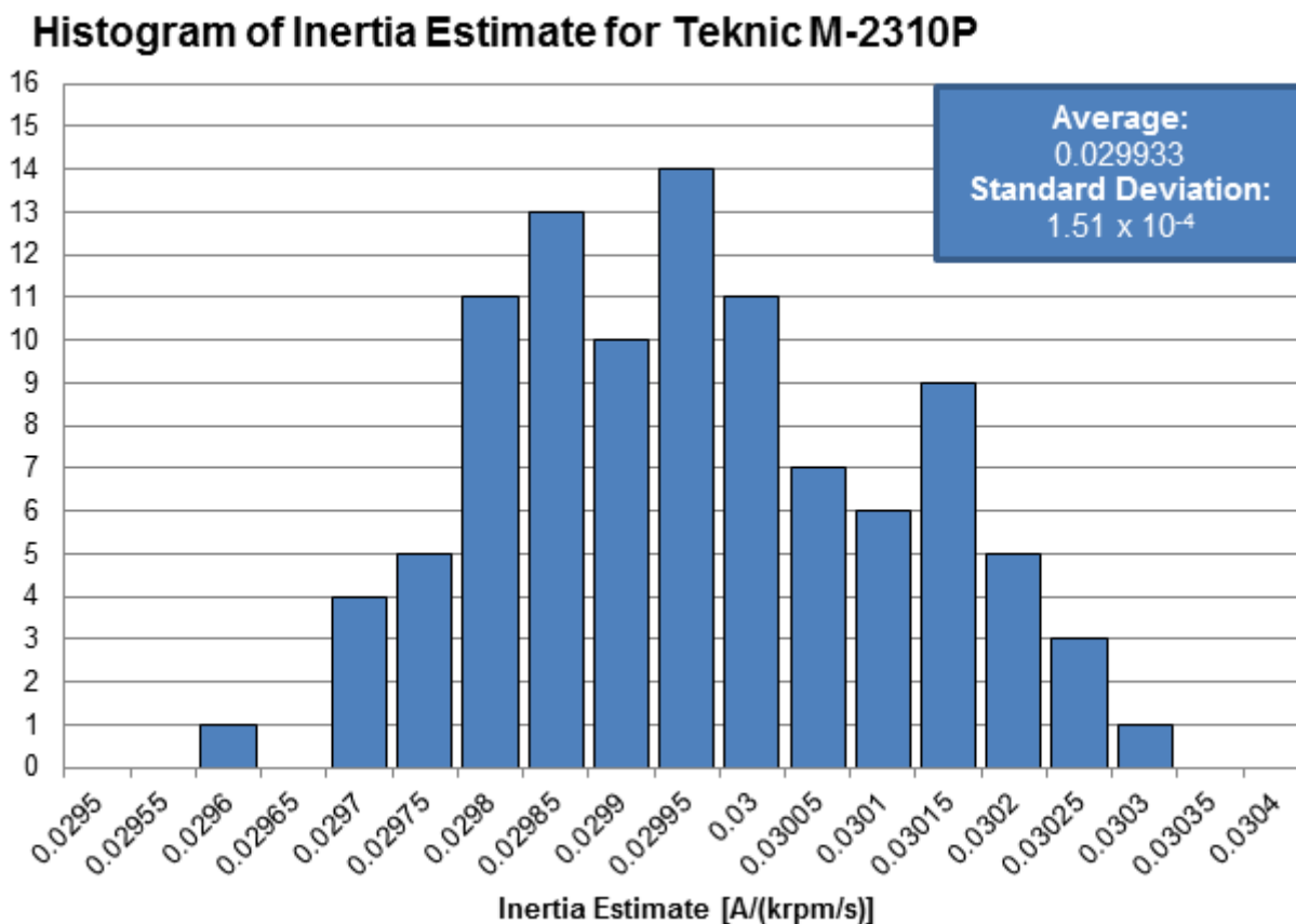
Figure 5-14. Inertia Estimation Results for Teknic M-2310P
