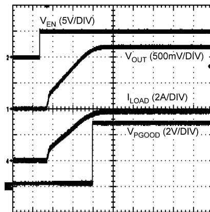
Startup Waveform(2ms/DIV)
