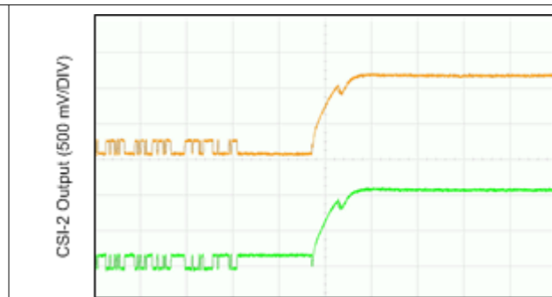
4-12. CSI-2 End of Transmission (EoT)
