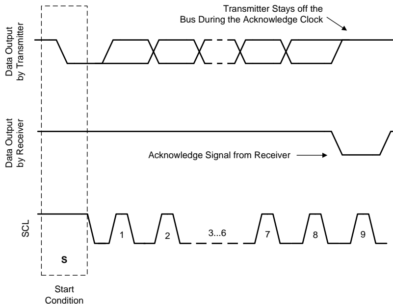
43. Acknowledge Signal
