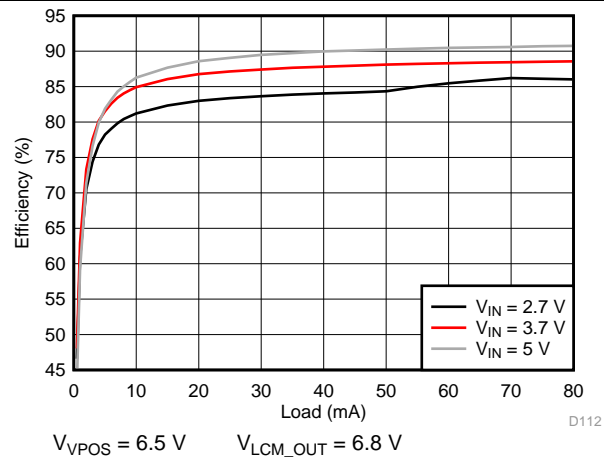
198. VPOS Efficiency
