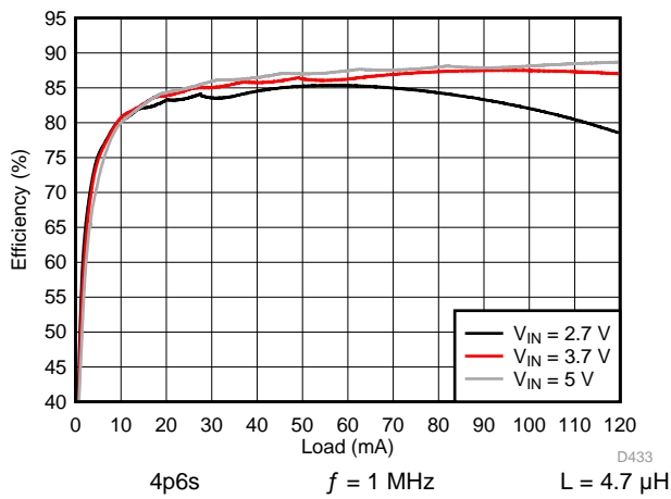
181. Backlight Boost Efficiency
