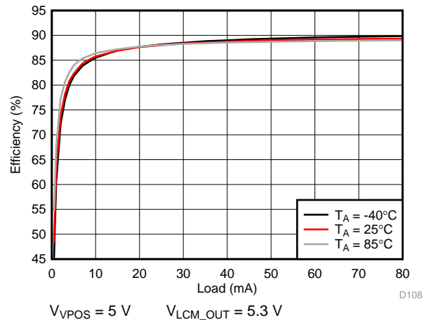
194. VPOS Efficiency
