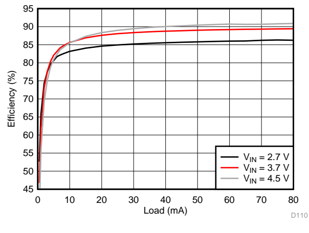
196. VPOS Efficiency
