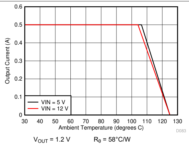
7-16. Ambient Temperature vs Output Current
