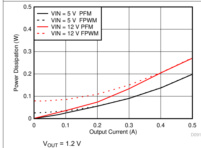
7-15. Power Dissipation
