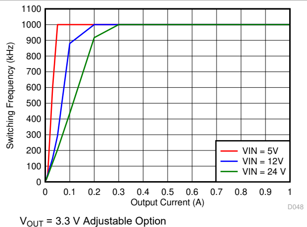
7-24. Auto PFM Mode Switching Frequency vs Output Current
