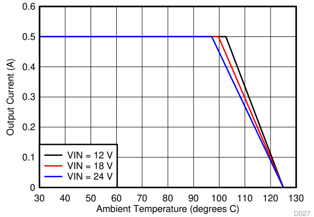
7-20. Ambient Temperature vs Output Current
