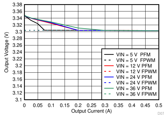
9-45. Line and Load Regulation for V_{OUT} = 3.3\text{ V}
