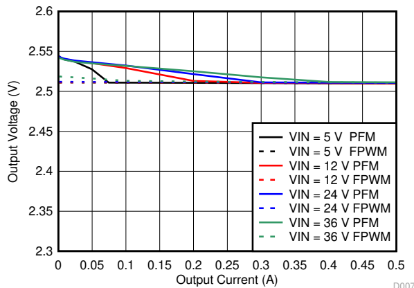
9-34. Line and Load Regulation
