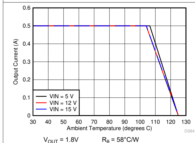
7-17. Ambient Temperature vs Output Current
