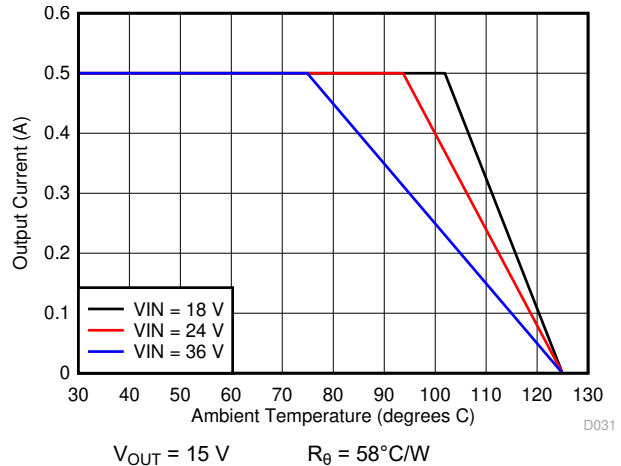
7-22. Ambient Temperature vs Output Current
