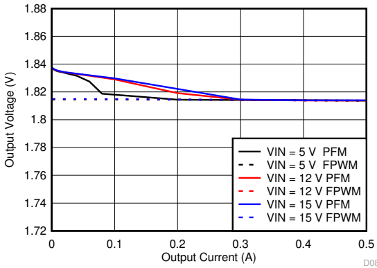
9-38. Line and Load Regulation for V_{OUT} = 1.8\text{ V}
