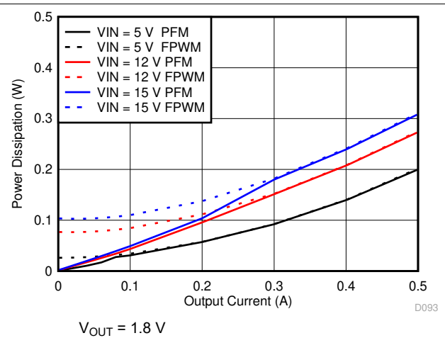
7-14. Power Dissipation
