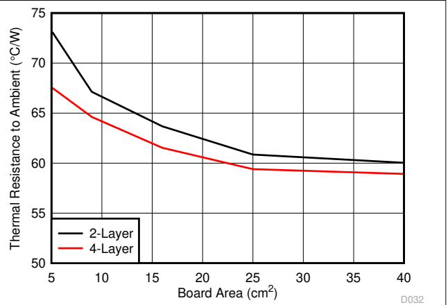
Figure 7-8. Package Thermal Resistance vs Board Copper Area, No Air Flow
