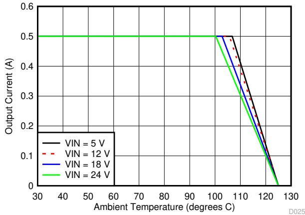
7-19. Ambient Temperature vs Output Current
