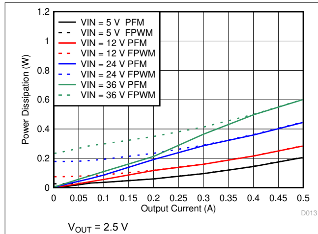
7-13. Power Dissipation
