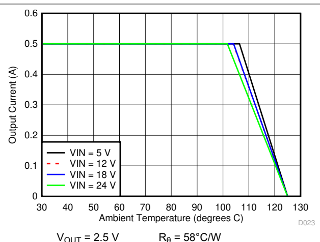
7-18. Ambient Temperature vs Output Current
