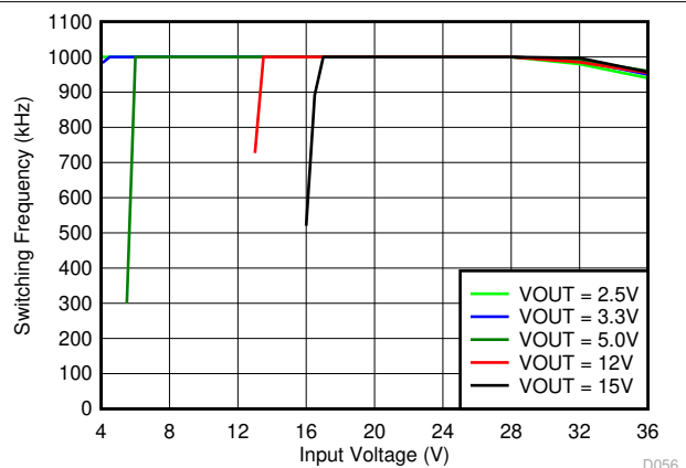
7-30. Switching Frequency vs Input Voltage for Adjustable Output Options at Full Load
