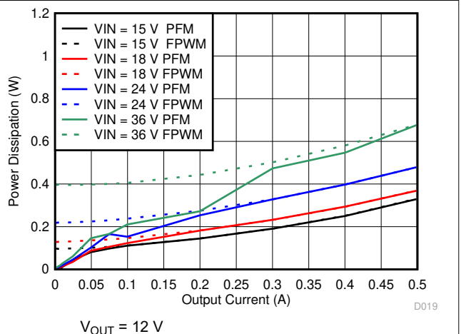
Figure 7-10. Power Dissipation
