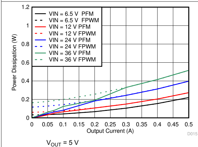
Figure 7-11. Power Dissipation
