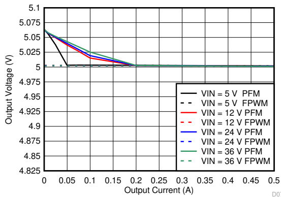
9-44. Line and Load Regulation for V_{OUT} = 5\text{ V}
