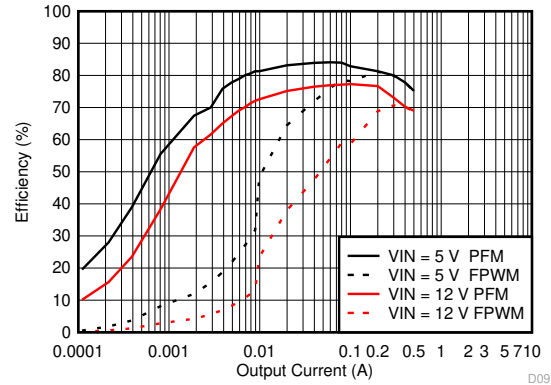
9-37. Efficiency for V_{OUT} = 1.2\text{ V}
