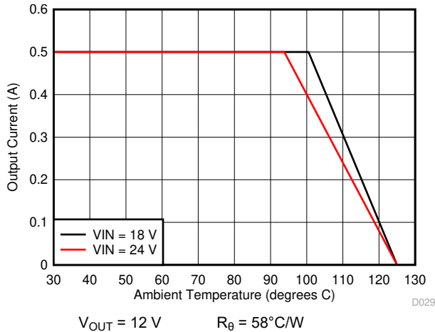
7-21. Ambient Temperature vs Output Current
