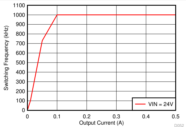
7-26. Auto PFM Mode Switching Frequency vs Output Current
