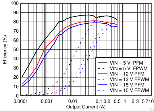
9-36. Efficiency for V_{OUT} = 1.8\text{ V}
