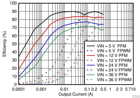
9-30. Efficiency
