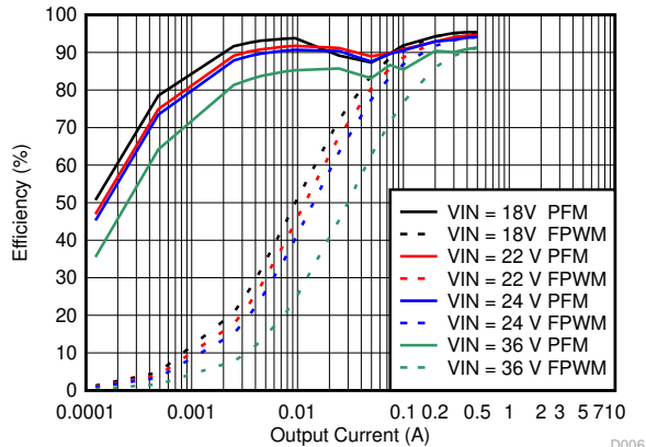
9-24. Efficiency
