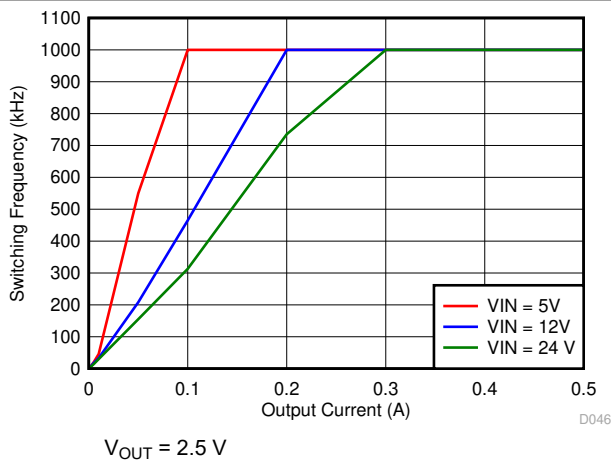
7-23. Auto PFM Mode Switching Frequency vs Output Current
