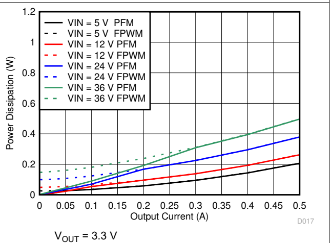
Figure 7-12. Power Dissipation
