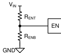
图 9-5. Enable Divider to Set External UVLO Threshold
