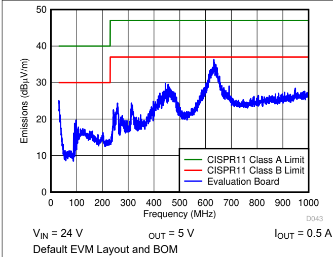
Figure 7-7. Radiated EMI
