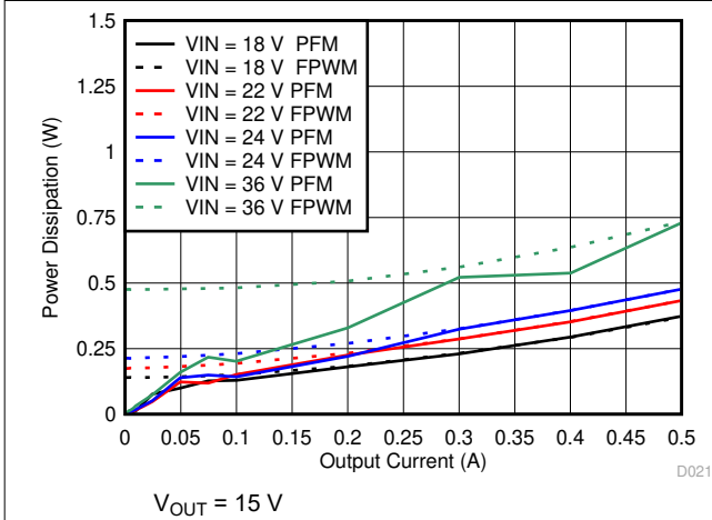
Figure 7-9. Power Dissipation
