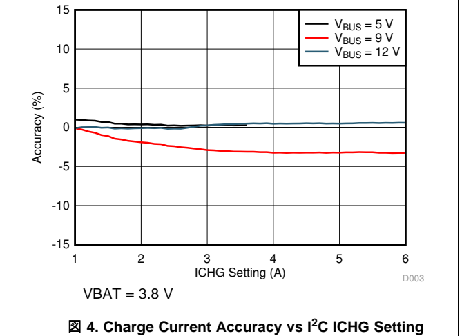
4. Charge Current Accuracy vs I 2 C ICHG Setting
