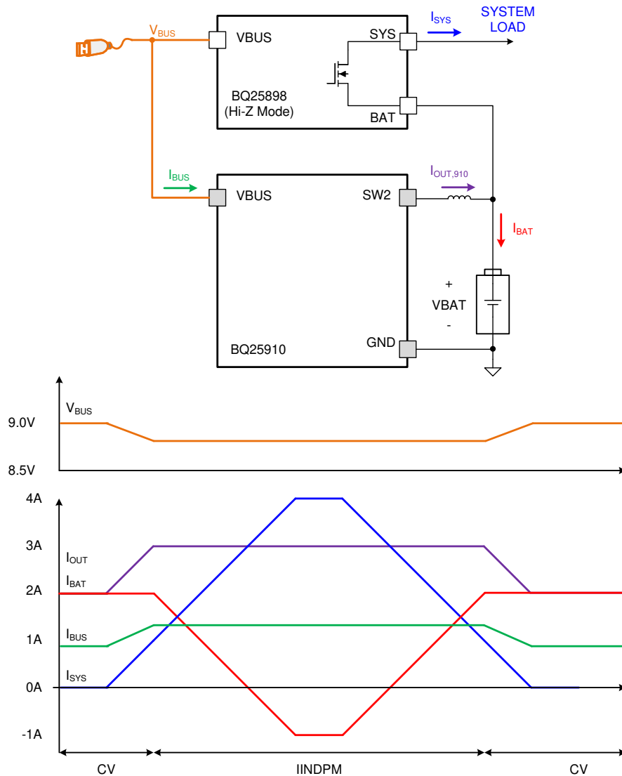
FIG 20. DPM Response
