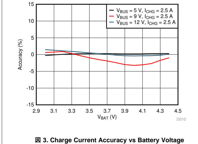
3. Charge Current Accuracy vs Battery Voltage
