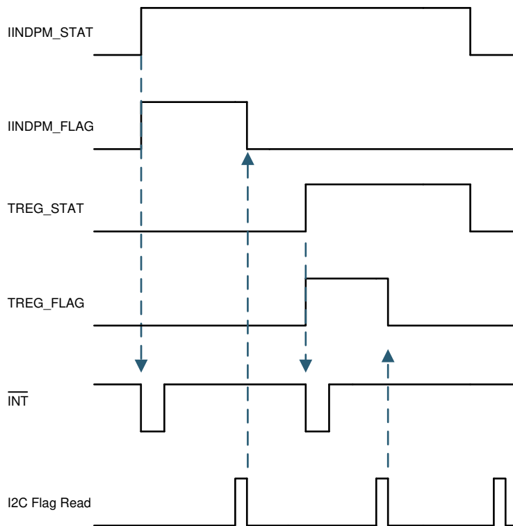
21. \overline{\text{INT}} Generation Behavior Example
