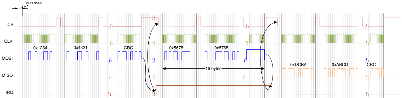
Figure 8-11. SPI Communication
