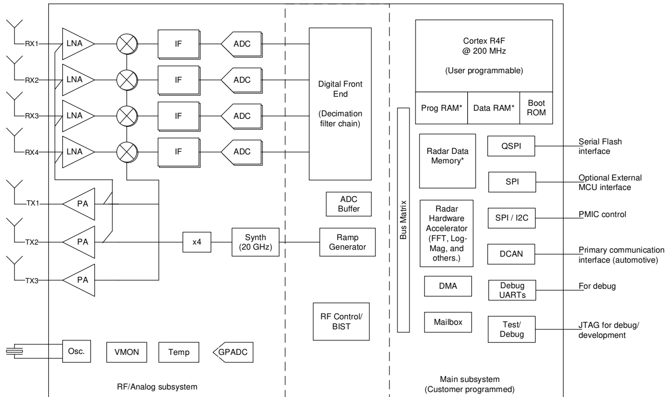
9-1. Functional Block Diagram
