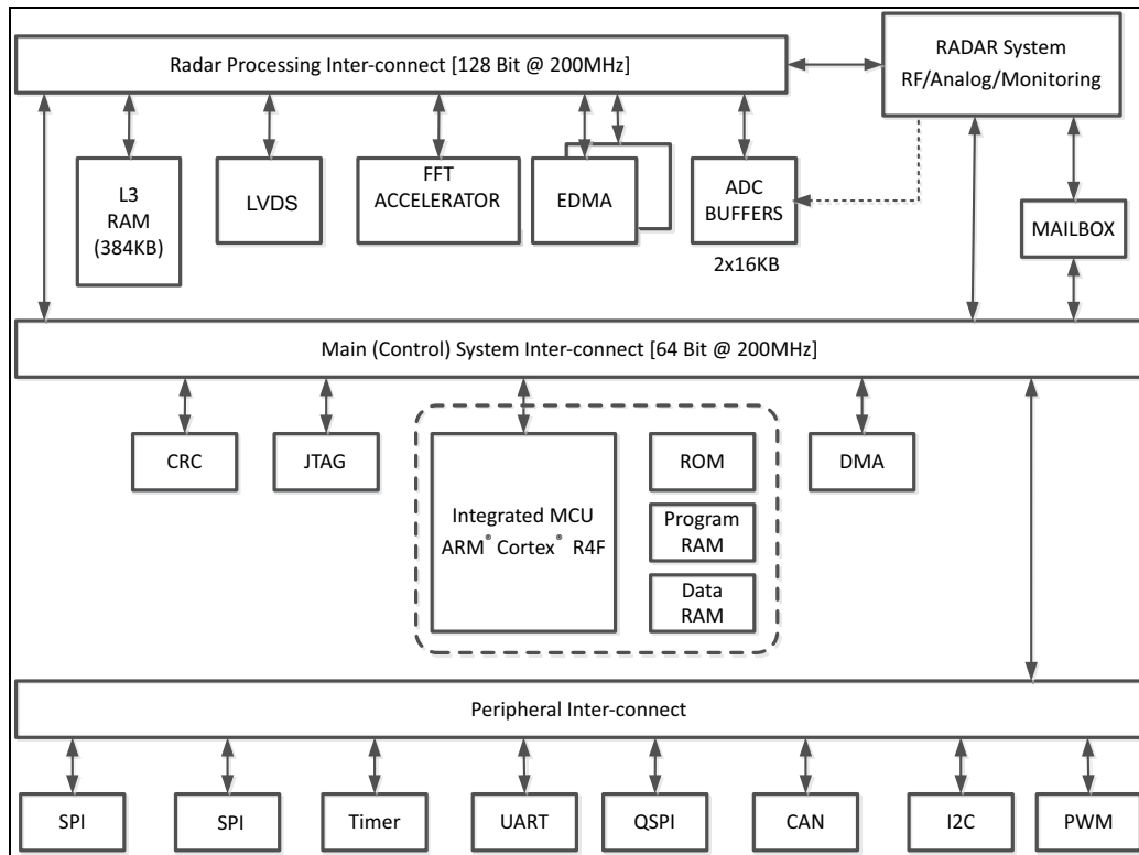
9-2. System Interconnect
