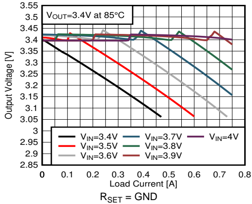
32. Output Voltage versus Load Current V OUT = 3.4 V
