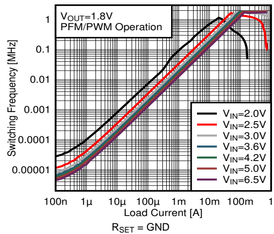
37. Switching Frequency versus Load Current V OUT = 1.8 V
