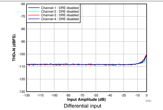
图 6. THD+N vs Input Amplitude With DRE Disabled
