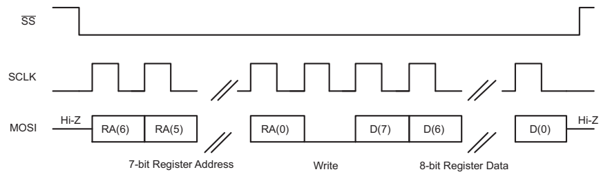
图 93. SPI Single-Byte Write Transfer
