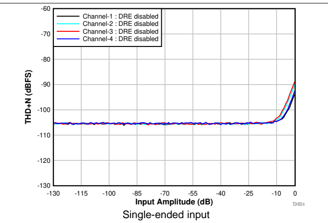
图 8. THD+N vs Input Amplitude With DRE Disabled
