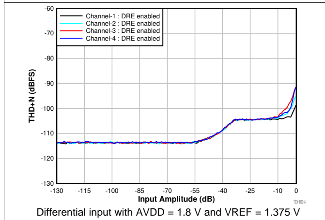
图 9. THD+N vs Input Amplitude With DRE Enabled
