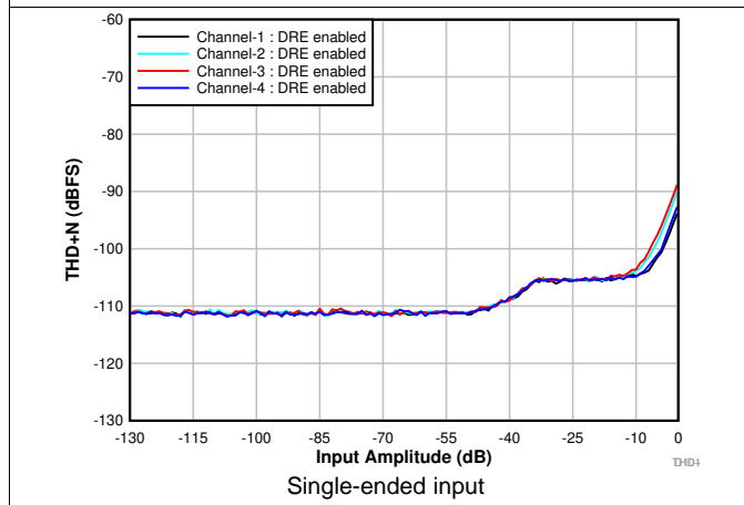
图 7. THD+N vs Input Amplitude With DRE Enabled
