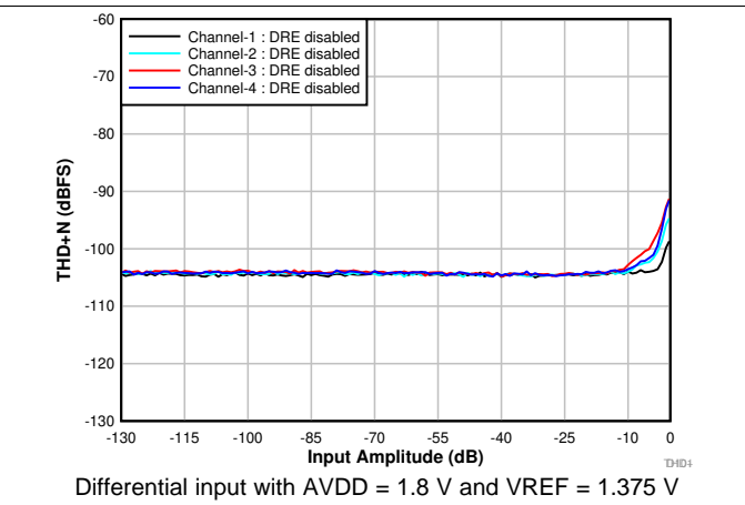
图 10. THD+N vs Input Amplitude With DRE Disabled
