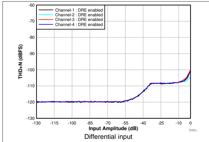
图 5. THD+N vs Input Amplitude With DRE Enabled
