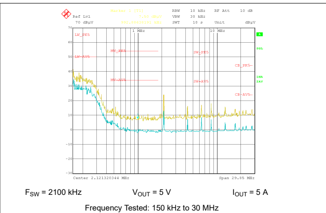
10-54. Conducted EMI versus CISPR25 Limits (Yellow: Peak Signal, Blue: Average Signal)
