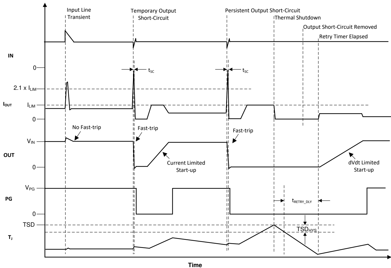
8-4. Input Line Transient and Output Short-Circuit Response
