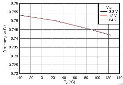
7-21. NRETRY Oscillator Hysteresis vs Temperature
