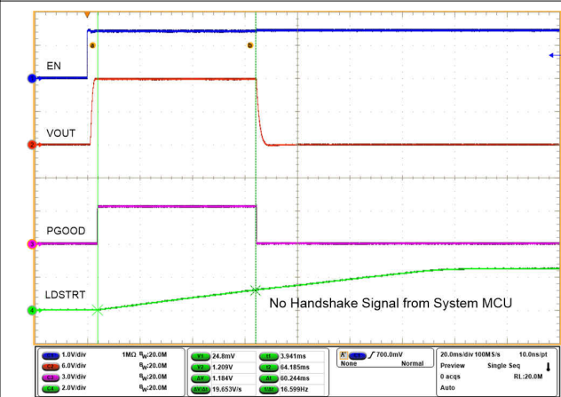
A. C_{LDSTRT} = 0.1 \mu F 9-12. Unsuccessful Load Handshake (LDSTRT)
