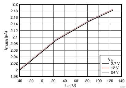
7-14. ITIMER Discharge Current vs Temperature
