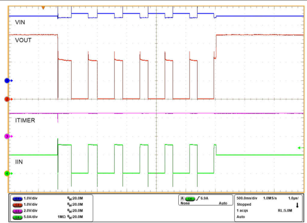
9-18. Overload Response and Recovery
