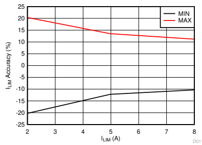
7-11. Output Current Limit ( I_{LIM} ) Accuracy
