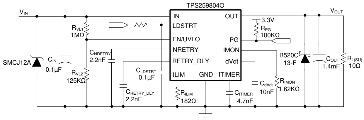
図 9-1. Typical Application Schematic - Input Protection for Patient Monitoring System
