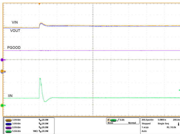
7-33. Supply Line Transient Immunity - Input Voltage Step
