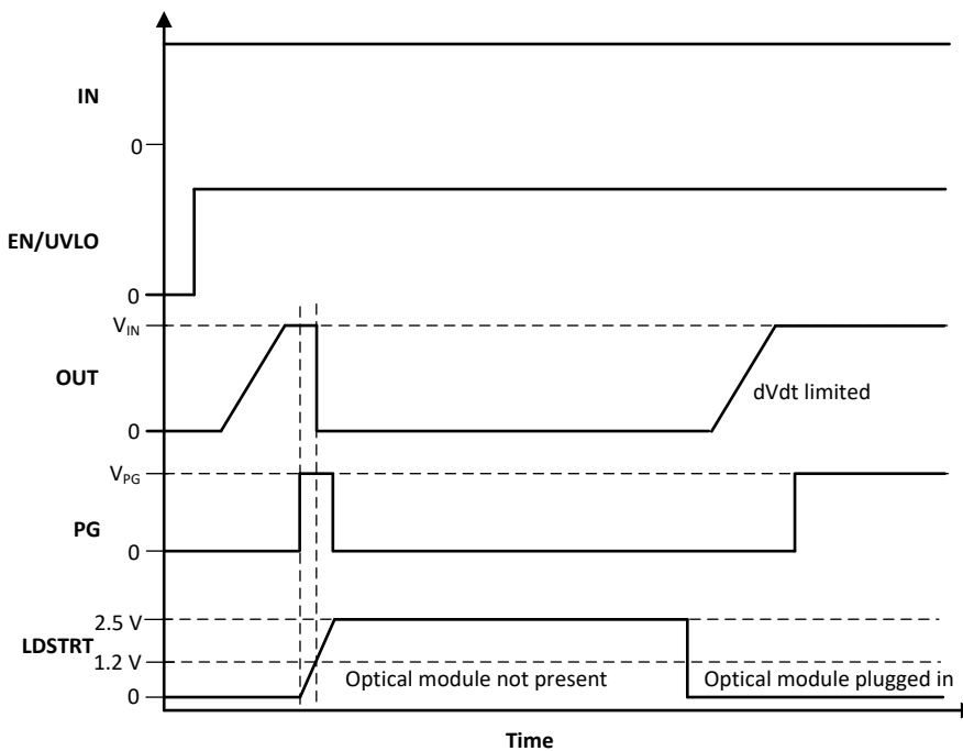
8-8. Optical Module Plug-In Detection Using LDSTRT
