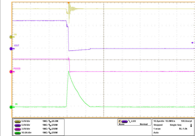
A. R_{LIM} = 182 \Omega 9-8. Output Hard Short-Circuit While ON (Zoomed In)
