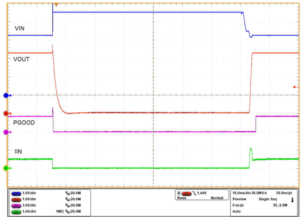
9-20. Overvoltage Protection Response and Recovery with TPS259802O Device
