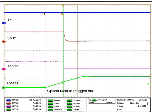
9-16. Output Voltage Profile When Optical Module is Plugged Out
