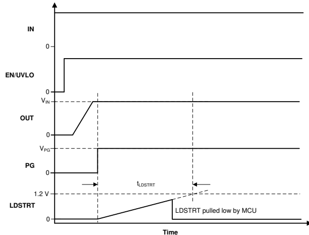
8-6. Successful LDSTRT Handshake
