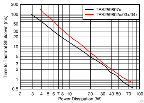
7-23. Thermal Shutdown Plot - Inrush/Overload
