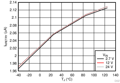
7-20. NRETRY Bias Current vs Temperature
