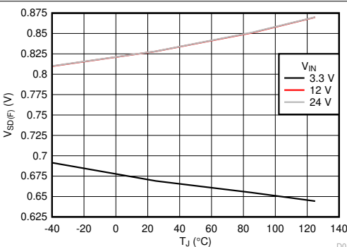
7-7. EN/UVLO Falling Threshold for Lowest Current Consumption
