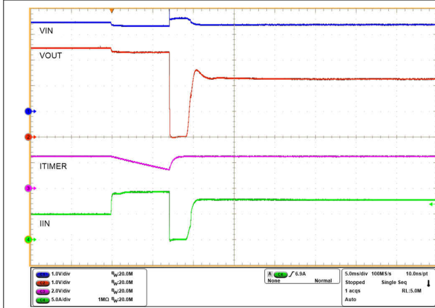
9-17. Circuit Breaker With Transient Overcurrent Blanking Interval of 6 ms; Device Restarts in Current Limit Mode
