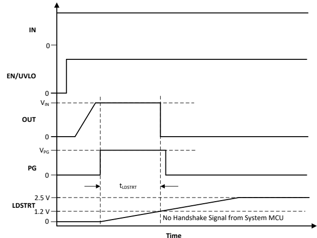
8-7. Unsuccessful LDSTRT Handshake
