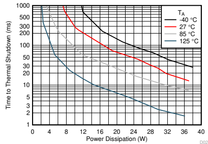
7-22. Thermal Shutdown Plot - Steady State
