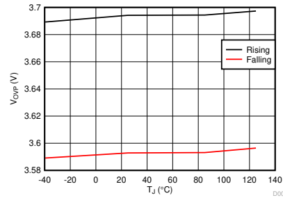
7-2. Supply OVP Threshold vs Temperature
