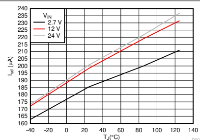
7-8. Shut-Down Current vs Temperature
