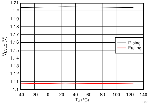
7-5. EN/UVLO Threshold vs Temperature
