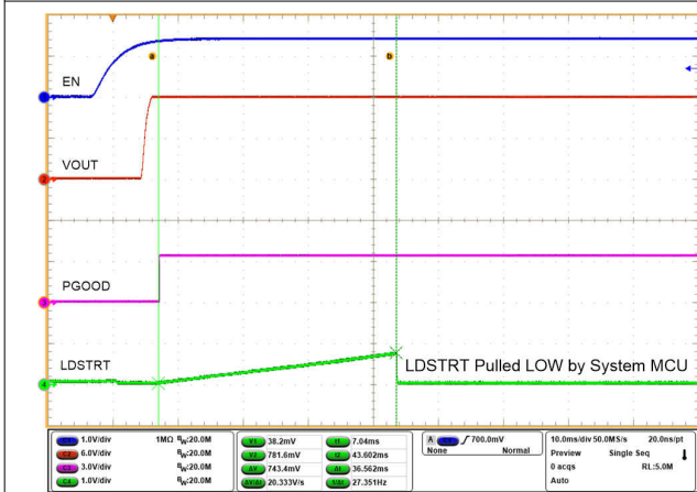
A. C_{LDSTRT} = 0.1 \mu F 9-11. Successful Load Handshake (LDSTRT)
