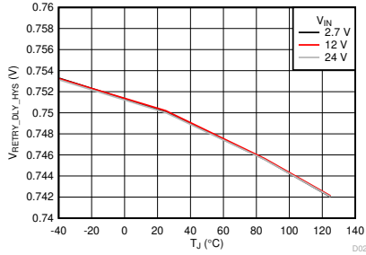
7-19. RETRY_DLY Oscillator Hysteresis vs Temperature
