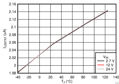
7-15. LDSTRT Charging Current vs Temperature
