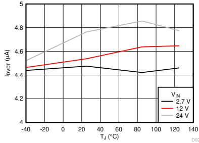
7-17. DVDT Charging Current vs Temperature
