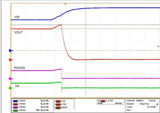
9-19. Overvoltage Cut-off at 3.7 V with TPS259802O Device
