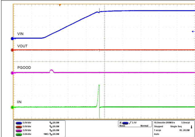
A. R_{LIM} = 182 \Omega 9-9. Power-Up With Short-Circuit on Output
