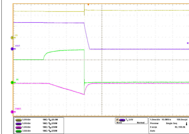
A. R_{LIM} = 182 \Omega C_{TIMER} = 4.7 \text{ nF}
