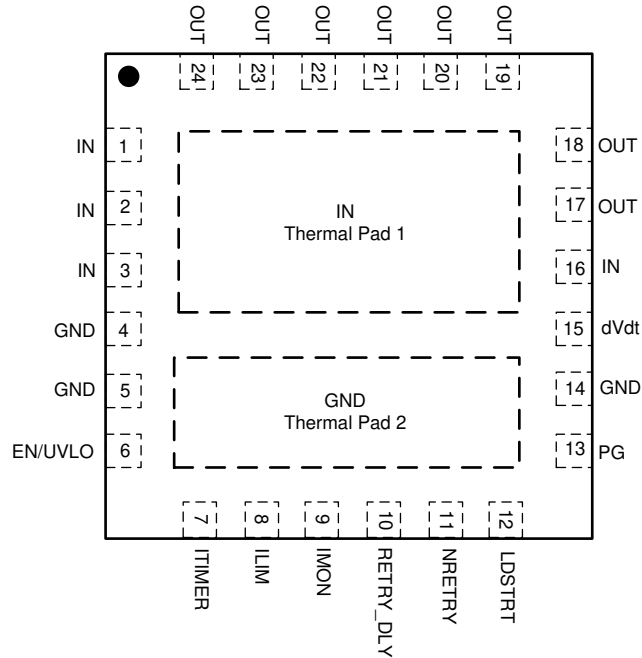
6-1. RGE 24-Pin QFN Top View
