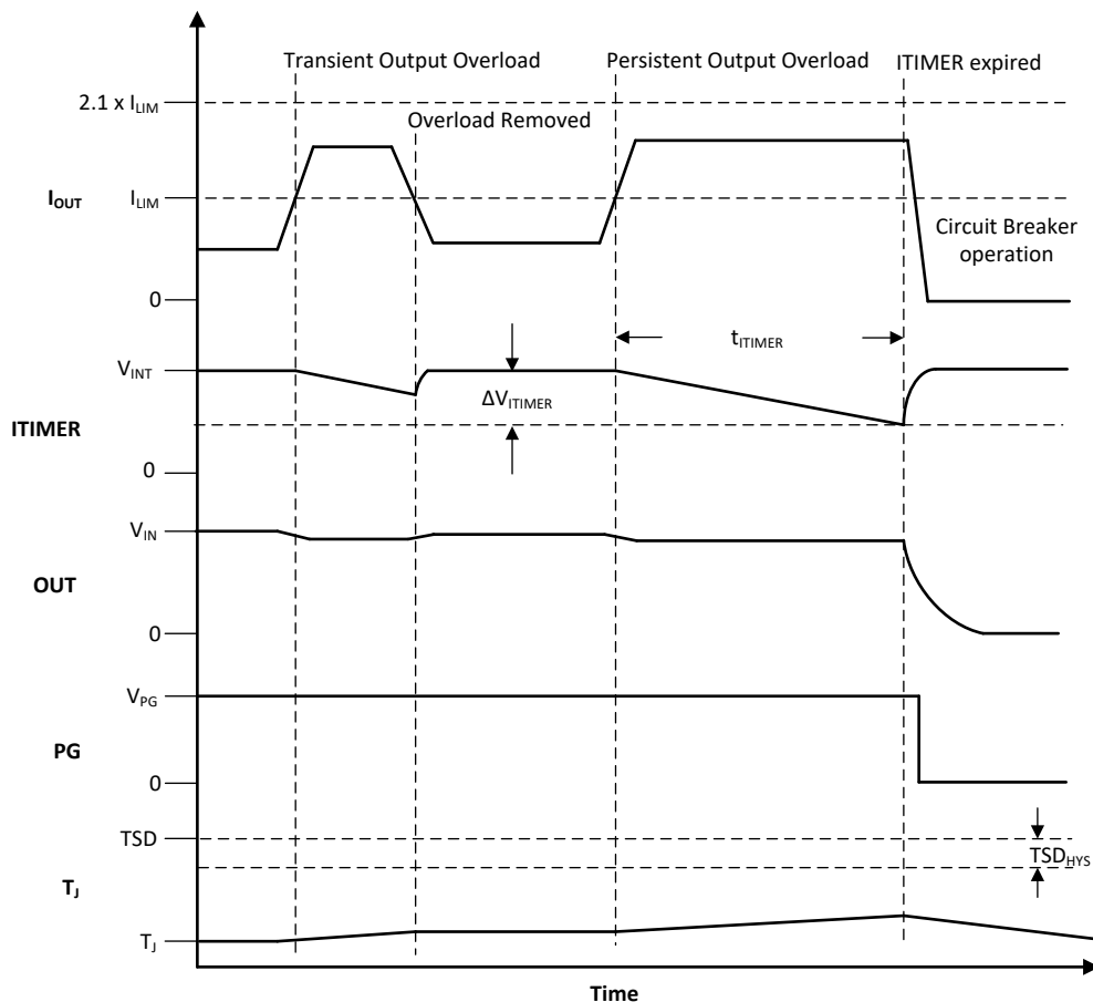
8-3. Circuit Breaker Response
