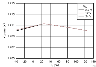
7-16. LDSTRT Threshold Voltage vs Temperature
