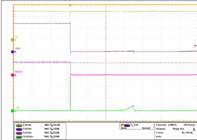
A. R_{LIM} = 182 \Omega 9-7. Output Hard Short-Circuit While ON
