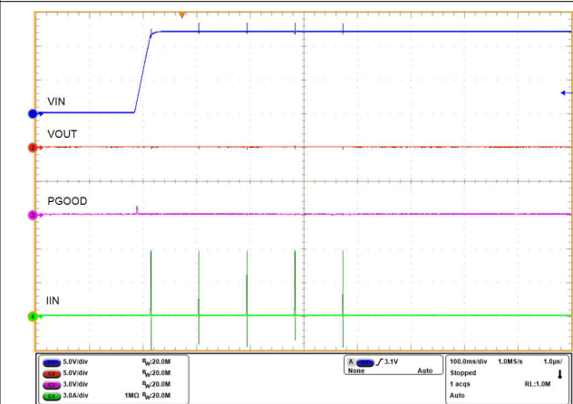
A. R_{LIM} = 182 \Omega 9-10. Power-Up With Short-Circuit on Output - Auto-Retry 4 Times With Retry Delay of 100 ms
