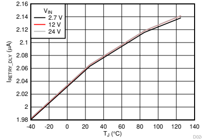
7-18. RETRY_DLY Bias Current vs Temperature
