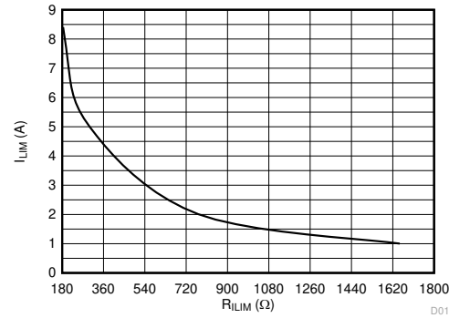
7-10. Output Current Limit ( I_{LIM} ) vs R_{LIM}
