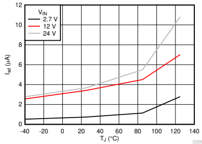
7-9. Deep Shut-Down Current vs Temperature
