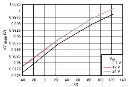
7-13. ITIMER Voltage Threshold Delta vs Temperature
