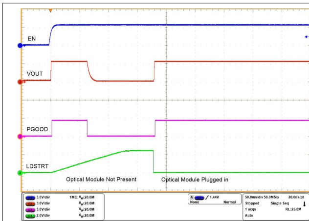
9-15. Output Voltage Profile When Optical Module is Inserted
