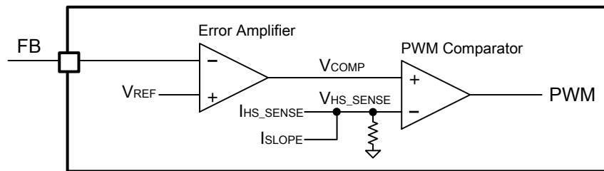
7-1. Error Amplifier and PWM Comparator
