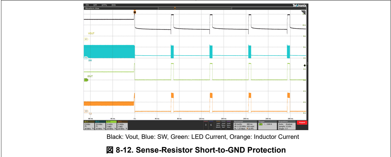
Black: Vout, Blue: SW, Green: LED Current, Orange: Inductor Current
