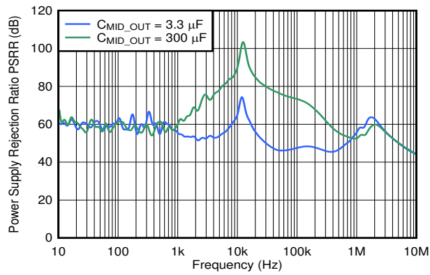
6-37. MID_OUT PSRR vs Frequency and C_{MID\_OUT}
