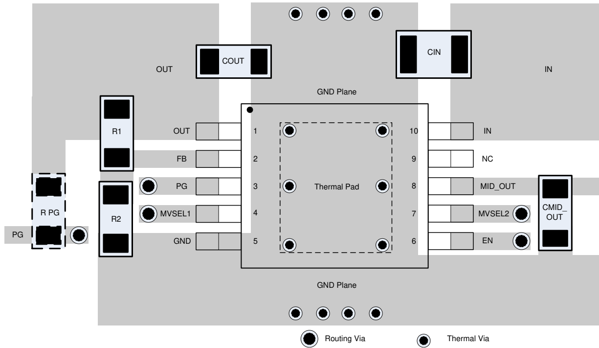
8-4. Adjustable Version Layout Example
