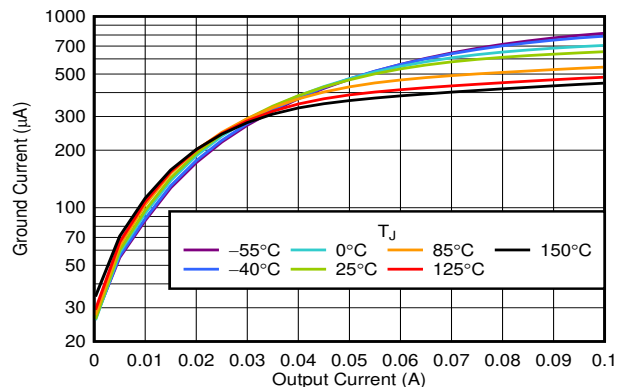
图 6-6. I_{GND} vs I_{OUT} ( MID\_OUT in Dropout)
