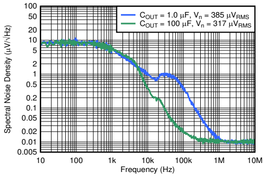
6-31. Spectral Noise Density vs Frequency and C_{\text{OUT}}
