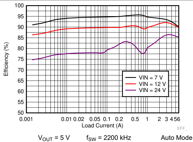
8-7. TPS7H4010-SEP Efficiency
