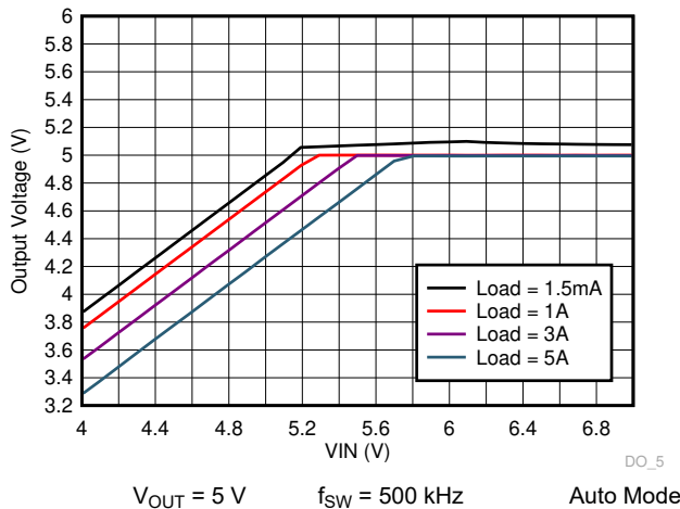
8-13. TPS7H4010-SEP Dropout Curve
