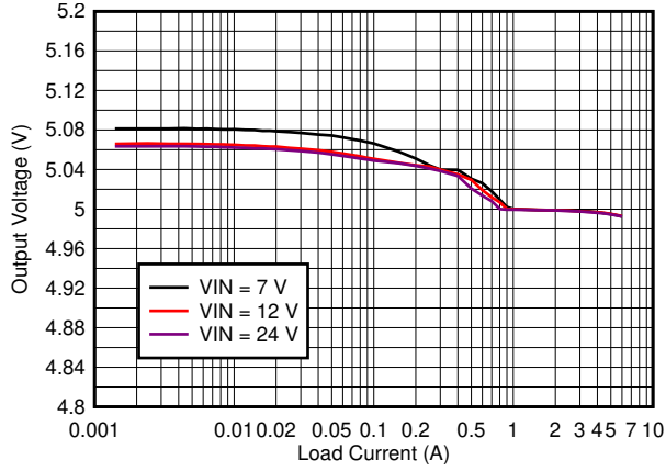
8-9. TPS7H4010-SEP Load and Line Regulation
