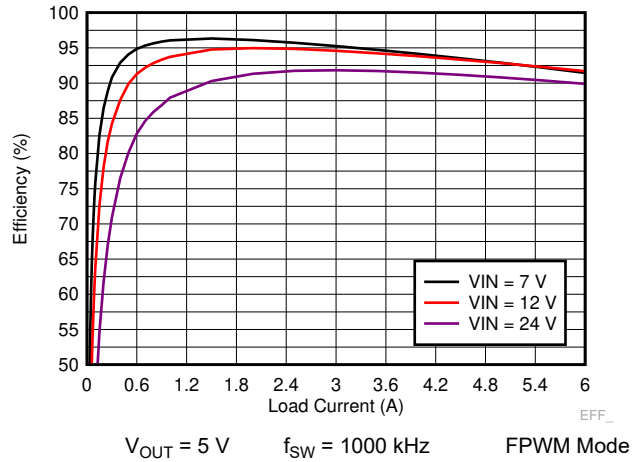
8-6. TPS7H4010-SEP Efficiency
