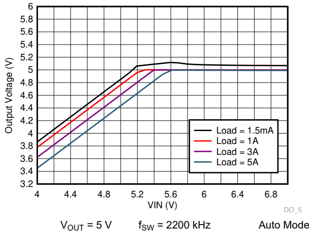
8-11. TPS7H4010-SEP Dropout Curve
