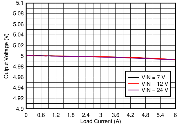
8-10. TPS7H4010-SEP Load and Line Regulation
