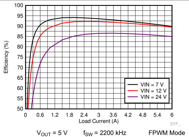
8-8. TPS7H4010-SEP Efficiency
