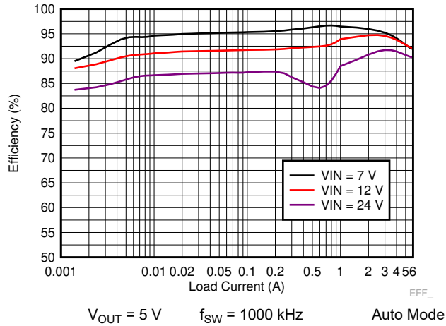
8-5. TPS7H4010-SEP Efficiency
