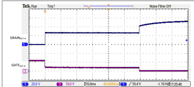
10-3. I_{LIM} Foldback and Turn-Off
