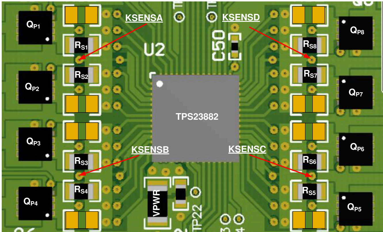
12-3. Eight Port Layout Example (Top Side)
