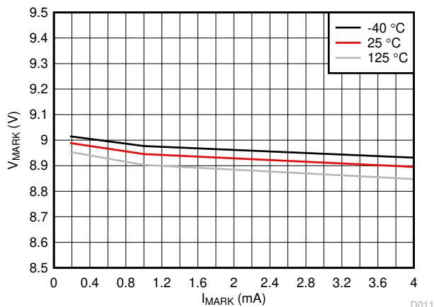
7-11. Mark Voltage vs I_{MARK} and Temperature
