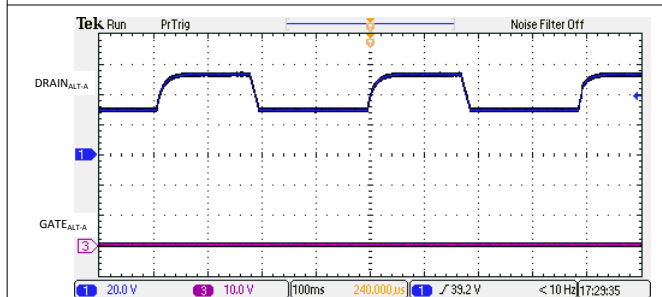
10-5. Open Circuit Detection Signature
