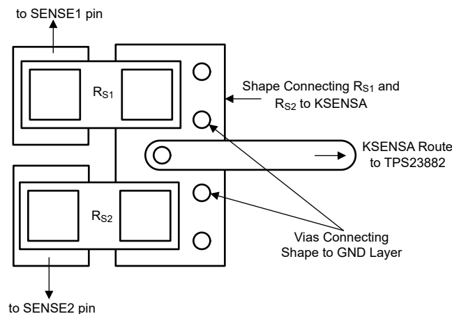
12-2. Kelvin Sense Layout Example
