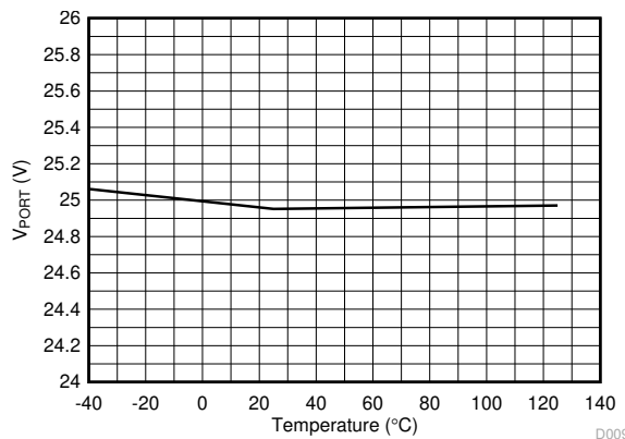
7-9. Discovery Open Circuit Voltage vs Temperature
