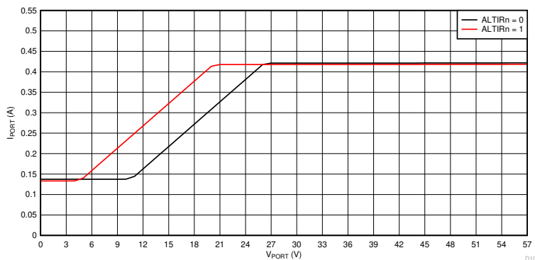
图 9-76. Inrush Foldback Curves, I PORT vs V PORT
