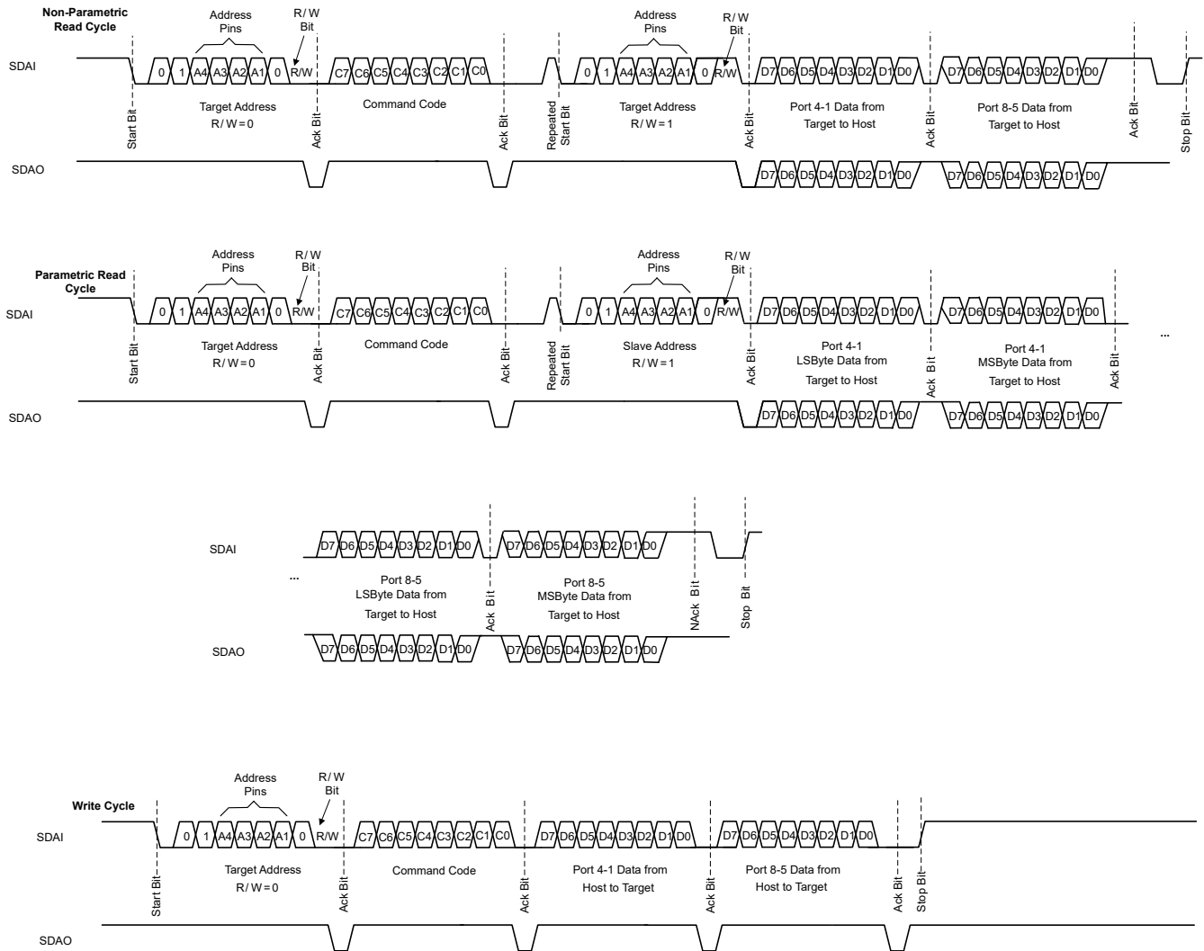
9-5. I 2 C interface Read and Write Protocol – Configuration B
