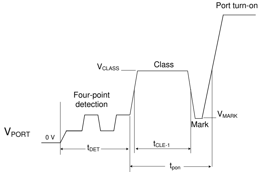
☒ 8-3. 2-Pair Detection, 1-Event Classification and Turn On
