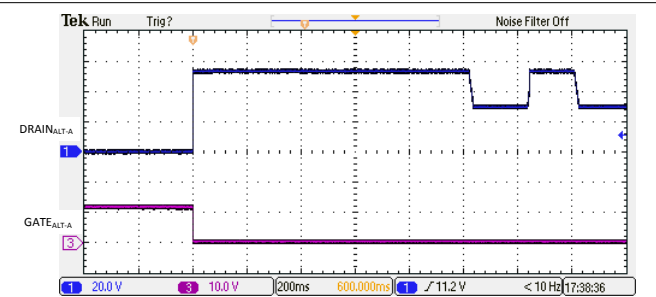
10-4. Backoff Due to PCut Fault
