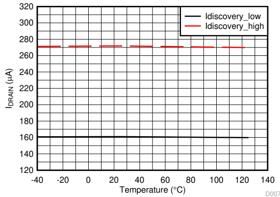
7-7. Discovery Currents vs Temperature
