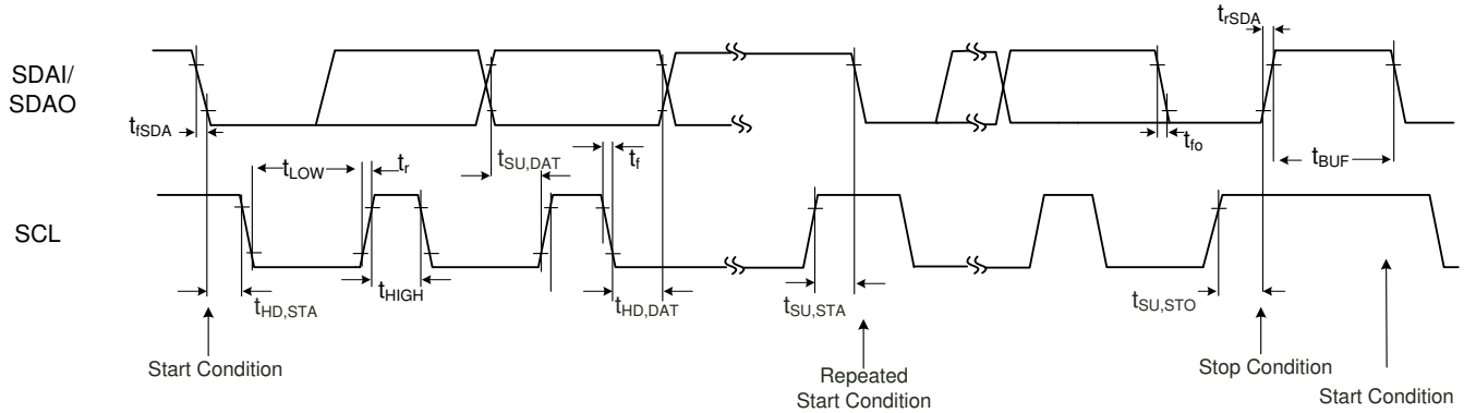
8-1. I 2 C Timings
