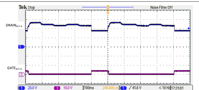
10-6. Semiauto Mode Discovery with a Valid Class 0-3 Load
