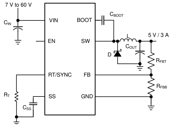
Figure 8-1. Application Circuit, 5-V Output
