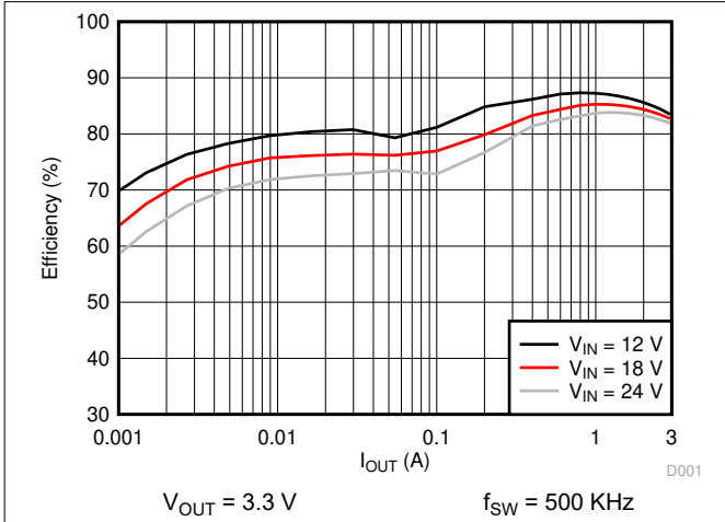
6-1. Efficiency vs. Load Current
