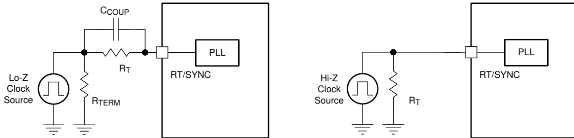
7-5. Synchronizing to an External Clock
