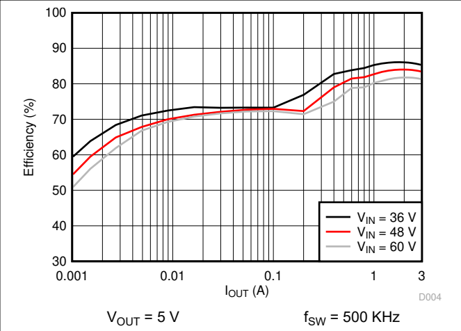
6-4. Efficiency vs. Load Current
