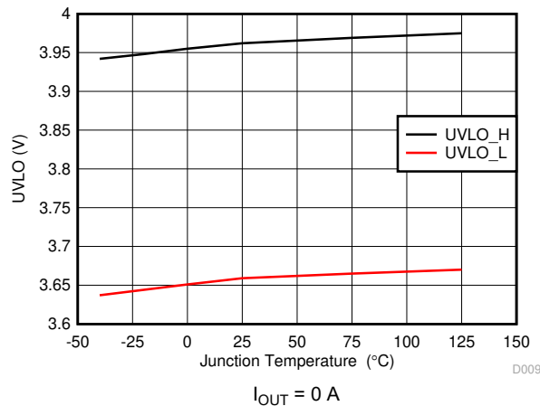
6-12. UVLO Threshold
