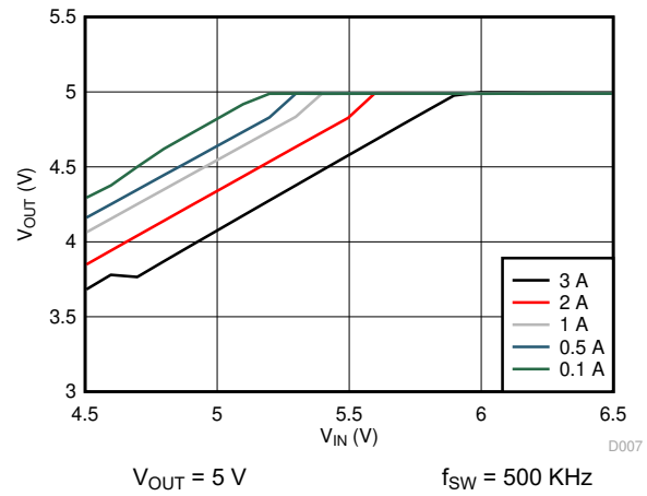
6-8. Dropout Curve
