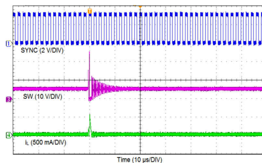
7-8. Synchronizing in Sleep Mode
