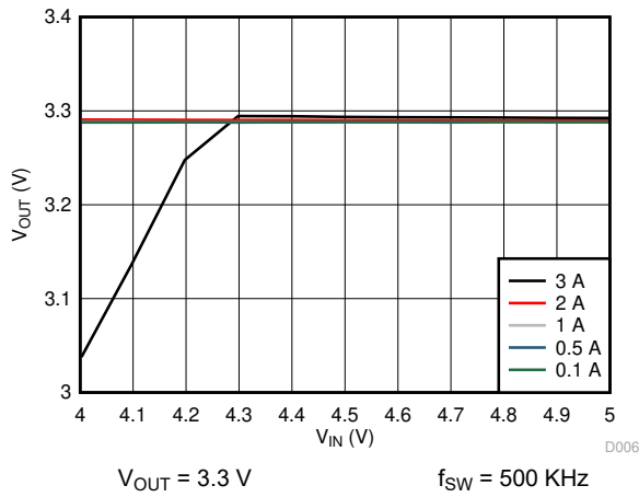
6-7. Dropout Curve
