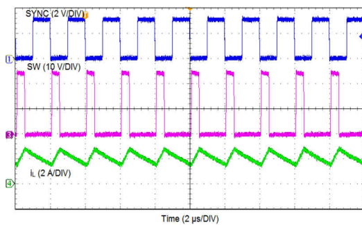
7-6. Synchronizing in CCM
