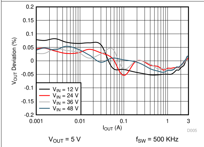
6-5. Load Regulation
