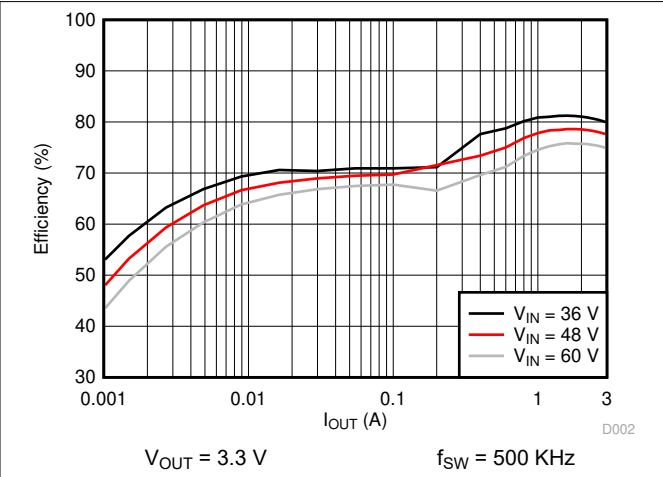
6-2. Efficiency vs. Load Current
