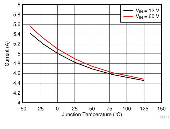
6-10. High-Side Current Limit vs Junction Temperature
