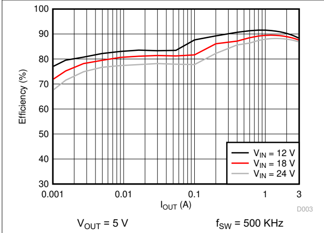
6-3. Efficiency vs. Load Current
