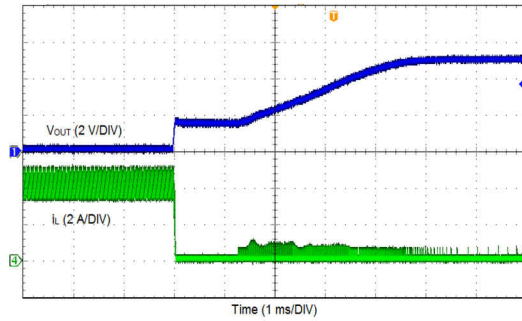
8-9. Output Short Recovery
