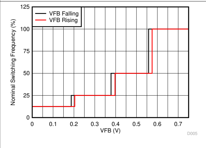
6-6. Frequency vs V_{FB}
