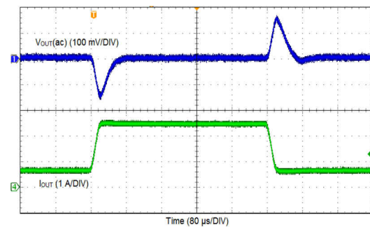
8-5. DCM Mode
