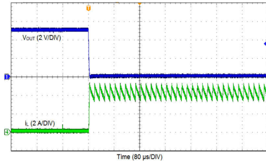
8-8. Output Short
