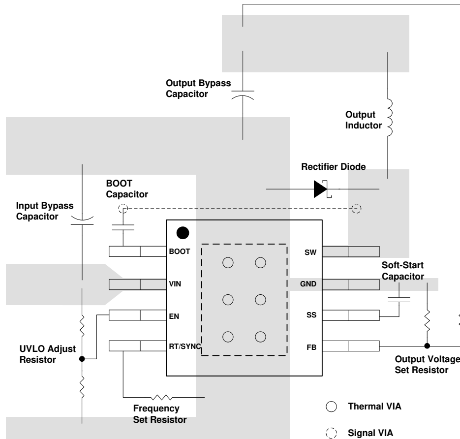
10-1. Layout
