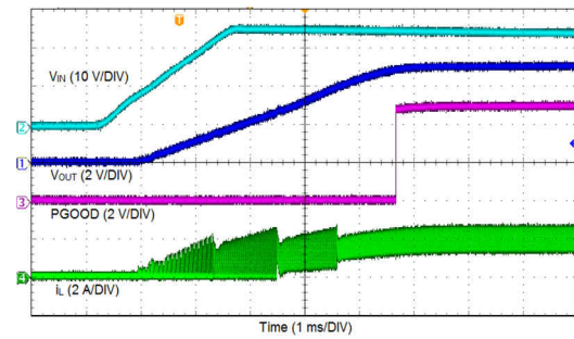
8-3. Start-up By V_{IN}
