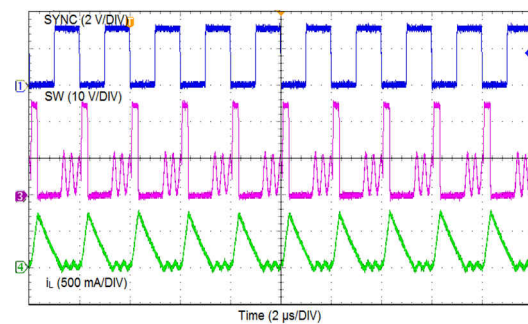
7-7. Synchronizing in DCM
