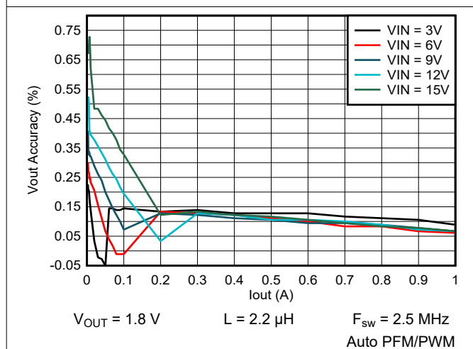
9-30. Output Voltage vs Output Current
