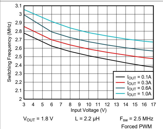
9-29. Switching Frequency vs Input Voltage
