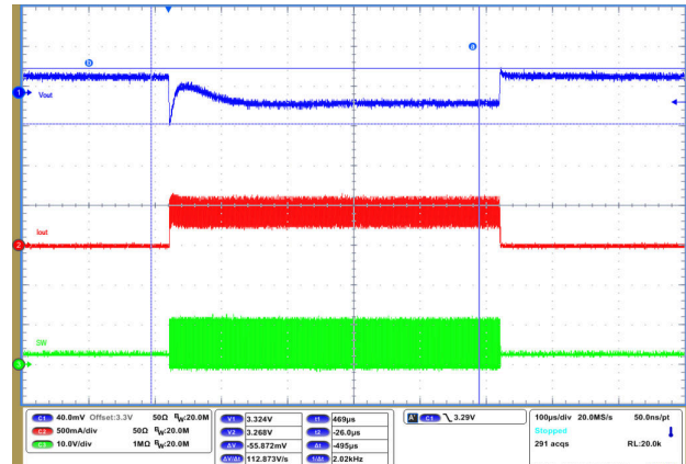
9-69. Shutdown Timing with Output Discharge Enabled
