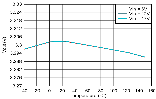
Figure 7-5. Output Voltage Accuracy – VSET Selected
