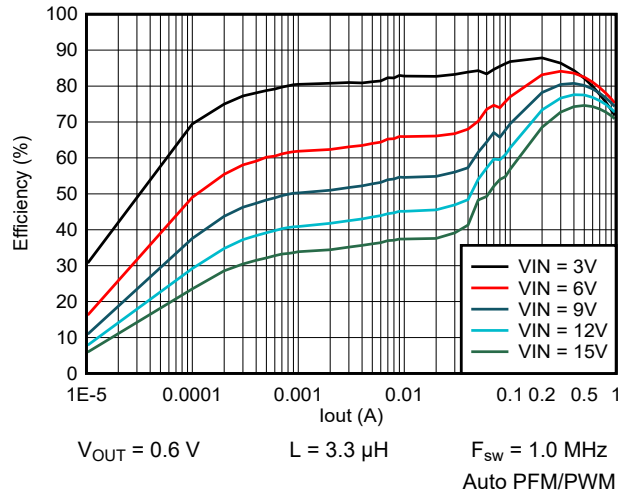
Figure 9-56. Efficiency vs Output Current
