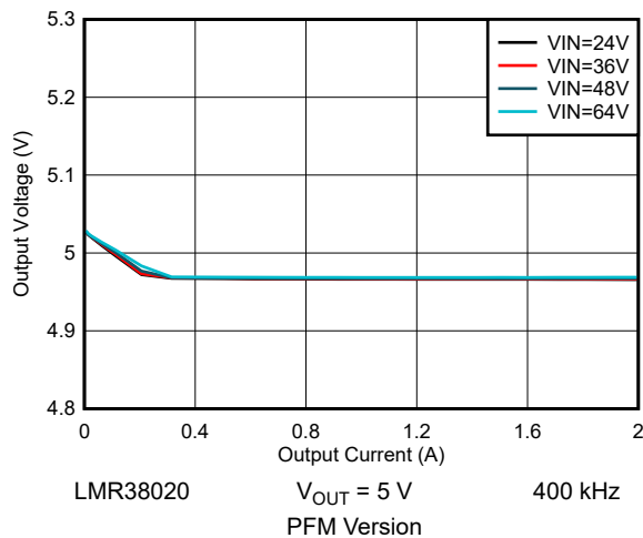
9-13. 5-V Load Regulation
