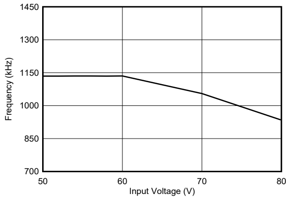
☒ 8-8. Typical Frequency Foldback at T ON_MIN
