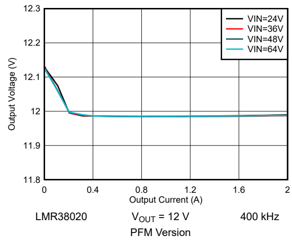
9-14. 12-V Load Regulation
