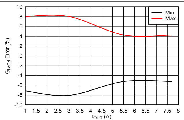
7-14. Analog Current Monitor Gain Accuracy
