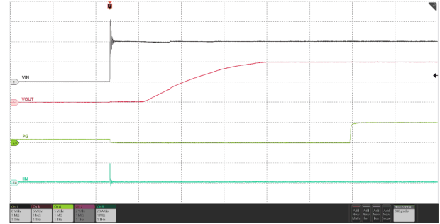
7-32. Input Hot-Plug
