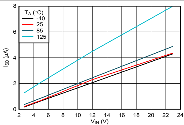
7-5. IN Shutdown Current vs Temperature
