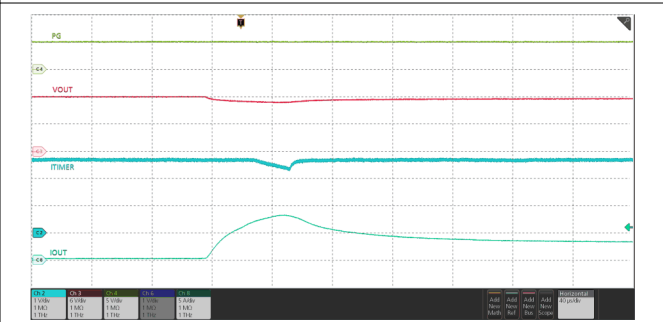
V IN = 12 V, C ITIMER = 120 pF, C OUT = 470 μF, R ILM = 715 Ω, I OUT ramped from 0 A → 8 A → 4 A within 100 μs
