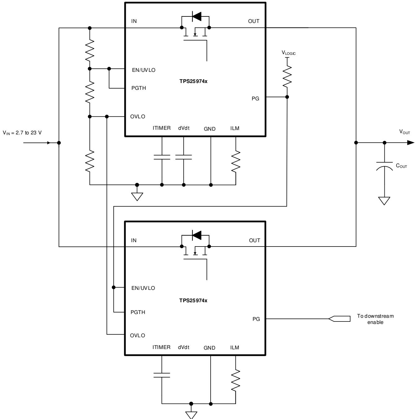
9-7. Two Devices Connected in Parallel for Higher Steady State Current Capability
