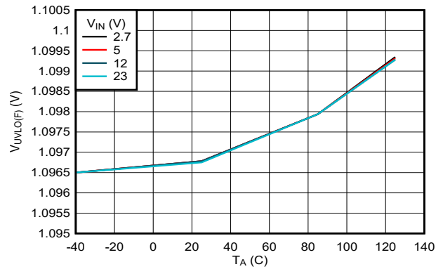
7-8. EN/UVLO Falling Threshold vs Temperature
