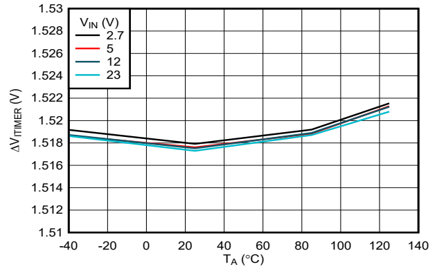
7-20. ITIMER Discharge Differential Voltage Threshold vs Temperature
