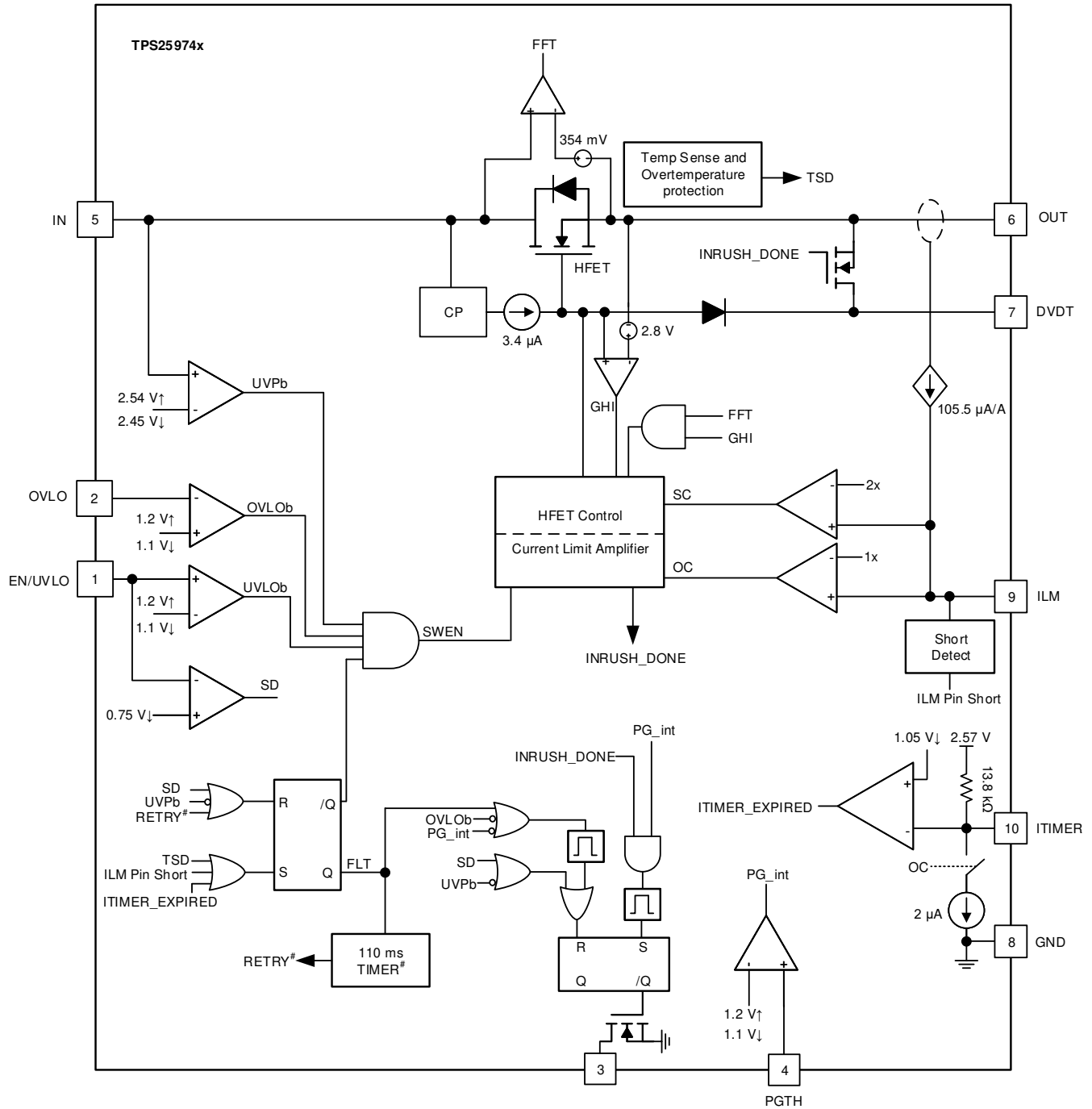
8-3. TPS25974x Block Diagram
