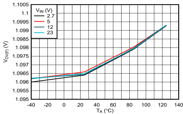
7-11. OVLO Falling Threshold vs Temperature (TPS25970x, TPS25974x Variants)
