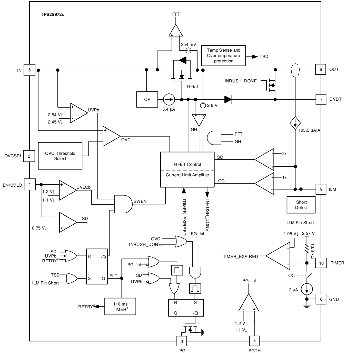
8-2. TPS25972x Block Diagram
