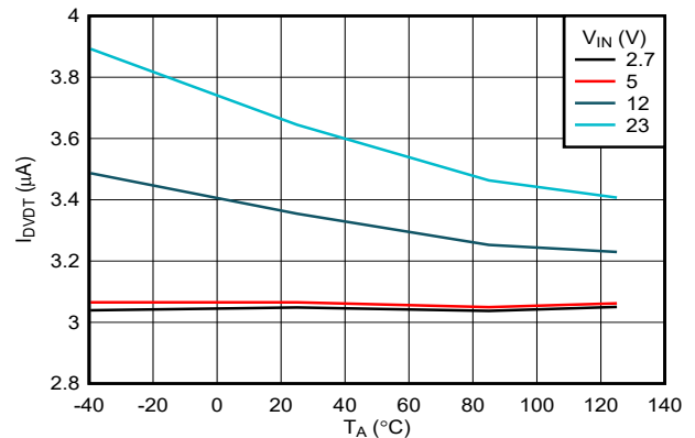
7-24. DVDT Charging Current vs Temperature
