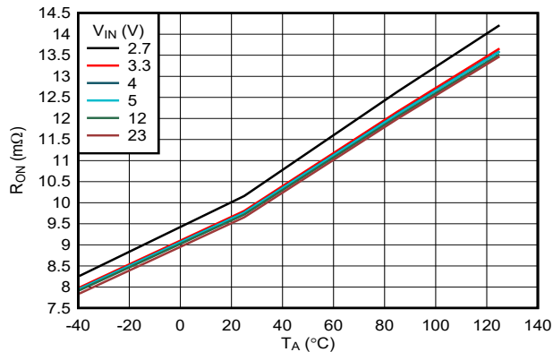
7-1. ON-Resistance vs Supply Voltage
