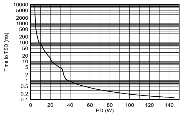
7-28. Time to Thermal Shut-Down During Inrush State
