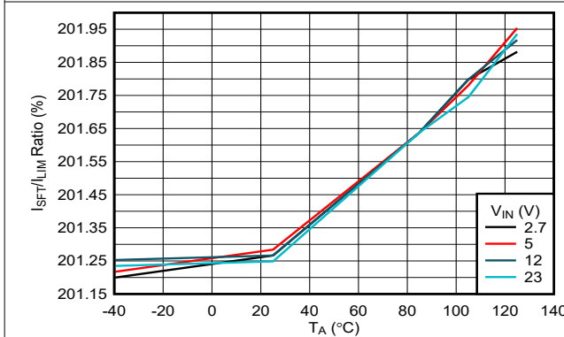
7-15. Scalable Fast-Trip Threshold: Current Limit Threshold ( I_{LIM} ) Ratio vs Temperature
