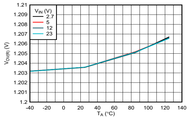
7-10. OVLO Rising Threshold vs Temperature (TPS25970x, TPS25974x Variants)
