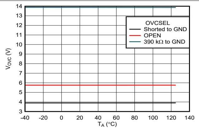
7-16. OVC Threshold vs Temperature (TPS25972x Variant)
