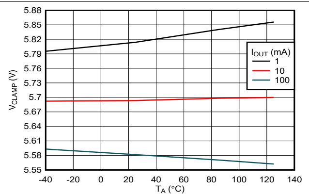
7-18. OVC Clamping Voltage (OVCSEL = OPEN) vs Load Current (TPS25972x Variant)
