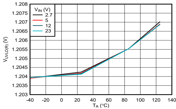
7-7. EN/UVLO Rising Threshold vs Temperature
