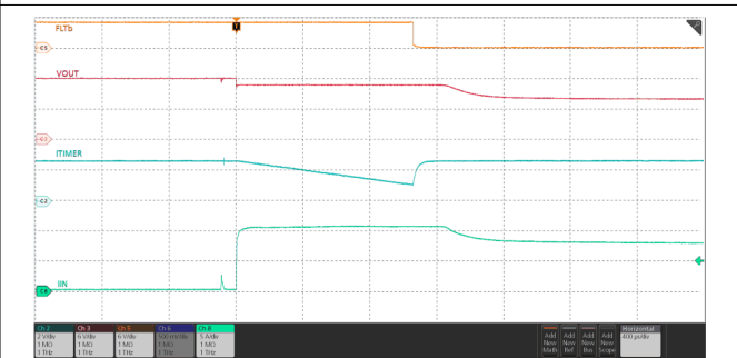
V IN = 12 V, C ITIMER = 1.3 nF, C OUT = 220 μF, R ILM = 715 Ω, I OUT stepped from 0 A → 11 A
