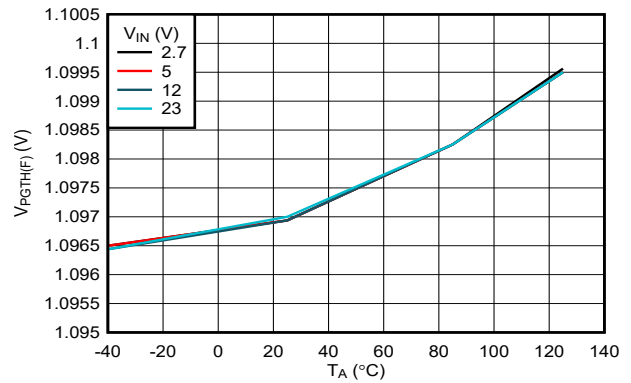
7-26. PGTH Threshold (Falling) vs Temperature (TPS25972x, TPS25974x Variants)
