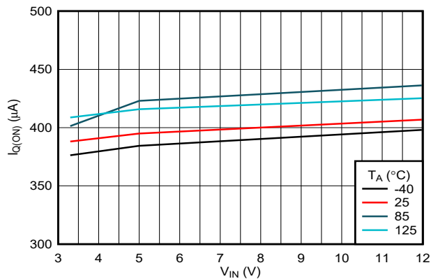
7-3. IN Quiescent Current vs Temperature (TPS25972x Variant)
