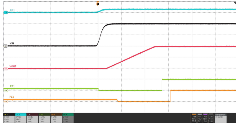
9-8. Parallel Devices Sequencing During Start-Up
