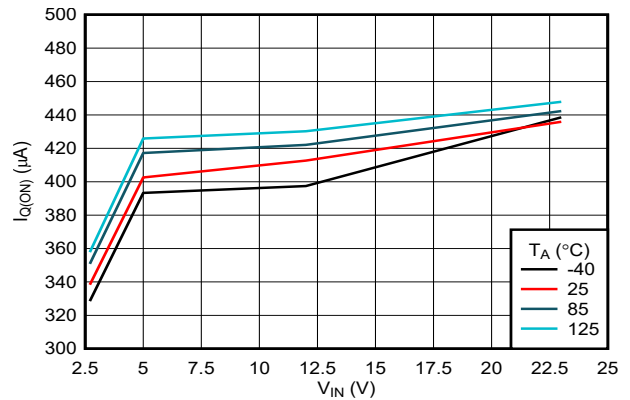
7-2. IN Quiescent Current vs Temperature (TPS25970x, TPS25974x Variants)
