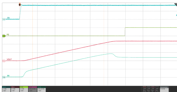
7-33. Inrush Current Without Slew Rate Control – Capacitive Load
