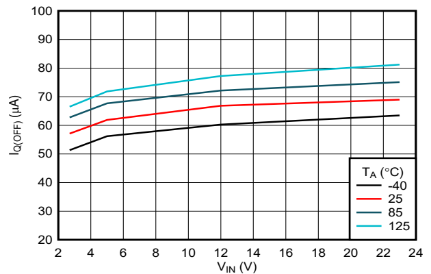
7-4. IN OFF State (UVLO) Current vs Temperature
