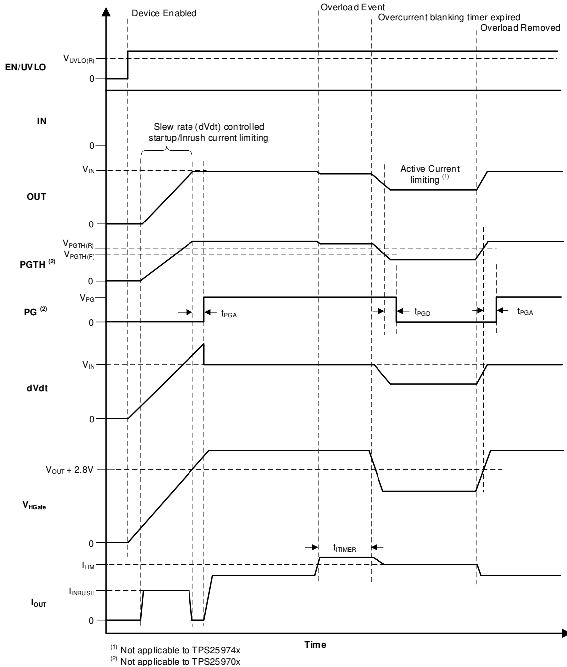
8-13. TPS25972x, TPS25974x PG Timing Diagram
