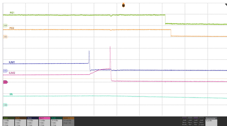
9-9. Parallel Devices Load Current During Steady State and Overload
