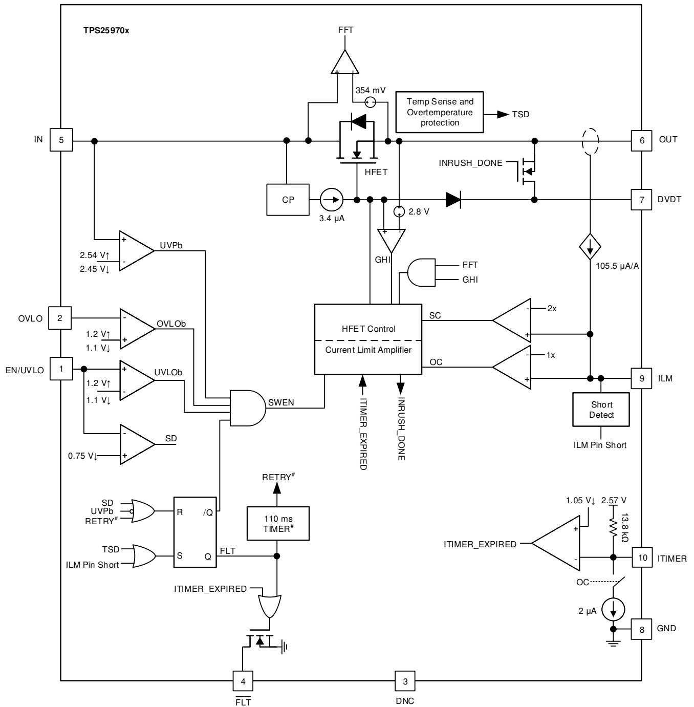
8-1. TPS25970x Block Diagram
