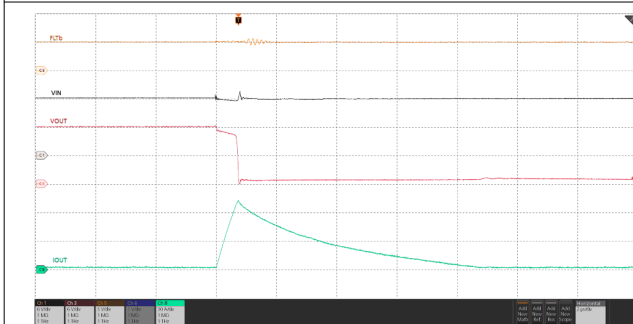
7-43. Circuit-Breaker Response TPS25974x
