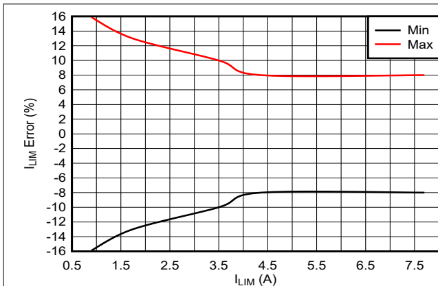
7-13. Overcurrent Threshold Accuracy (Across Process, Voltage and Temperature)
