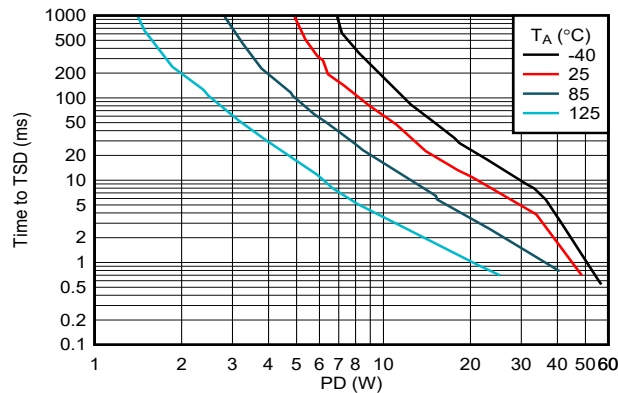
7-29. Time to Thermal Shut-Down During Steady State
