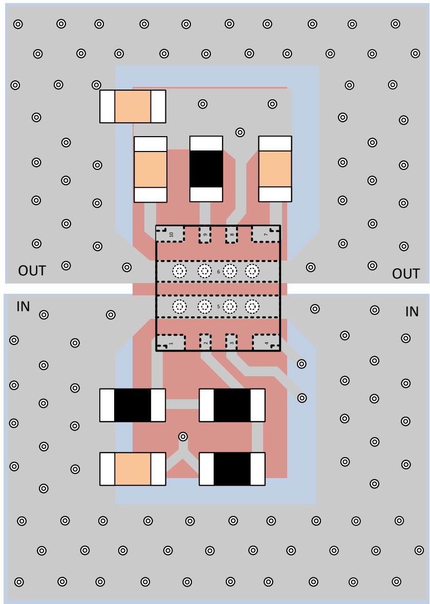
9-11. Layout Example - Single TPS25974x With PGTH Referred to OUT
