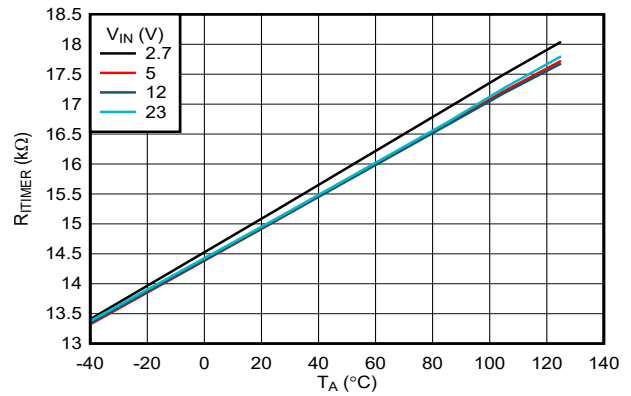
7-22. ITIMER Internal Pullup Resistance vs Temperature
