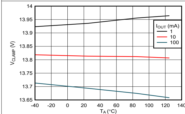
7-17. OVC Clamping Voltage (OVCSEL = 390 kΩ to GND) vs Load Current (TPS25972x Variant)
