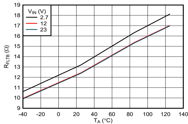
7-27. FLT Pin Pulldown Resistance vs Temperature
