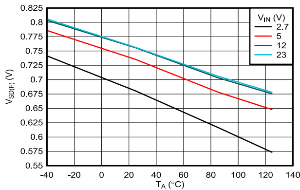
7-9. EN/UVLO Shutdown Falling Threshold vs Temperature
