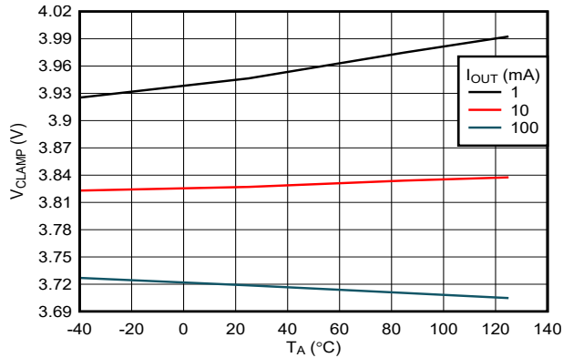
7-19. OVC Clamping Voltage (OVCSEL = GND) vs Load Current (TPS25972x Variant)
