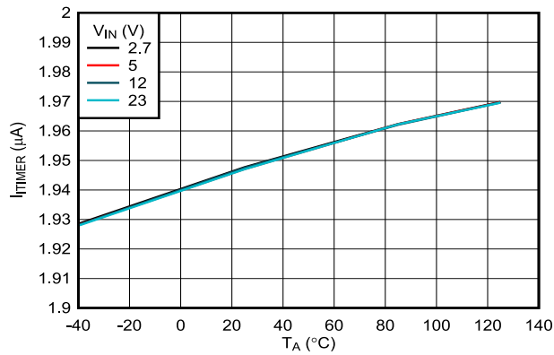
7-21. ITIMER Discharge Current vs Temperature
