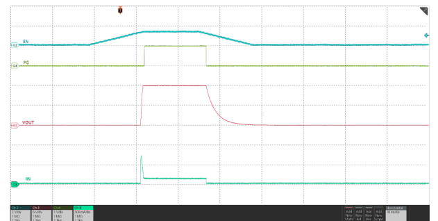
7-28. Time to Thermal Shut-Down During Inrush State
