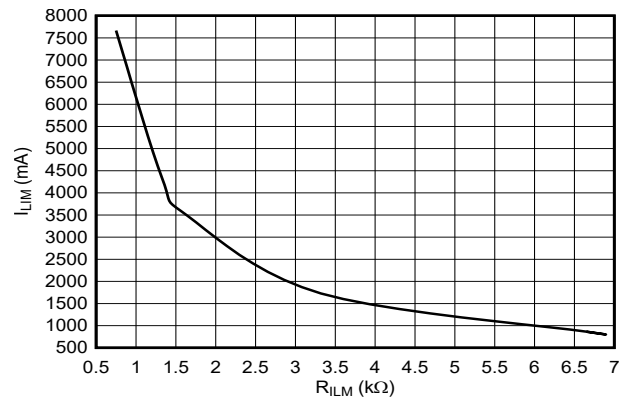
7-12. Overcurrent Threshold vs ILM Resistor
