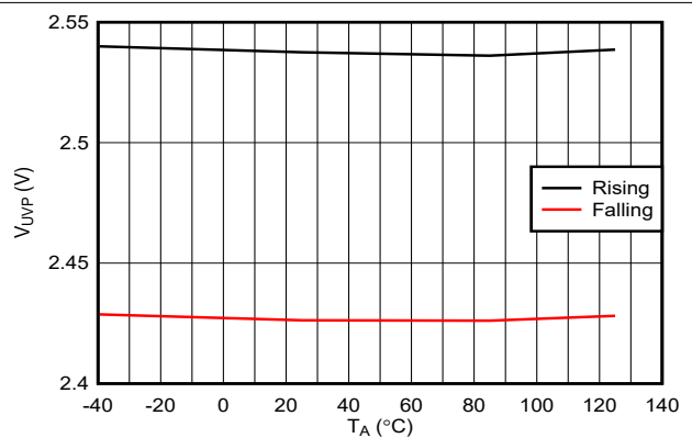
7-6. IN Undervoltage Threshold vs Temperature
