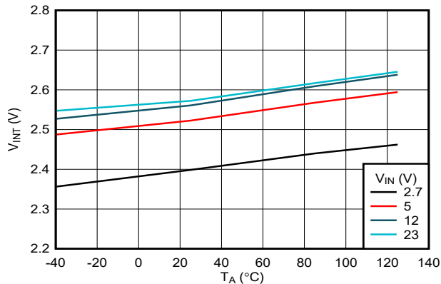
7-23. ITIMER internal Pullup Voltage vs Temperature
