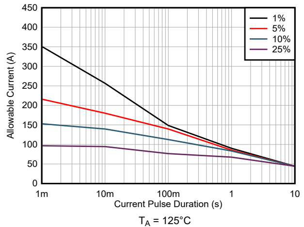
7-8. Maximum Repetitive Pulsed Current vs. Pulse Duration
