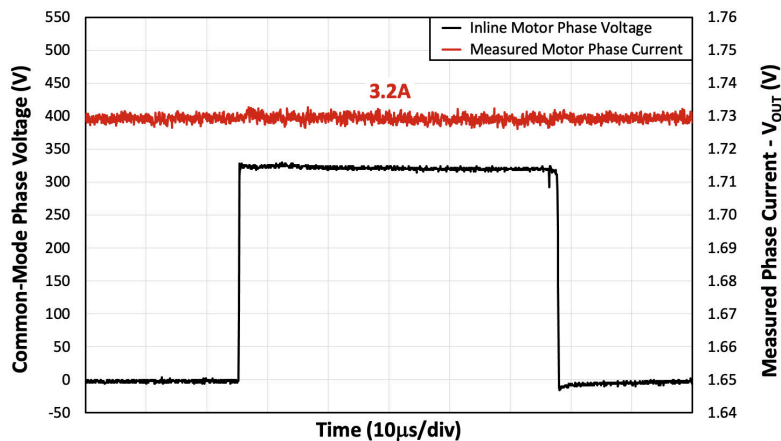
9-3. Inline Motor Current-Sense Input and Output Signals
