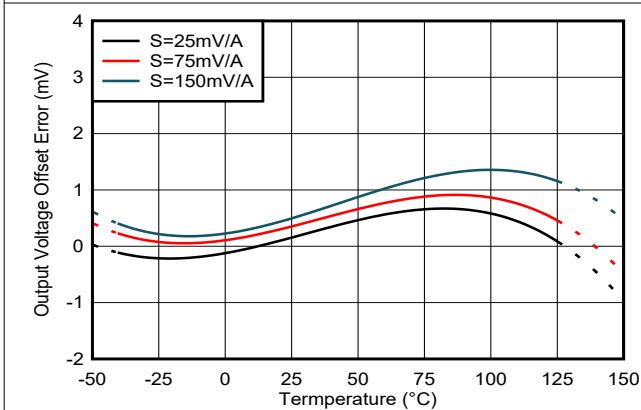
Figure 6-3. Offset Error vs Temperature: TMCS1133Bxx Device Options
