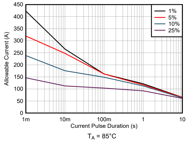
7-6. Maximum Repetitive Pulsed Current vs. Pulse Duration
