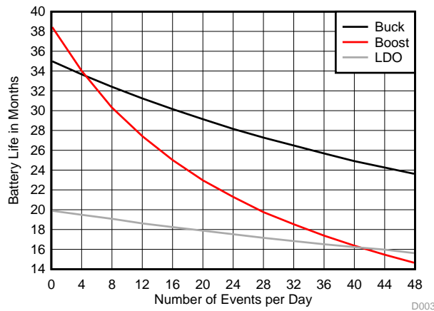
10. Number of Events Versus Battery Life With 220-ms Bluetooth® low energy Connections
