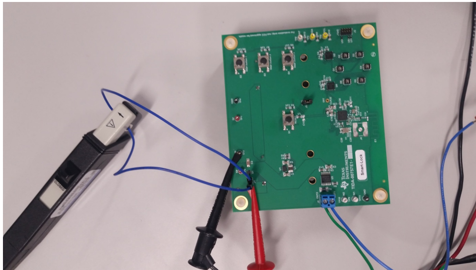
37. 5-V Power Supply Connection Configuration
