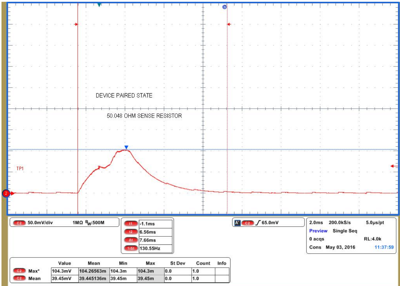
図 43. Bluetooth® low energy Device Paired Packet
