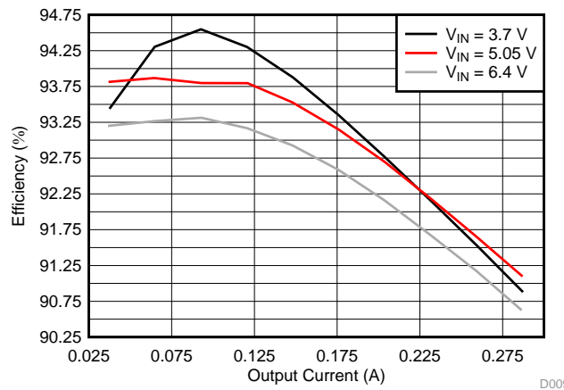
図 39. Buck Output Current Versus Efficiency (TPS62745)
