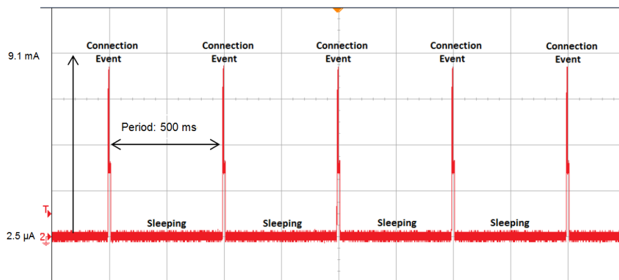
図 5. Current Consumption versus Time During Bluetooth® low energy Connections
