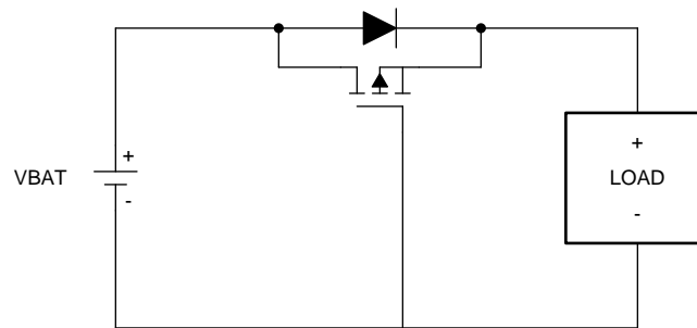
図 13. Reverse Polarity Protection PFET Configuration
