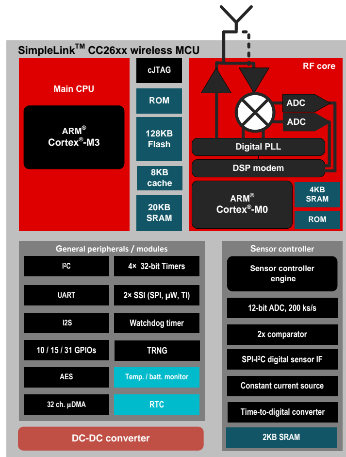
図 19. CC2640R2F Block Diagram
