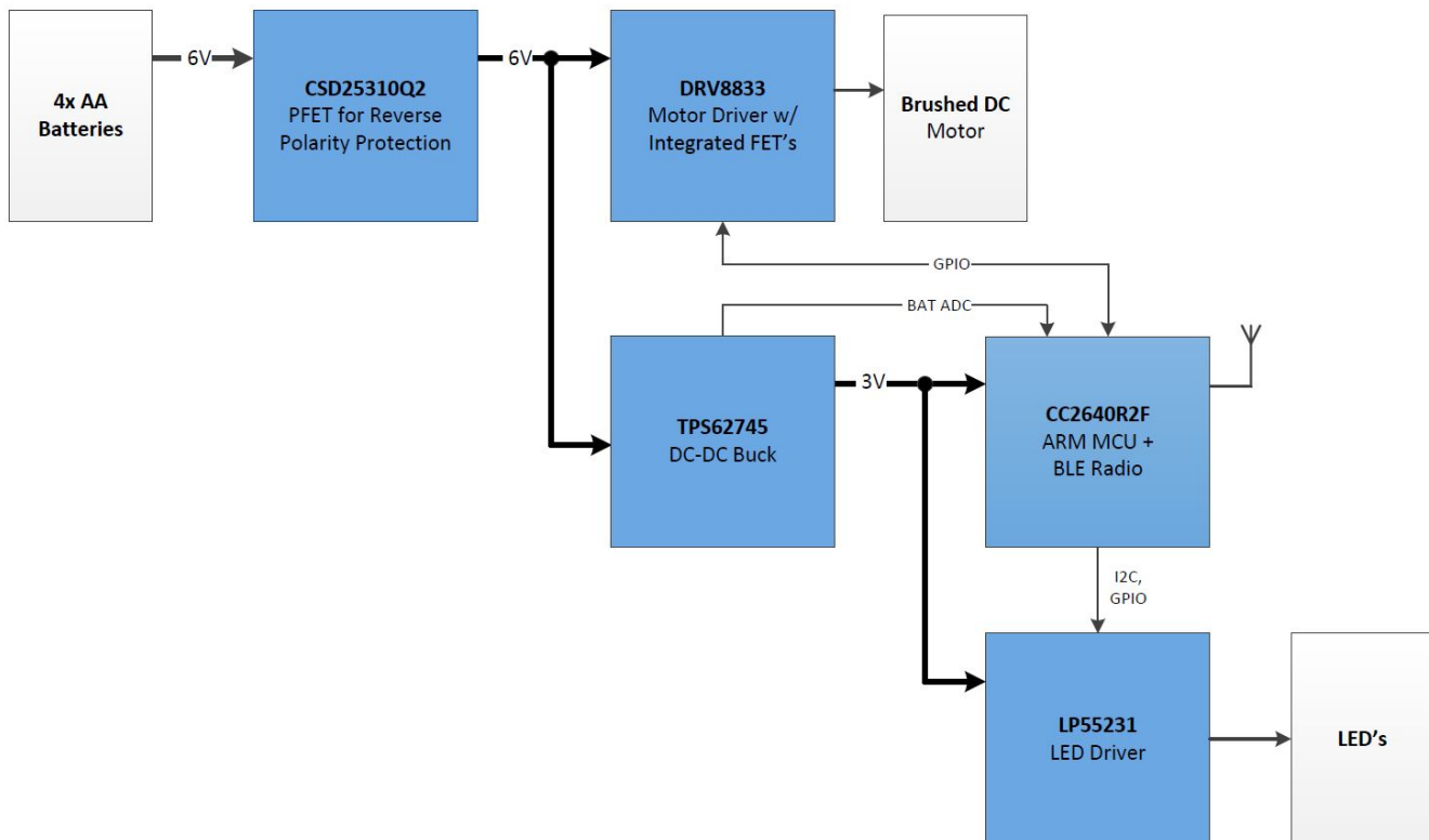
☒ 17. TIDA-00757 Block Diagram
