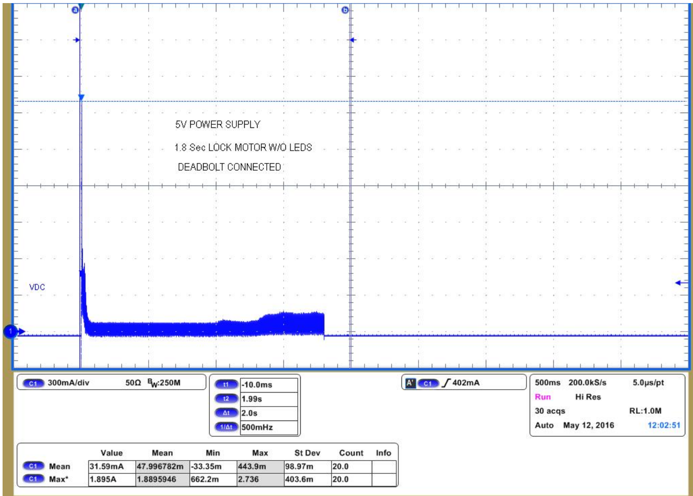
図 51. 1.8 Second Loaded Motor Lock Without LEDs Enabled
