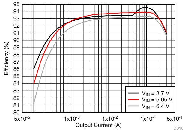
☒ 40. Buck Output Current Versus Efficiency, Wider Current Range (TPS62745)
