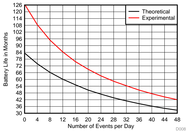
図 54. Number of Events Versus Battery Life (Theoretical and Experimental)
