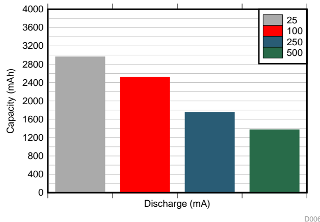
図 14. mAh Capacity of Energizer® AA Battery
