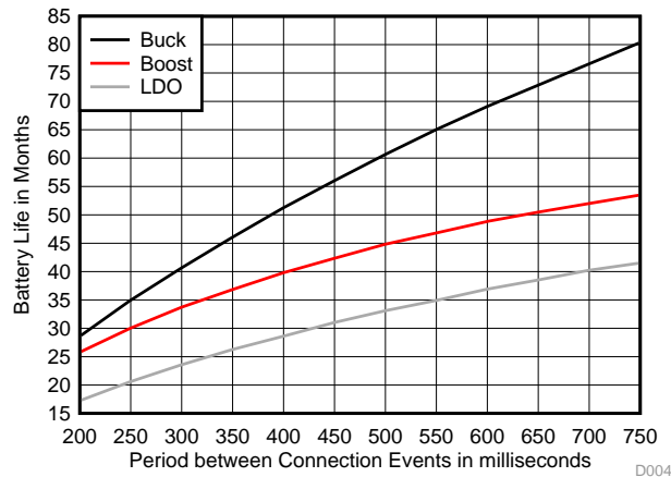
Fig 11. Bluetooth® low energy Connection Period Versus Battery Life With 12 Events
