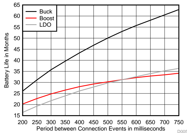
Fig 12. Bluetooth® low energy Connection Period Versus Battery Life With 24 Events
