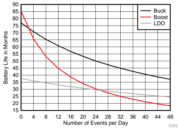
9. Number of Events Versus Battery Life With 500-ms Bluetooth® low energy Connections
