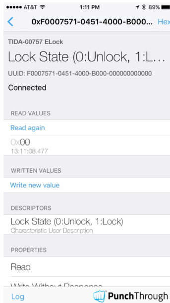
Fig 33. Lock State Values Screen
