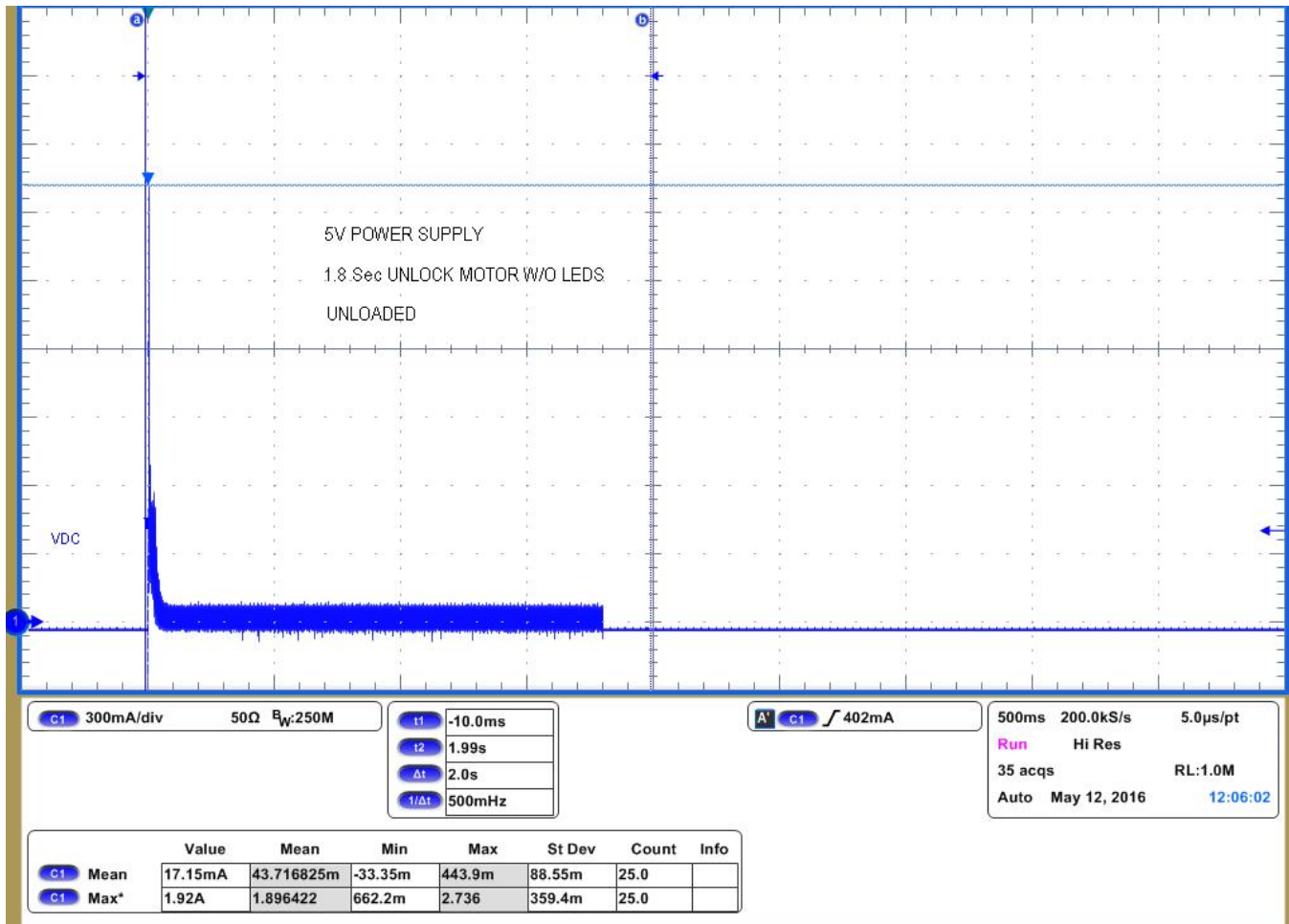
☒ 46. 1.8 Second Unloaded Motor Unlock Without LEDs Enabled
