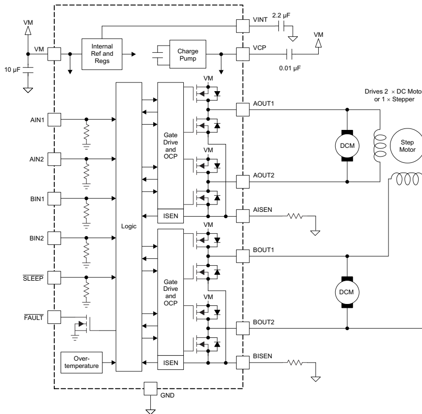
Figure 18. DRV8833 Block Diagram
