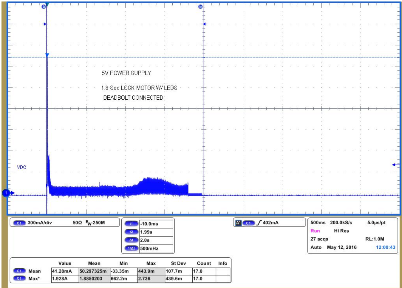
図 53. 1.8 Second Loaded Motor Lock With LEDs Enabled
