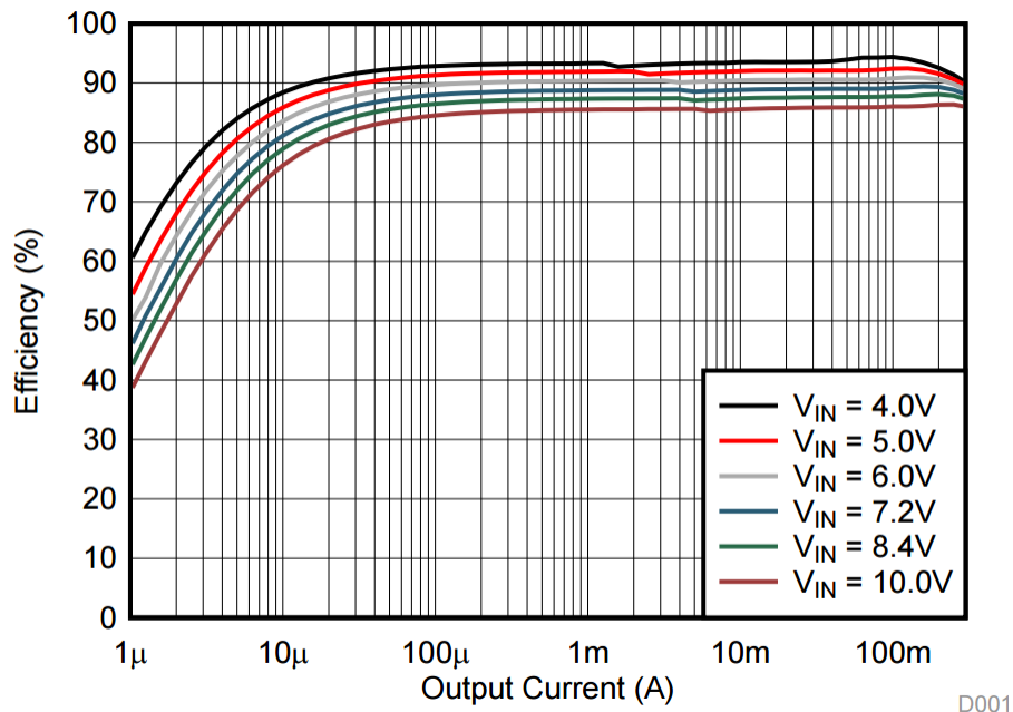
図 6. TPS62745 Efficiency Curve at V_{out} = 3.3\text{ V}
