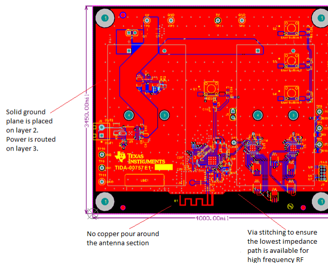
図 55. Smart Lock Reference Design Layout Guidelines
