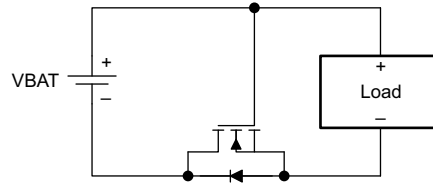
図 2. NMOS FET Ground Return Path
