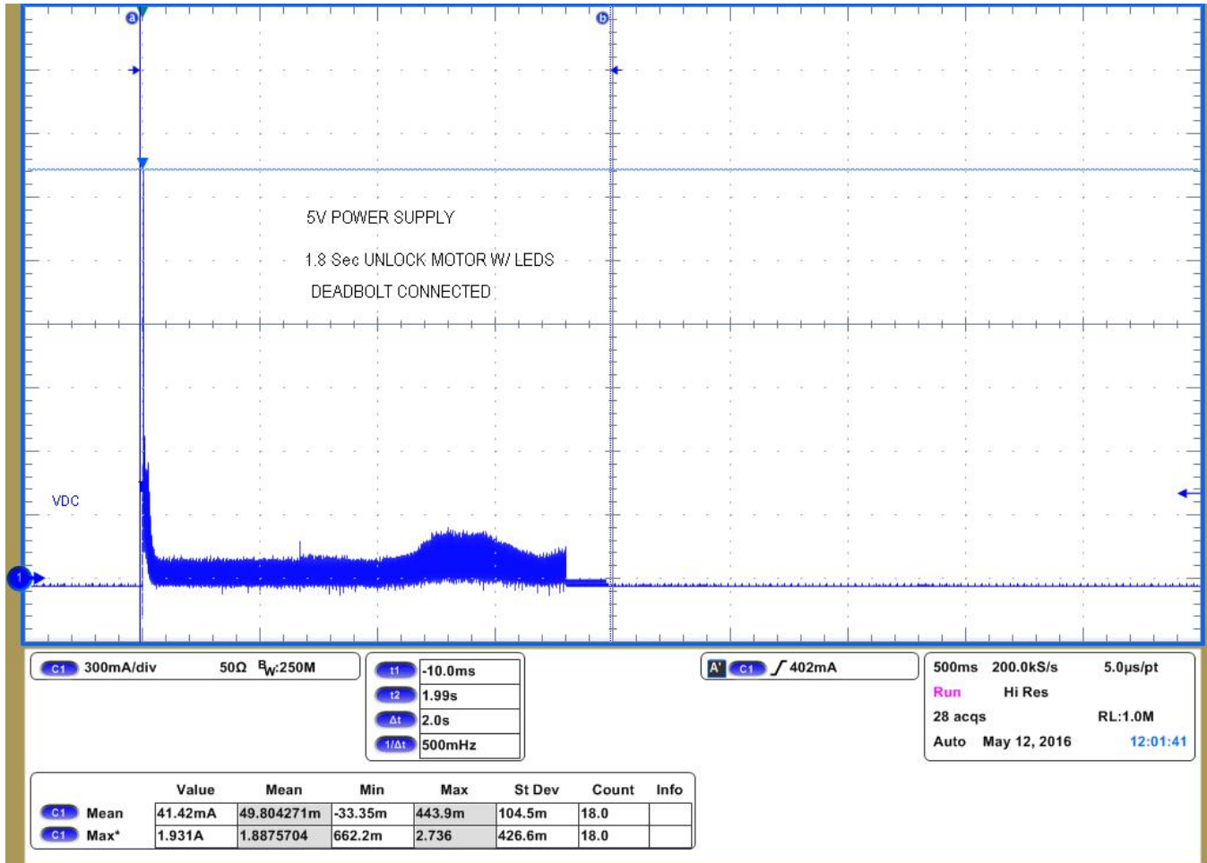
Fig 52. 1.8 Second Loaded Motor Unlock With LEDs Enabled
