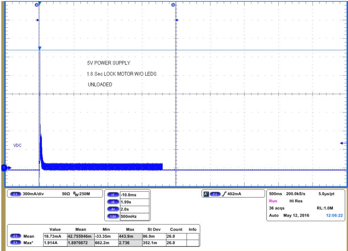
☒ 47. 1.8 Second Unloaded Motor Lock Without LEDs Enabled
