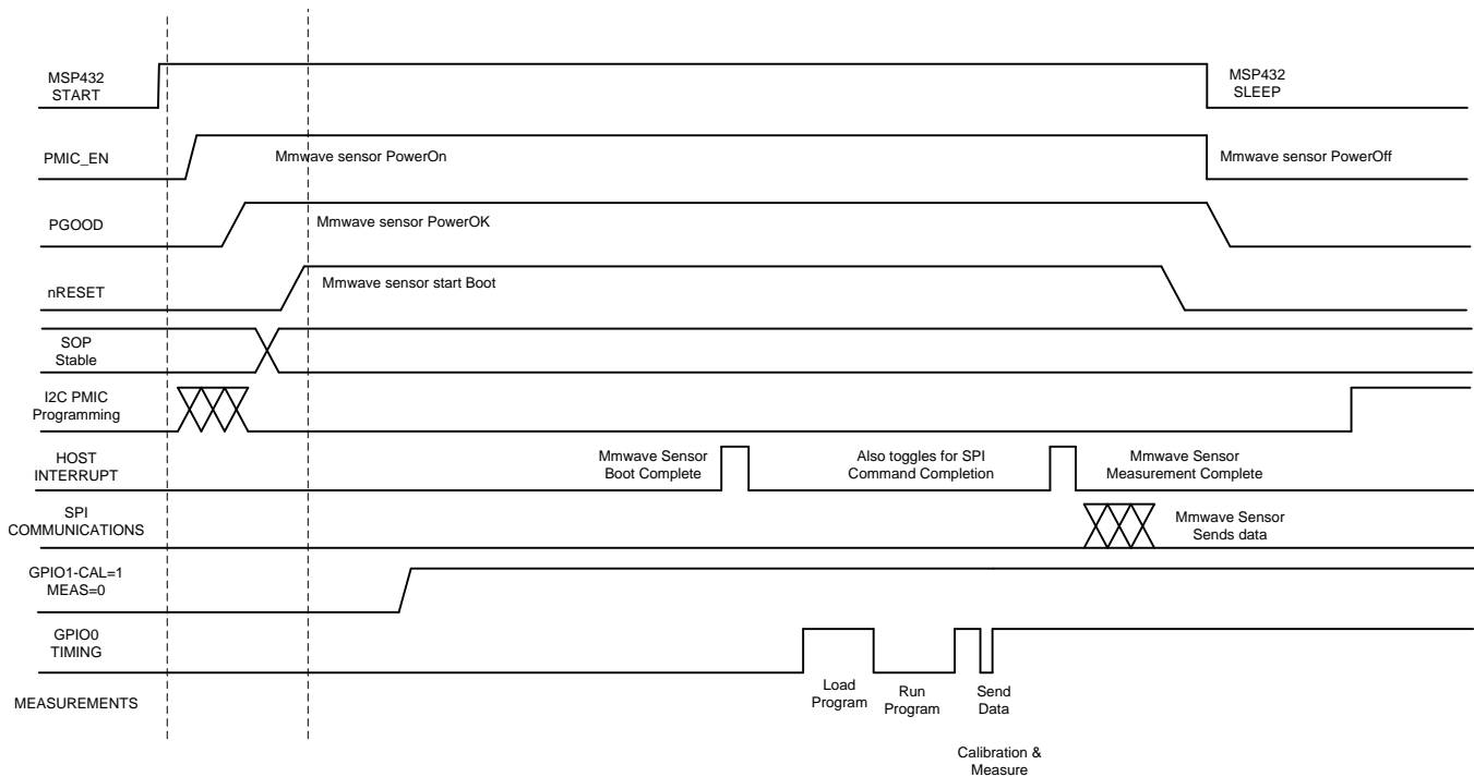
図 7. TIDEP-0091 Level Sensing Control and Communication Sequence
