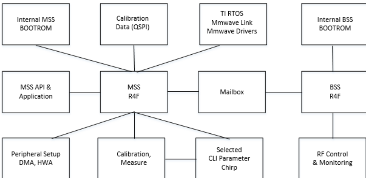
図 6. IWR1443 BOOST MSS/BSS Software Block Diagram
