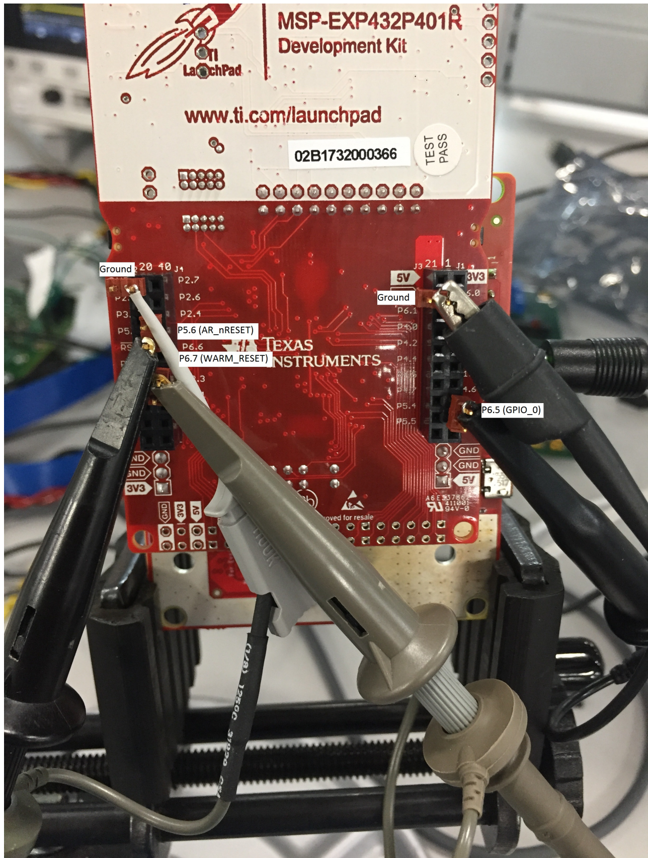
図 11. Oscilloscope Connections
