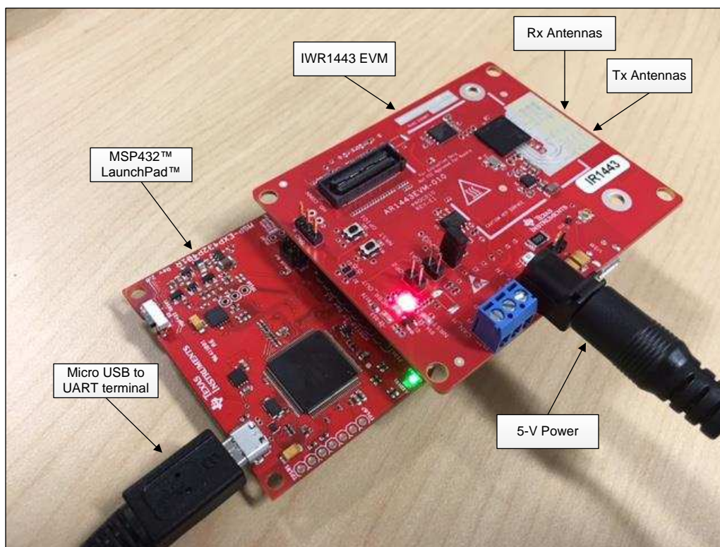
図 8. Level-Sensing Demonstration Hardware
