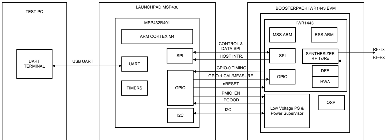
図 3. TIDEP-0091 mmWave Sensor IWR1443 BOOST and MSP432R401 EVM Diagram
