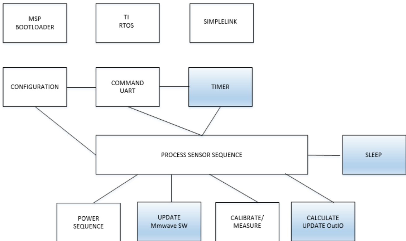
図 4. TIDEP-0091 MSP432 Host Processor Software Flow (Blue Boxes are Not Implemented)
