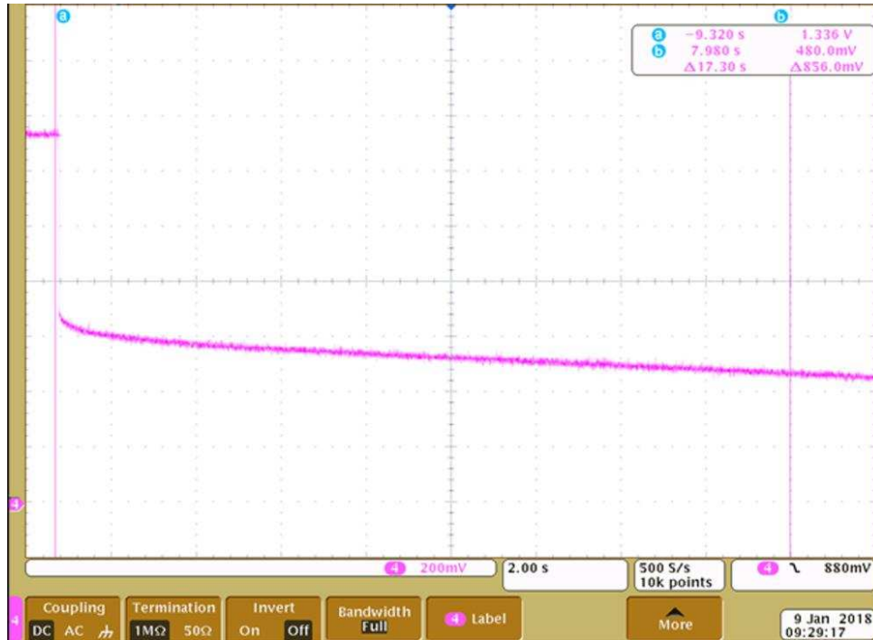
図 16. Discharge of Capacitive Load Without Fast Discharge Circuit
