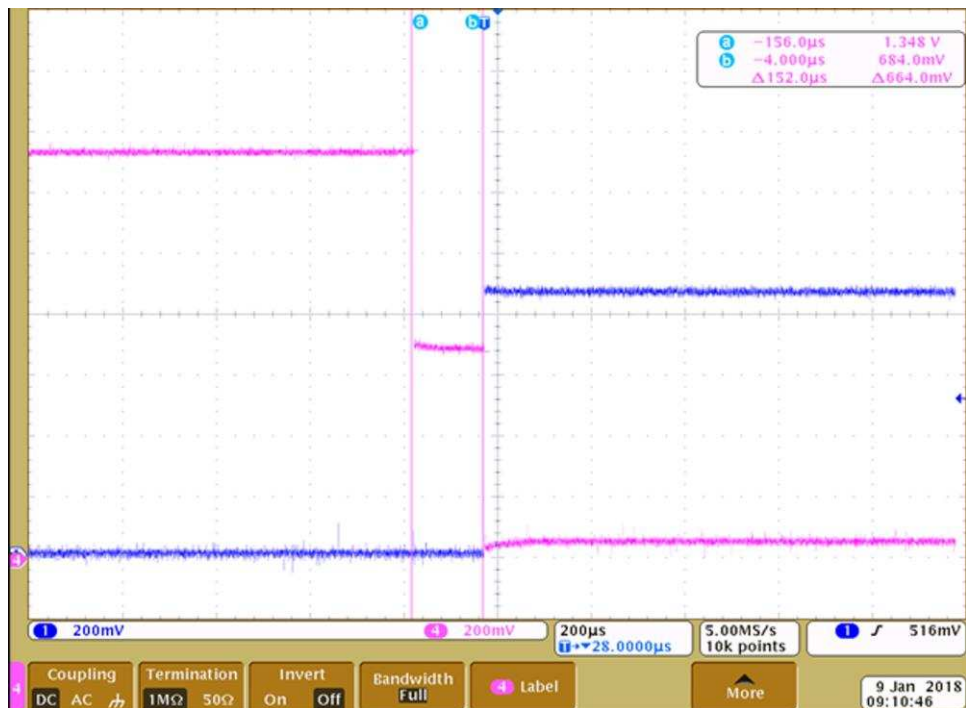
図 17. Discharge of Capacitive Load With Fast Discharge Enabled
