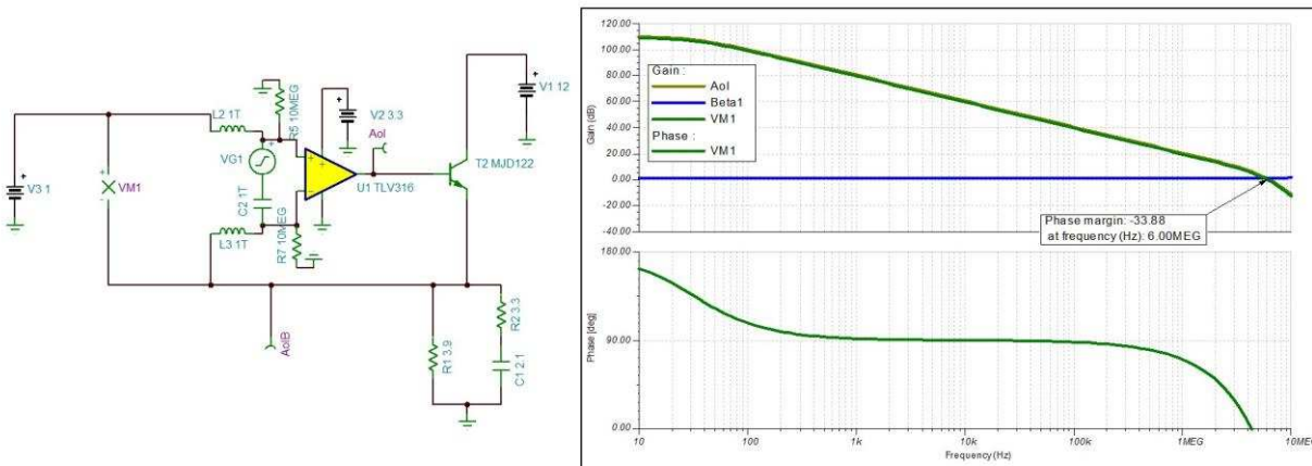
Figure 8. TINA-TI™ Stability Analysis of EC Mirror Driver Without Compensation
