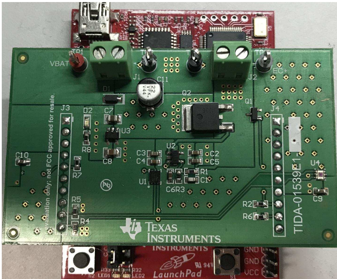
図 13. Image of TIDA-01539 Connected to MSP-EXP430G2552 LaunchPad™
