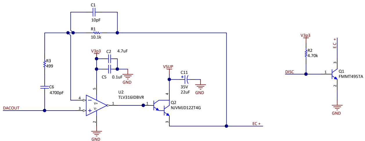
図 10. EC Mirror Driver Schematic
