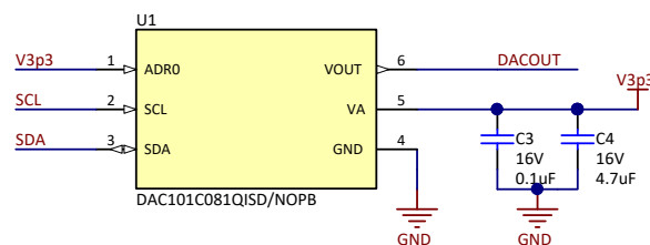
Figure 7. DAC Schematic
