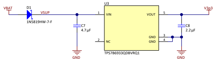
☒ 11. LDO Configuration Schematic
