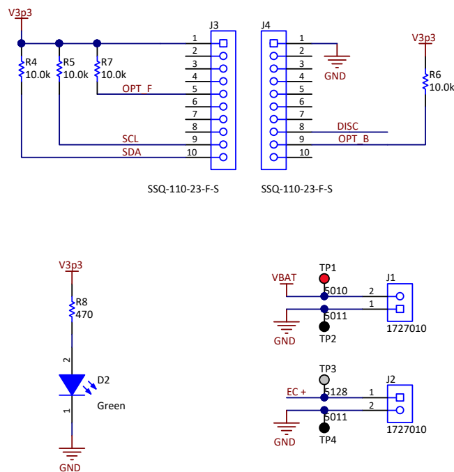
Figure 12. Schematic of Jumper Connections
