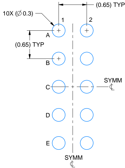
LAND PATTERN EXAMPLE EXPOSED METAL SHOWN SCALE:20X
