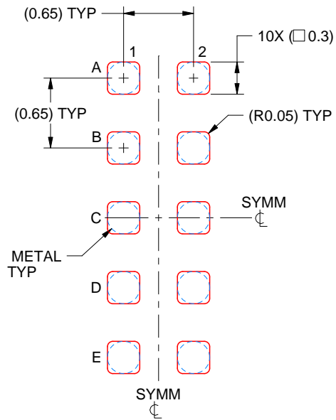
SOLDER PASTE EXAMPLE BASED ON 0.1 mm THICK STENCIL SCALE:20X
